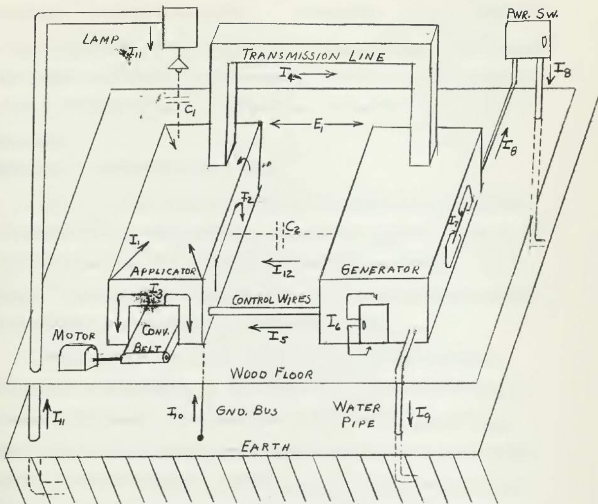
Fig. VII - 1 Stray Currents Result in Radiation from an RF Heater Installation
