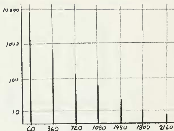
Fig. XIII - 3 Field Intensity-Frequency Signature of a 6 Mercury Arc Rectifier
