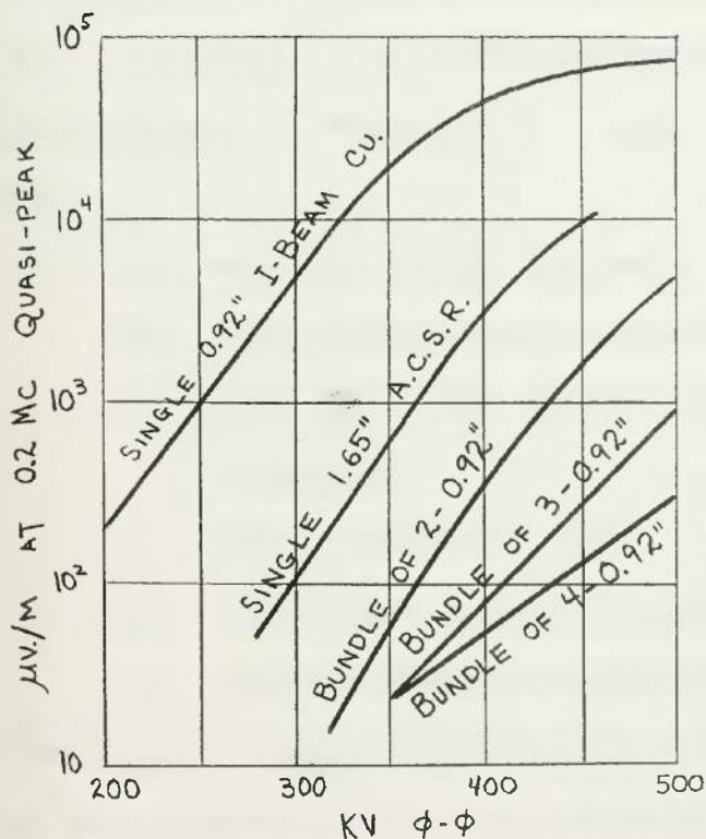
Fig. V - 6 RI Intensity Variation With Voltage In Fair Weather For Single and Bundled Conductors
