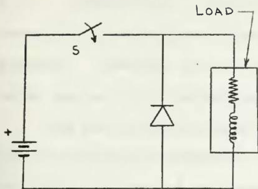
Fig. XI - 3 Shunt Diode Across Load
