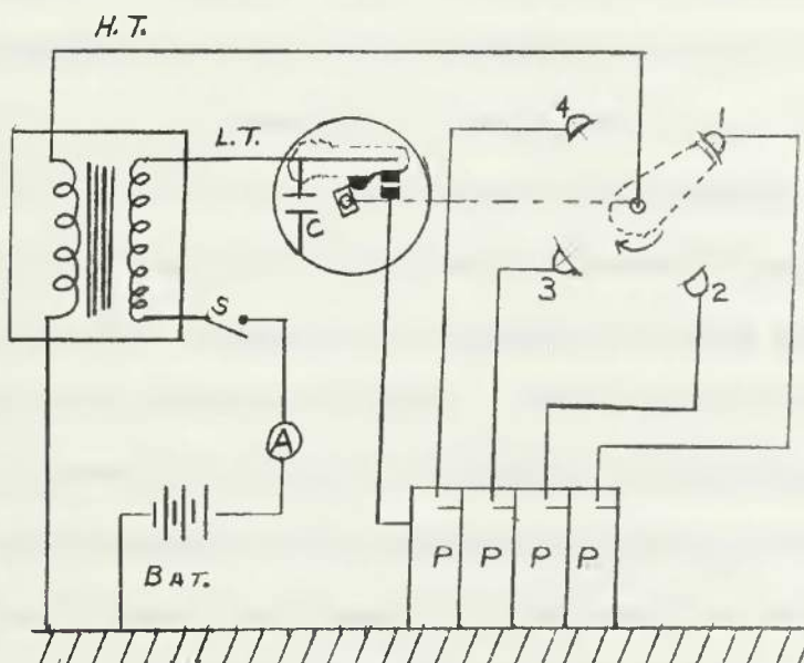
Fig. III - 1 Typical Ignition System
