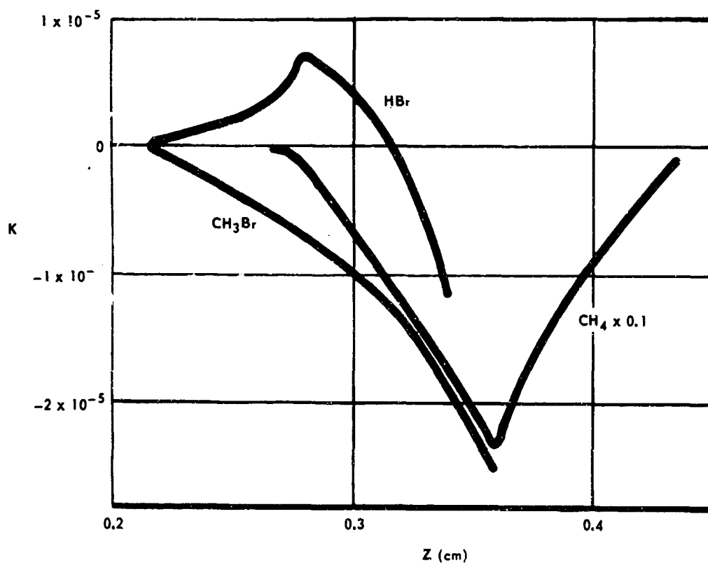
Fig. 9 NET REACTION RATES ( K_i , MOLES \text{CC}^{-1} \text{SEC}^{-1} ) FOR \text{HBr} , \text{CH}_3\text{Br} , AND \text{CH}_4 . ( \text{CH}_4 RATES WERE MULTIPLIED BY 0.1 BEFORE PLOTTING.)
