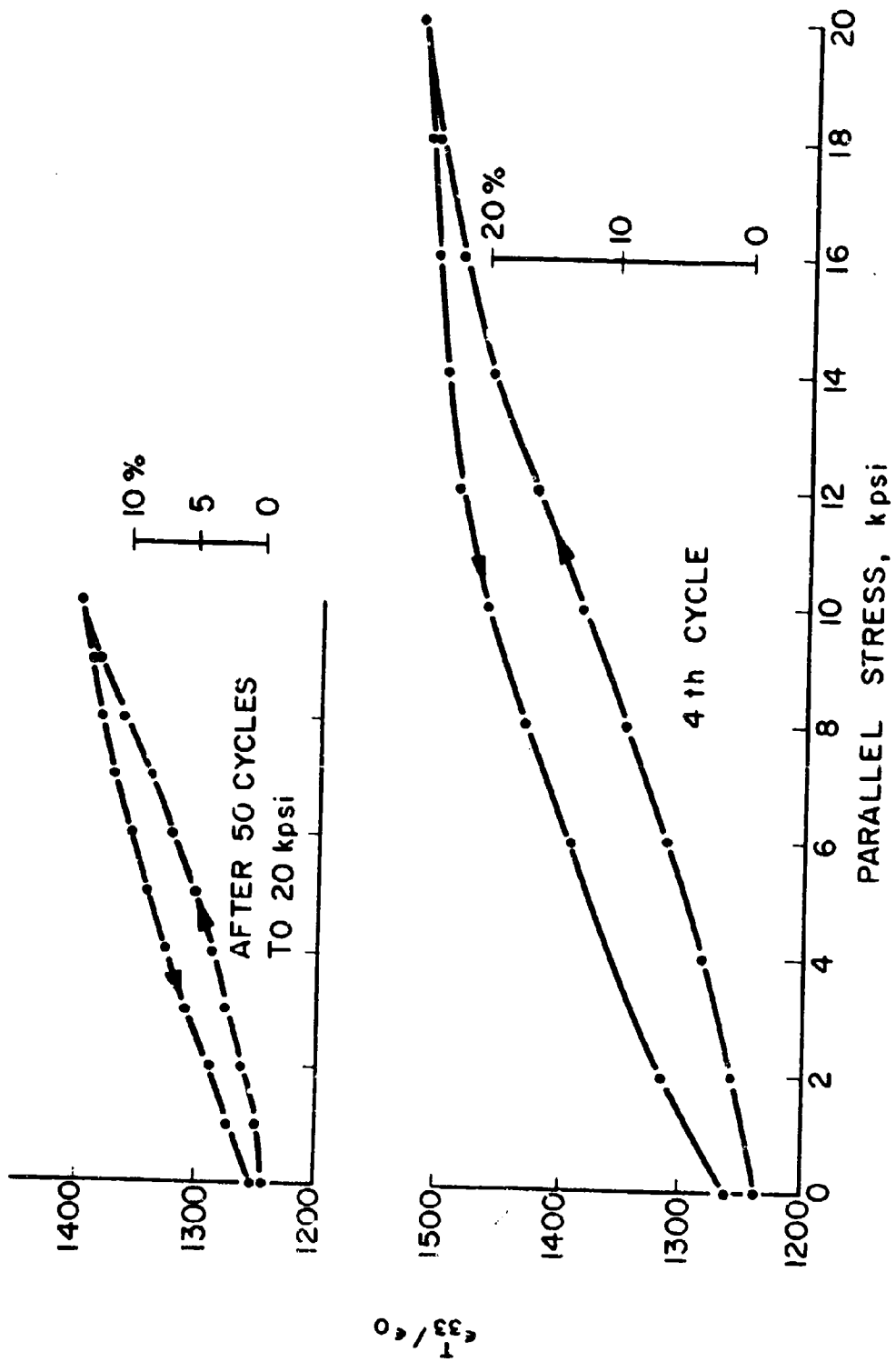
Fig. 16 \epsilon_{33} / \epsilon_0 vs. PARALLEL STRESS STABILIZED PZT-8
