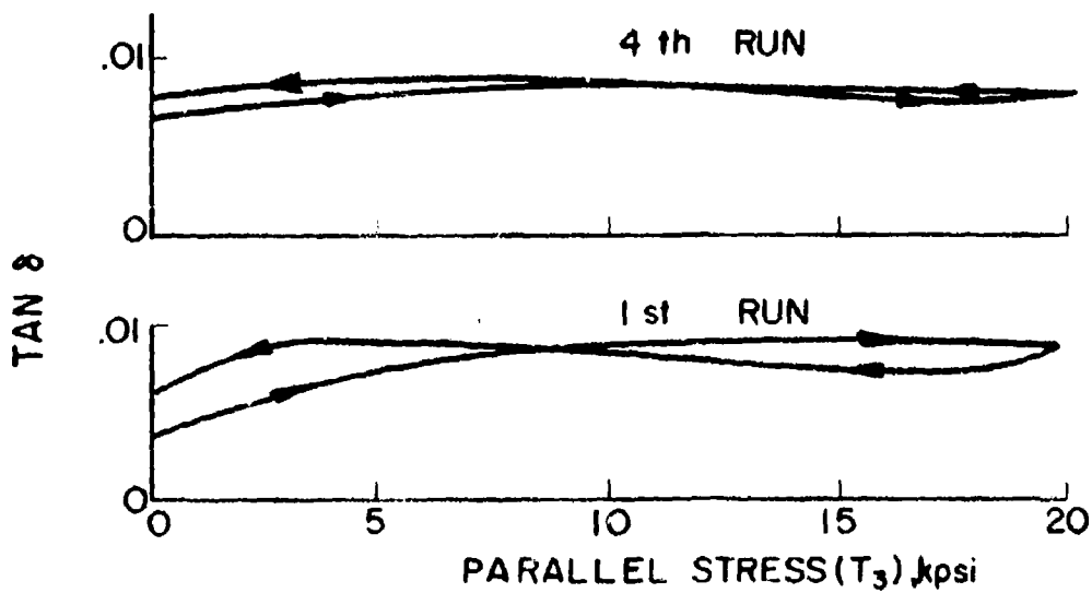
FIG. 12 12e_{33}^T/e_0 vs. PARALLEL STRESS, PZT-4 (NOT STABILIZED)
