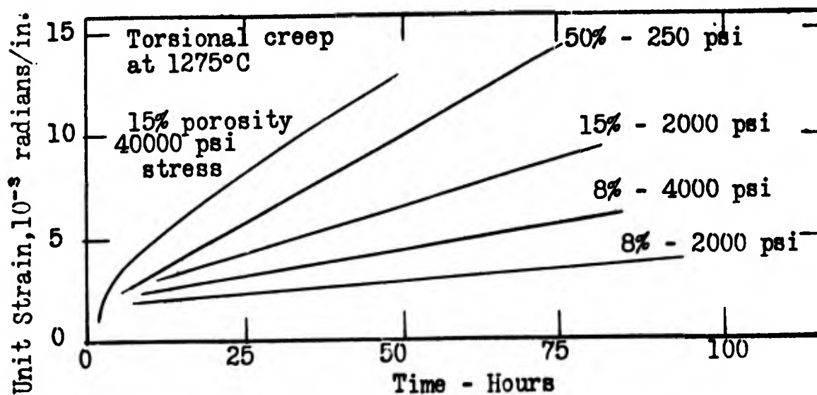
Figure 12. Creep, Creep Recovery, Torsional Creep and Influence of Porosity on Creep
