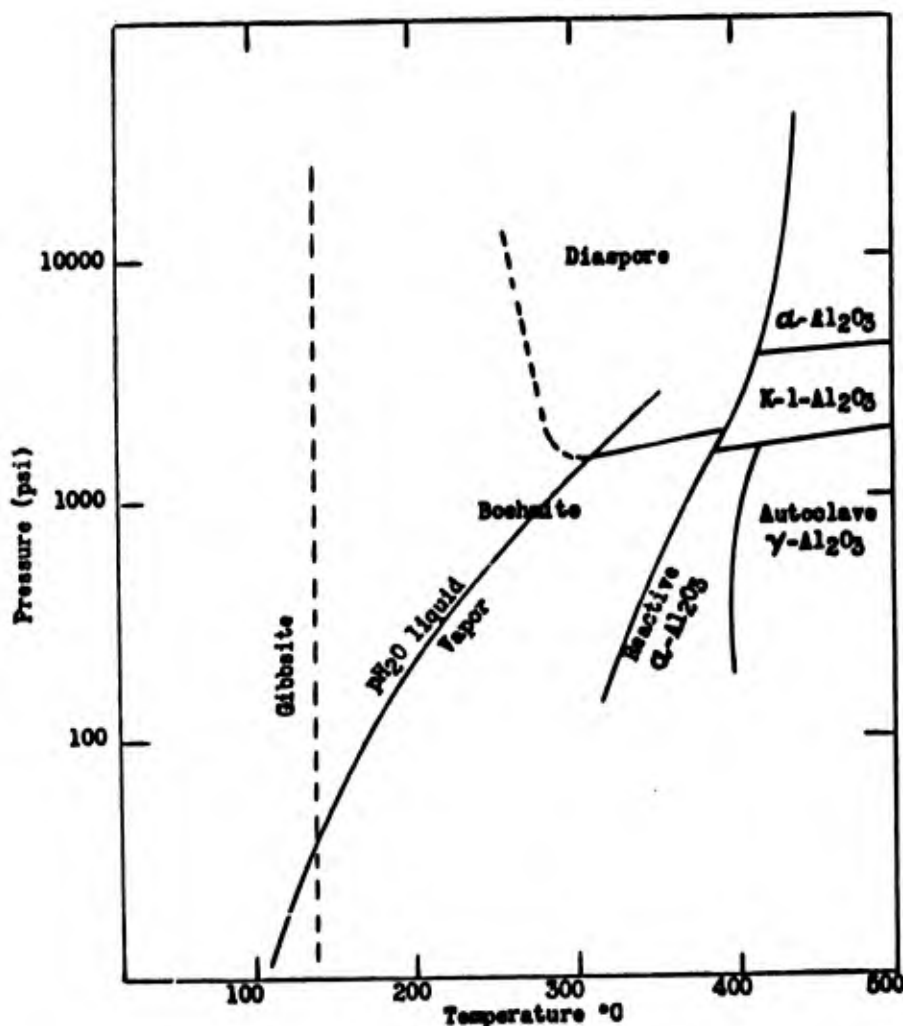
Figure 6. System \text{Al}_2\text{O}_3\text{-H}_2\text{O} (After Ervin and Osborn, and Krishner and Torkar)
