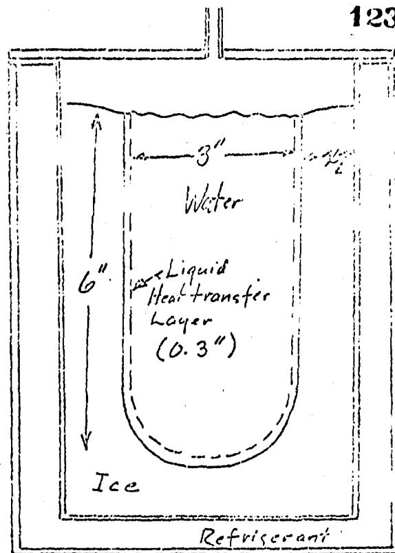
Figure 1 Computation Model
