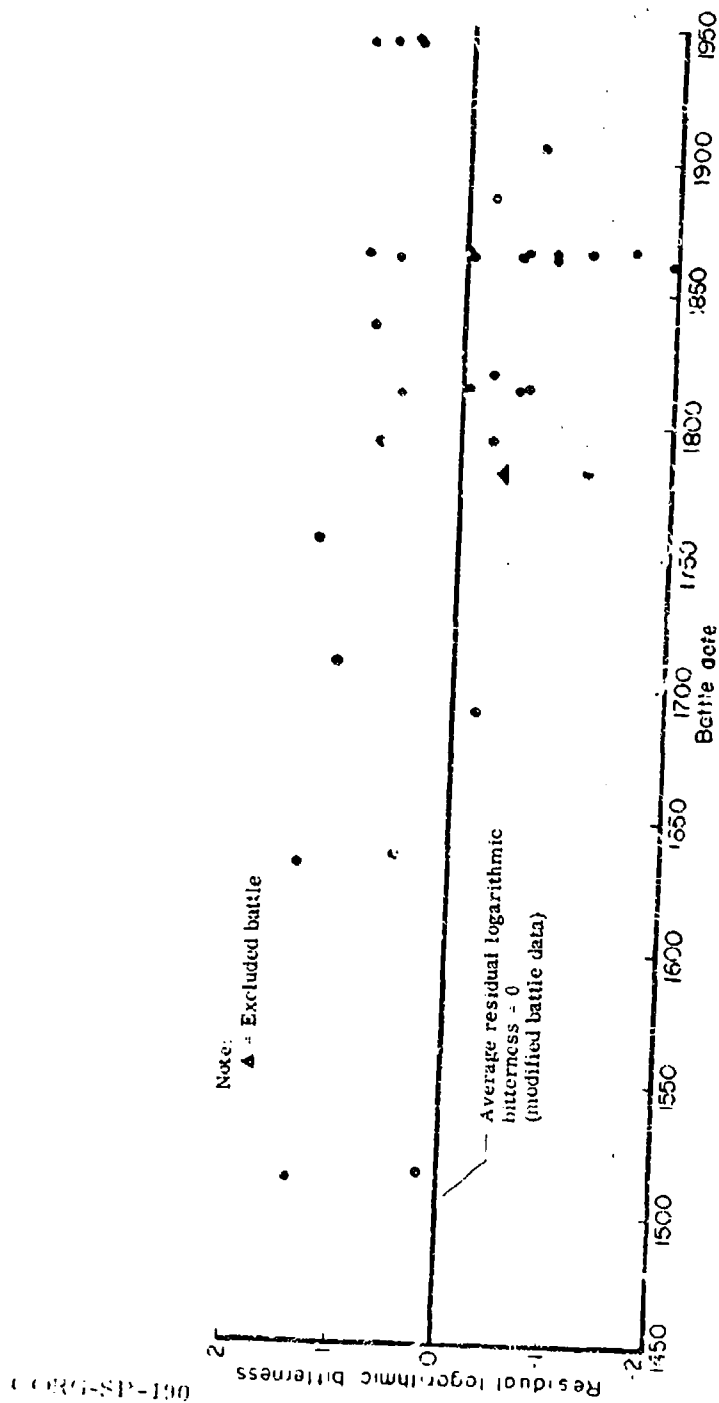
Figure 24. Linear scatter diagram of residual logarithmic bitterness against battle date for phase-2 data.
