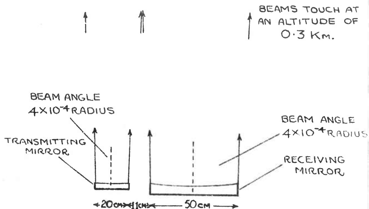
FIG. 14 THE PHYSICAL ARRANGEMENT OF THE TRANSMITTED AND RECEIVED BEAMS.
