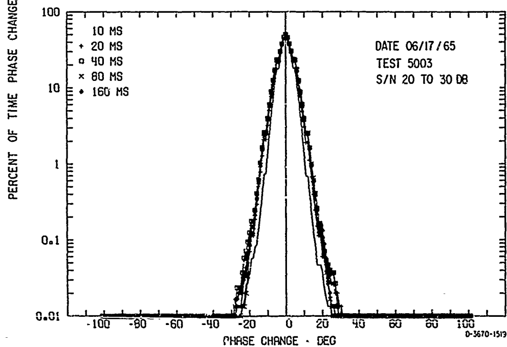
FIG. 26 PHASE DISTRIBUTION— STABLE PHASE AND AMPLITUDE TEST (5003)
