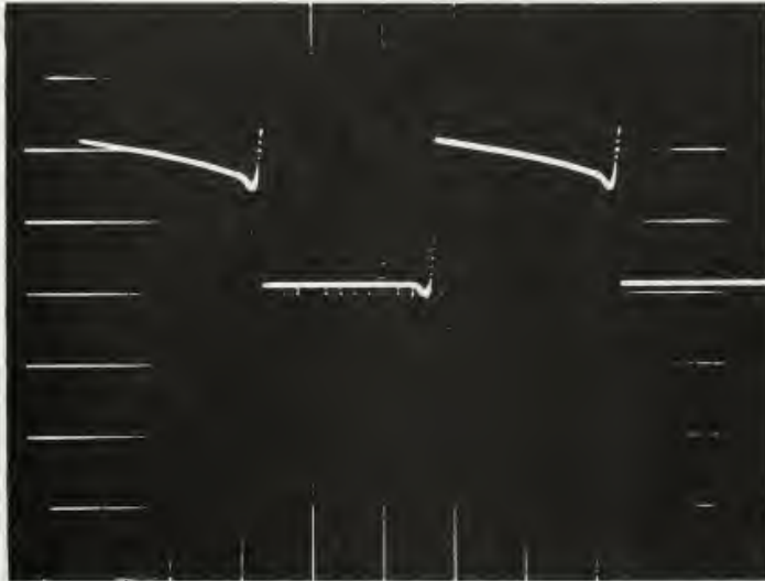
Fig. II-9 time 1 cm = 200 \mu sec Amplifier Current vs Time
