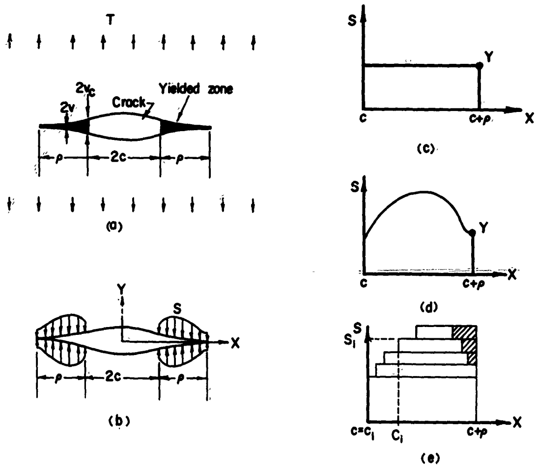
Fig. 9. The DM Model: (a) Crack with Wedge-shaped Plastic Zones, (b) Crack with "Equivalent" Internal Tension, (c) Uniform Tension Distribution of Dugdale, (d) Varying Tension Distribution, and (e) Stepwise Approximation of the Varying Tension Distribution.
