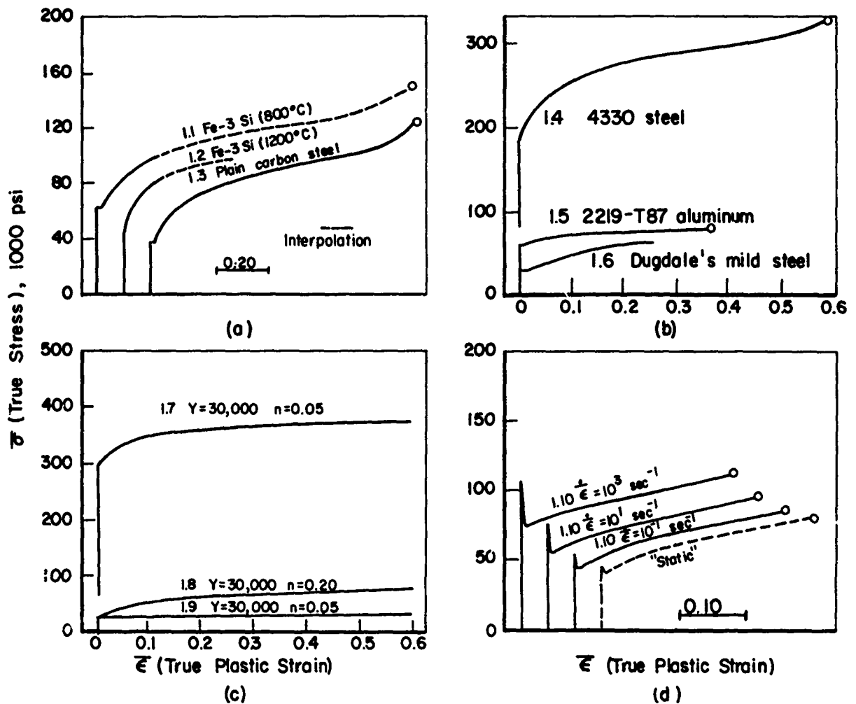
Fig. 1. True-Stresses/True-Strain Curves
