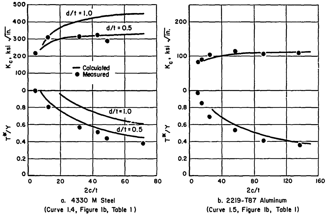
Fig. 13. Comparison of Calculated Fracture Stress and K_c Levels with Values Measured experimentally.
