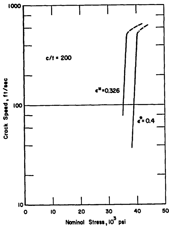
Fig. 15. Influence of Nominal Stress on Steady-State Crack Speed in Mild Steel (Curves 1.10, Fig. 1d and Table 1).
