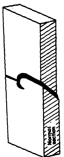
a. Local yielding in plain carbon steel
