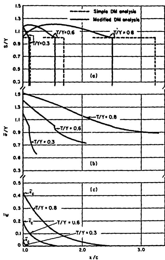
Fig. 10. Stress and Strain Gradients Calculated for a Crack in 4330 M Steel (Curve 1.4, Fig. 1c, Table 1, c = 3.75 in., t = 0.140 in.): Internal tension Stress True strain (plastic)
