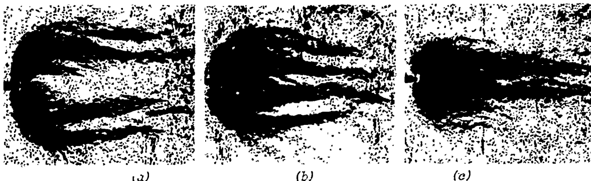
Fig. 3. Plastic Zone Revealed by Etching Sections Parallel to the Test Coupon Surface (Morris reagent, magnification 4.39X.)
