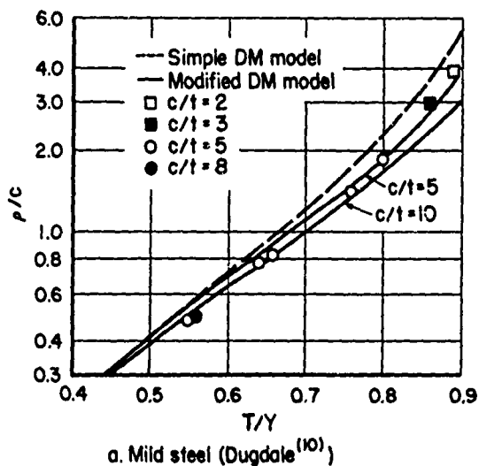
Fig. 11. Comparison of the Measured and Calculated Plastic-Zone Sizes
