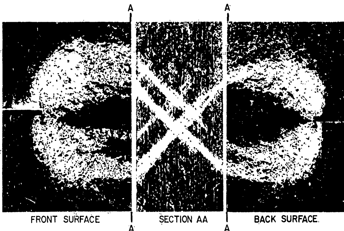
Fig. 4. Appearance of Plastic Zone on the Front Surface, Back Surface, and a Normal Section
