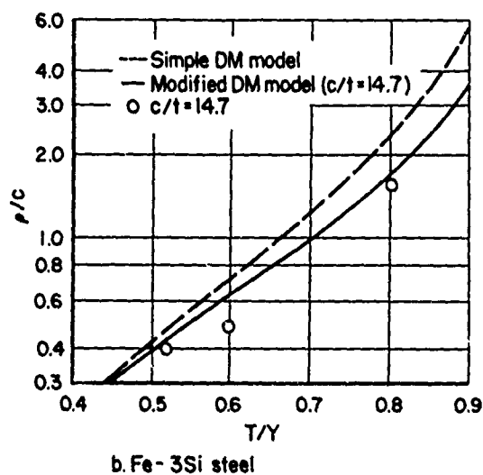
Fig. 11. Comparison of the Measured and Calculated Plastic-Zone Sizes
