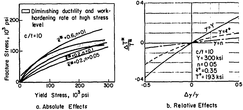
Fig. 14. Calculated Curves Showing the Influence of Yield-Strength Level, Work-Hardening Rate, and Ductility on the Fracture Stress of Hypothetical Steels (Equation 1, Table 1).
