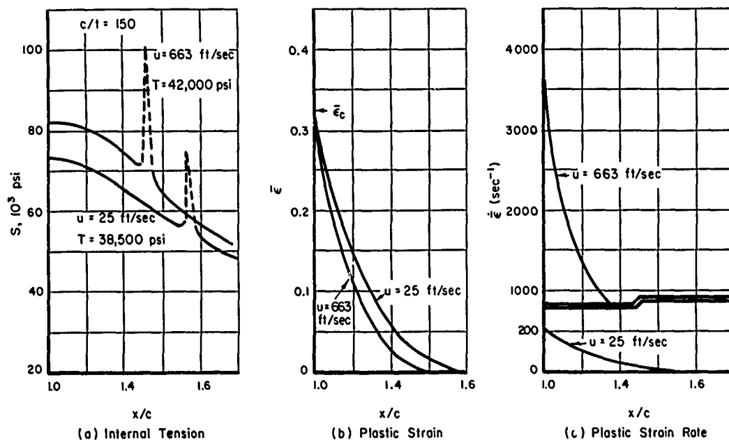
Fig. 16. Tension, Strain, and Strain Rate in Advance of a Propagating Crack in Mild Steel (Curves 1.10, Fig. 1d, Table 1).
