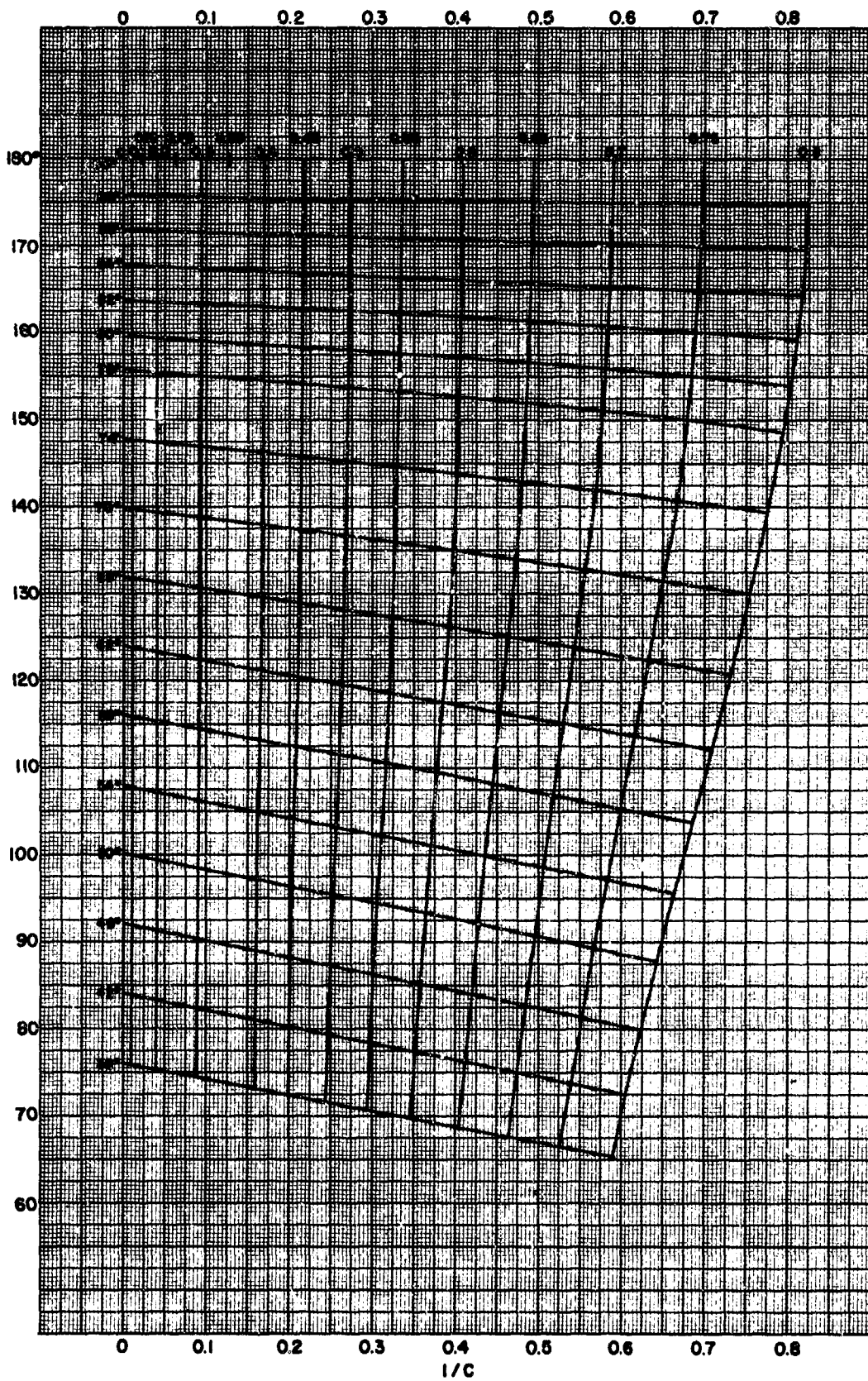
Chart XVI. T , 0 to 0.8, r , 38^\circ to 90^\circ
