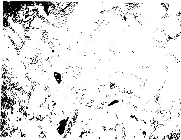
Figure 3. Ti-B (1 At% B), Quenched with 70°C per Second from 1550°C. X1250 \beta -Ti (Transformed), and Traces of Excess Monoboride.
