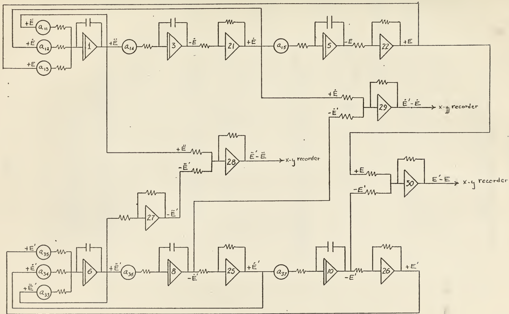
Fig. C-1 Analog Computer Set-up Used to Obtain Phase Trajectory of Fig. 42
