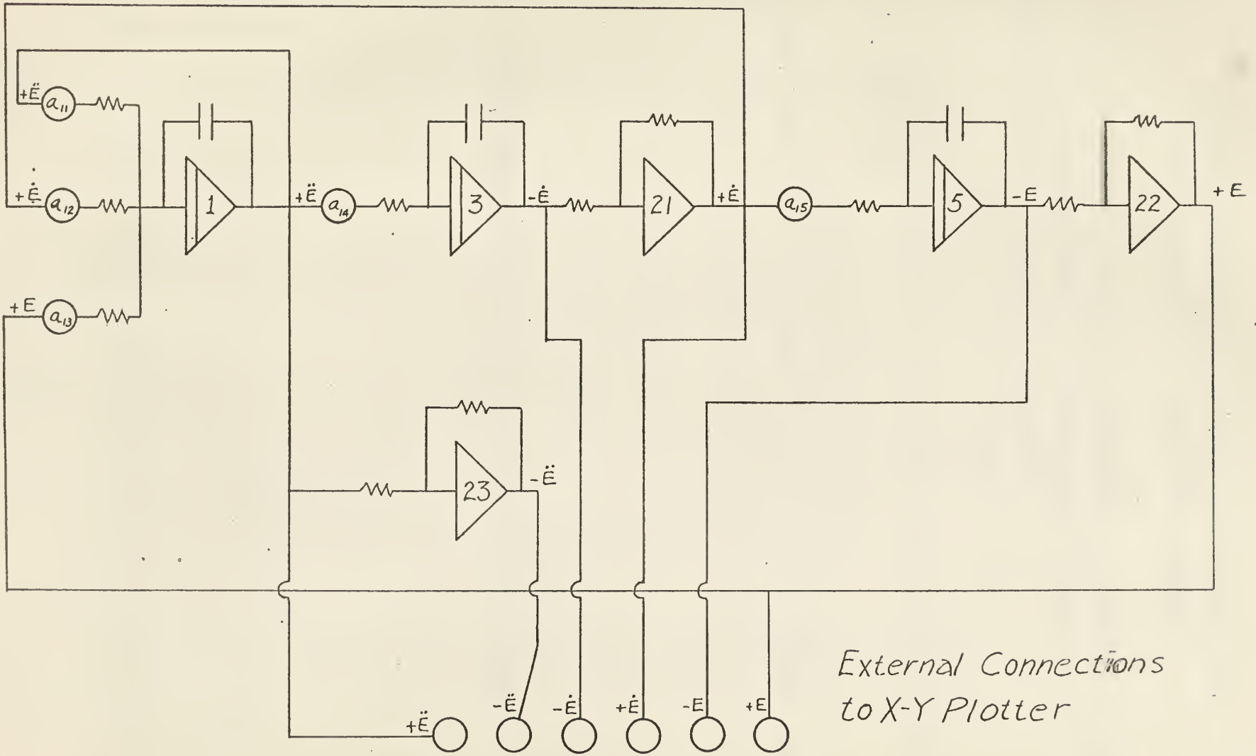
Fig. B-1 Analog Computer Set-up for Third Order Phase Trajectories
