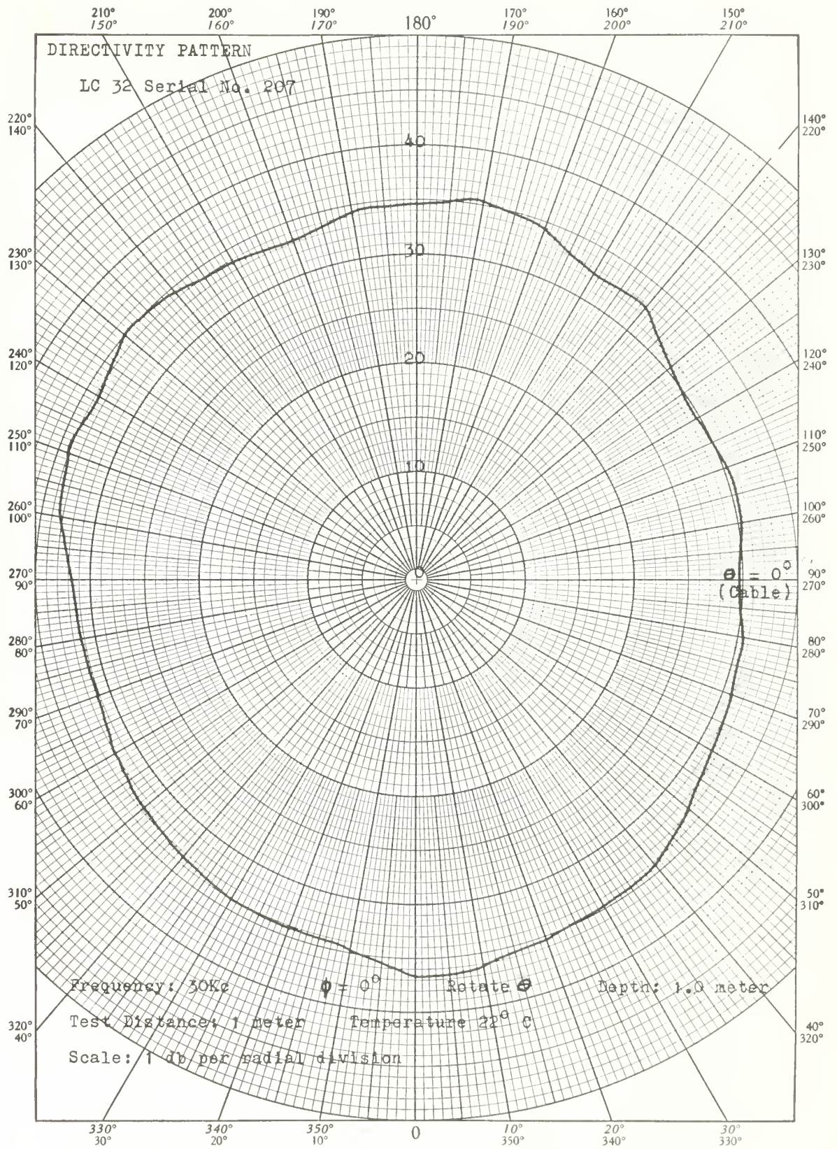
Figure II-10 Vertical Directivity Pattern, Ser. 207, 30Kc
