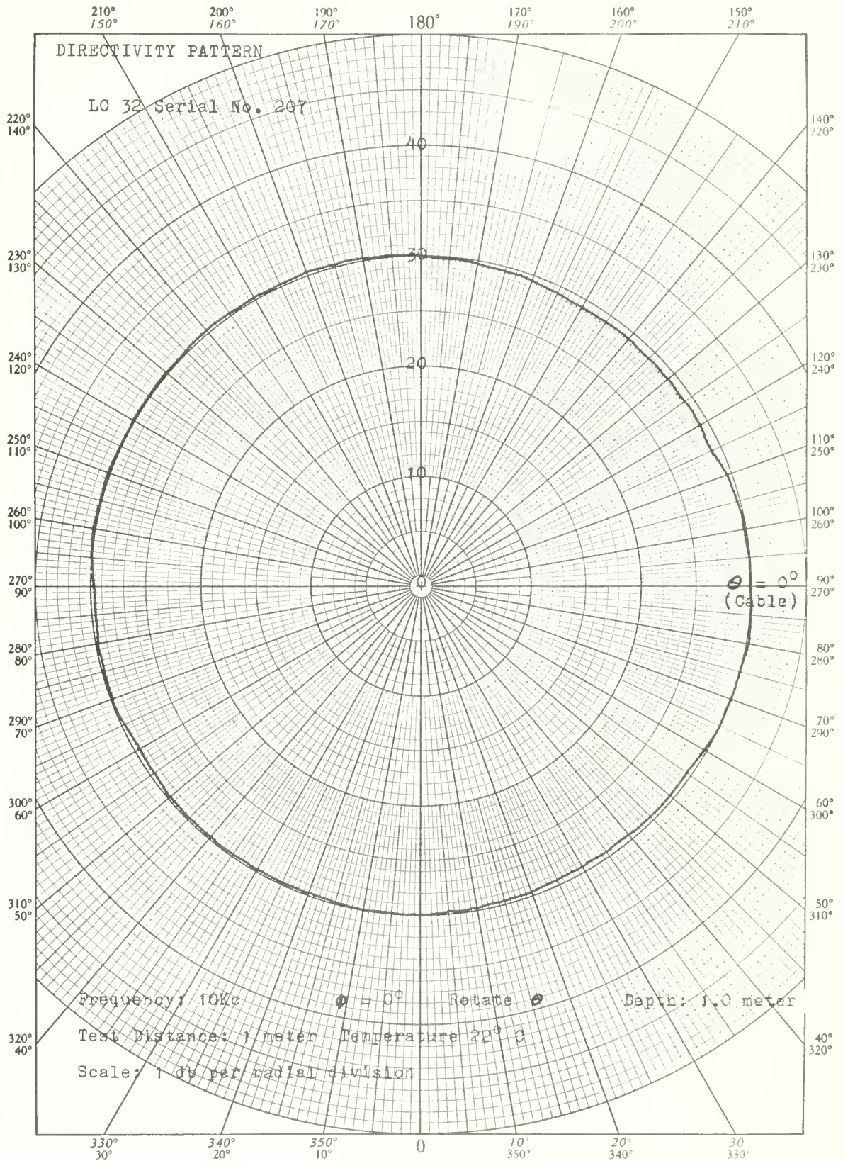
Figure II-8 Vertical Directivity Pattern, Ser. 207, 10Kc
