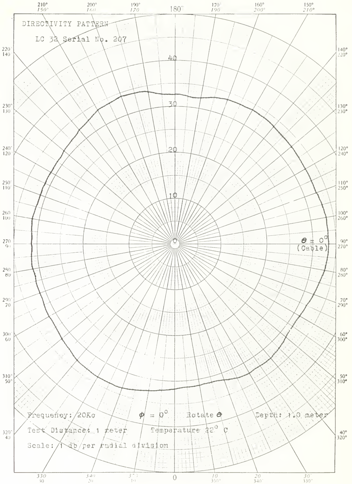
Figure II-9 Vertical Directivity Pattern, Ser. 207, 20Kc
