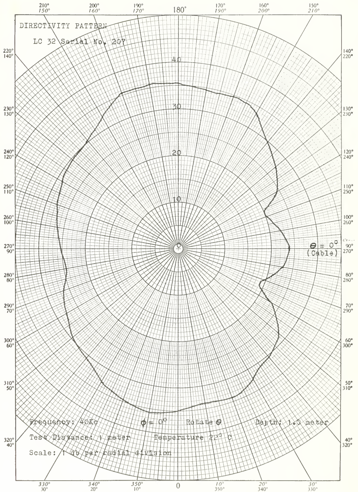
Figure II-11 Vertical Directivity Pattern, Ser. 207, 40Kc
