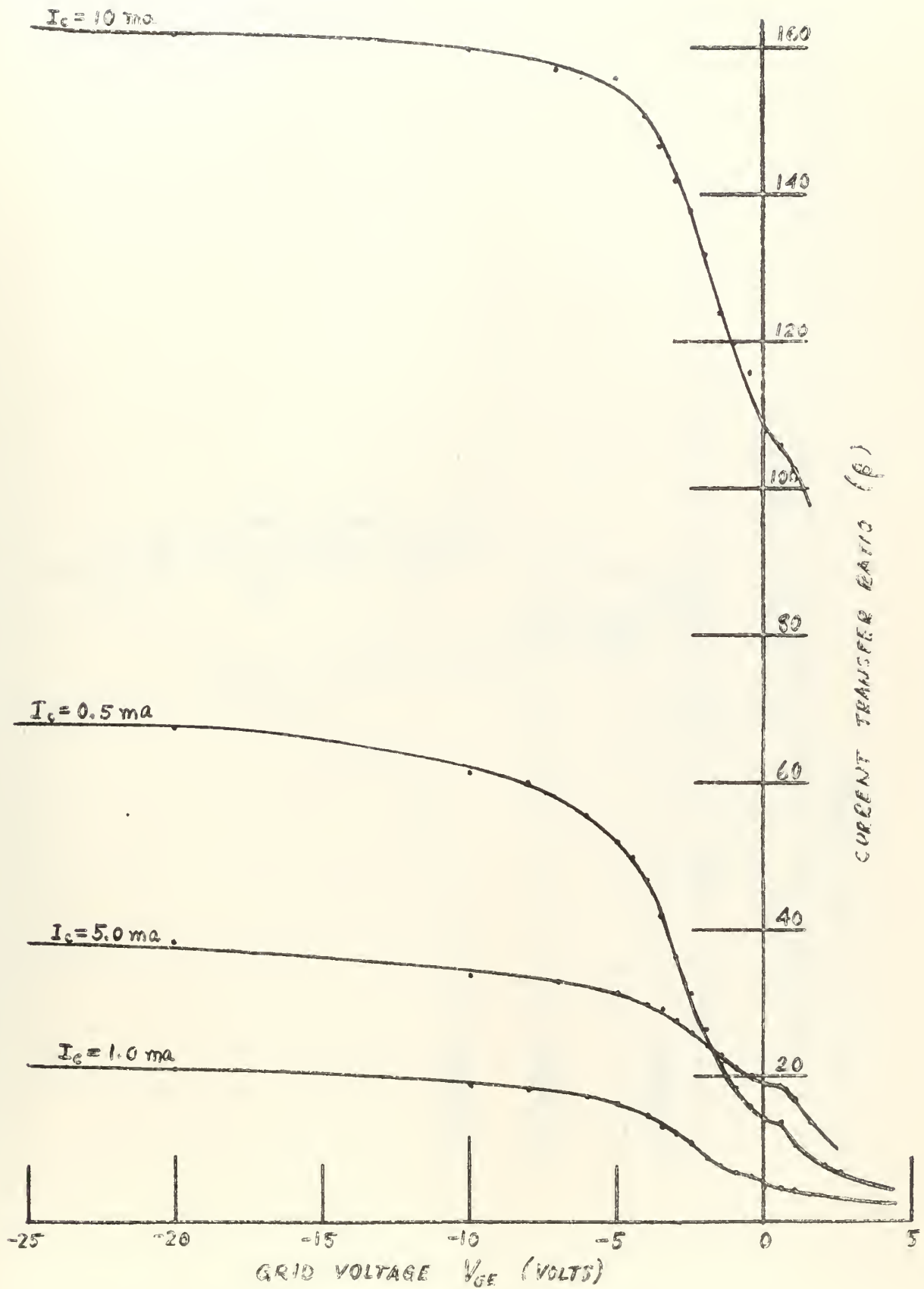
Fig. 8 Common emitter current transfer ratio as a function of V_{GE}
