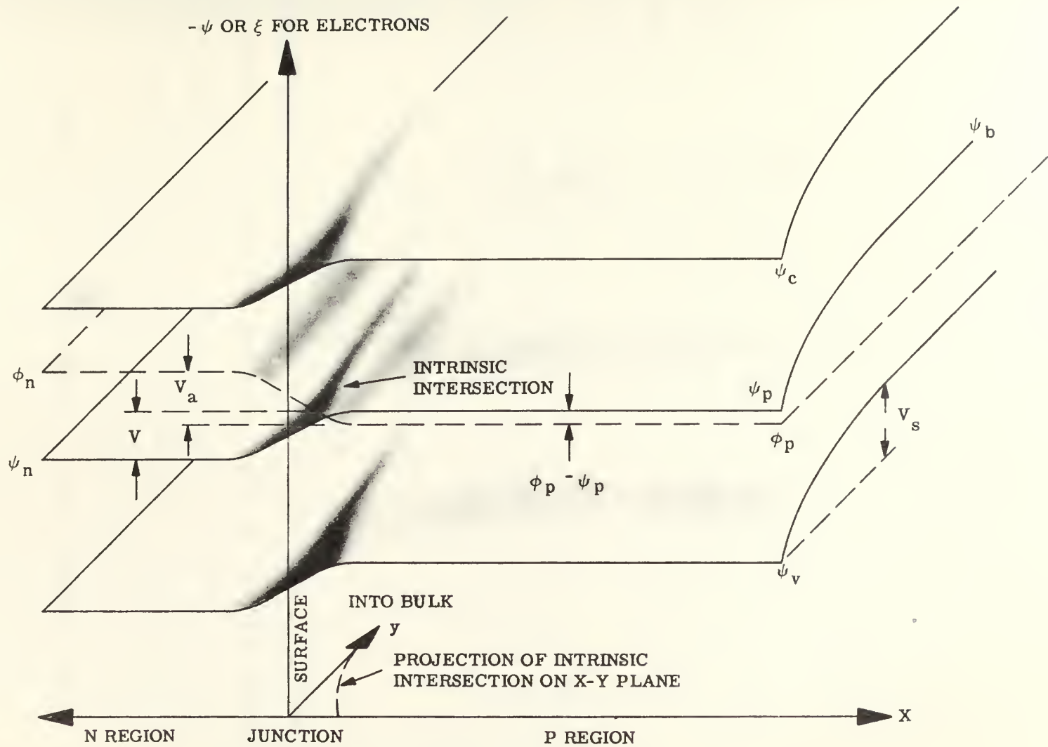
Fig. 5c Junction with forward bias V_a and positive potential V_s applied to the surface.
