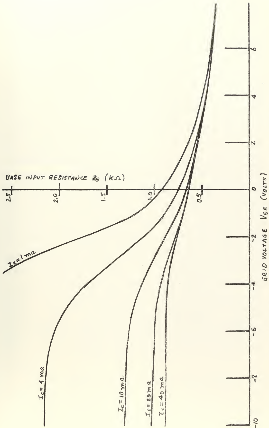
FIG. 1A BASE INPUT RESISTANCE AS A FUNCTION OF GRID VOLTAGE
