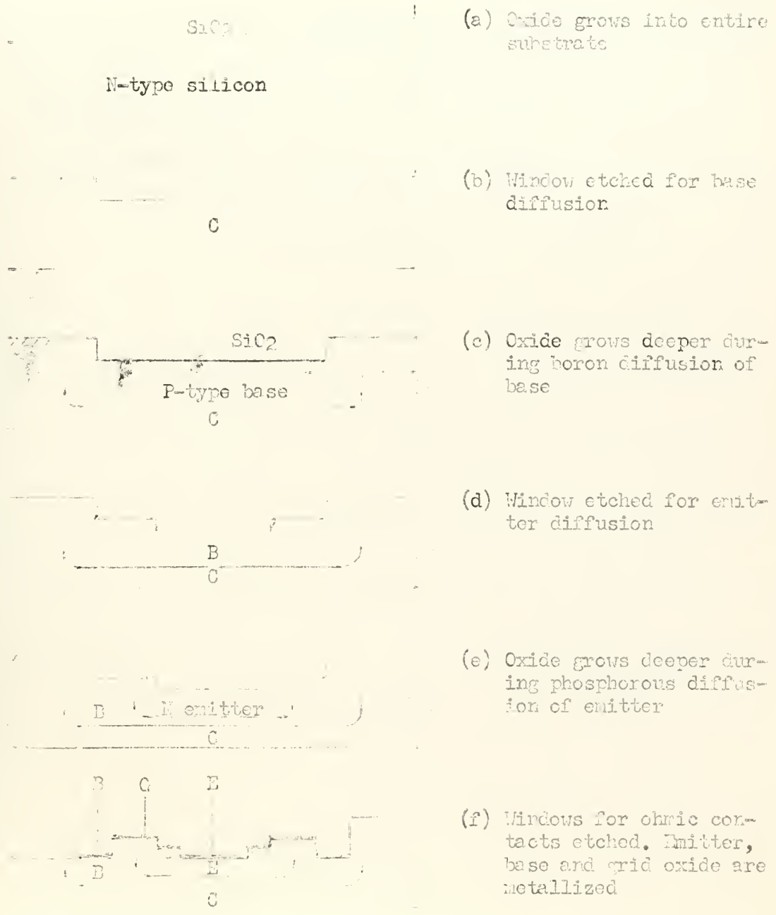
Fig. 1 Method of manufacture of surface-potential controlled transistor.
