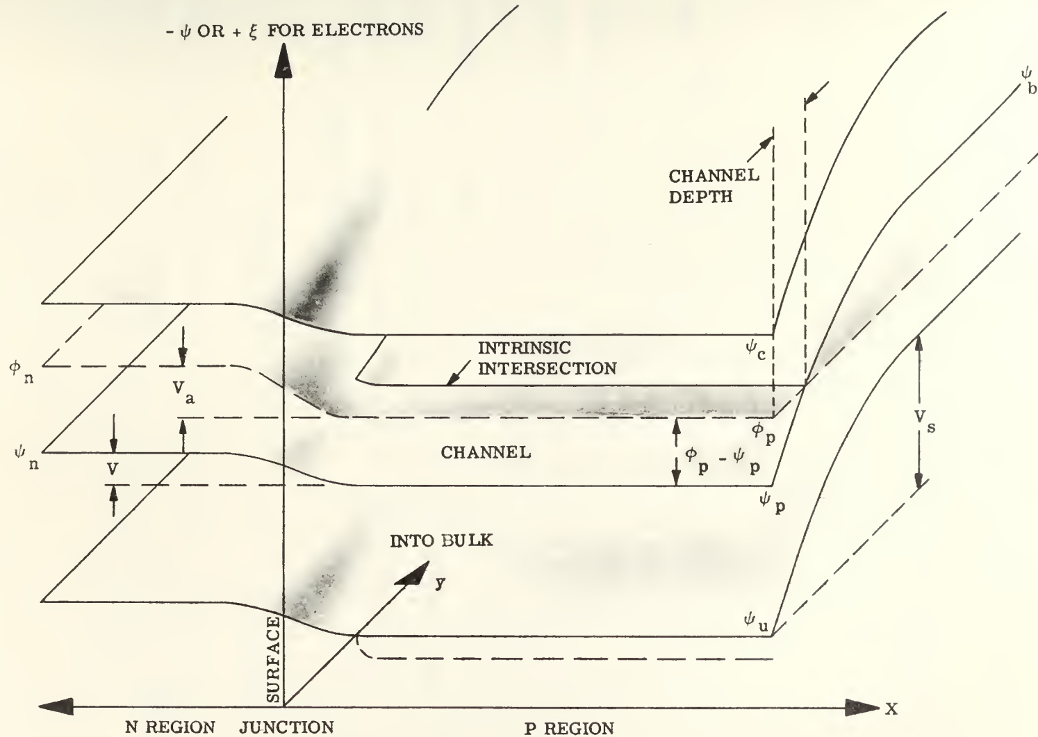
Fig. 5d Junction with forward bias V_a and applied surface potential V_g . Notice that the intrinsic intersection no longer touches surface. An n-type layer has been formed on the surface.
