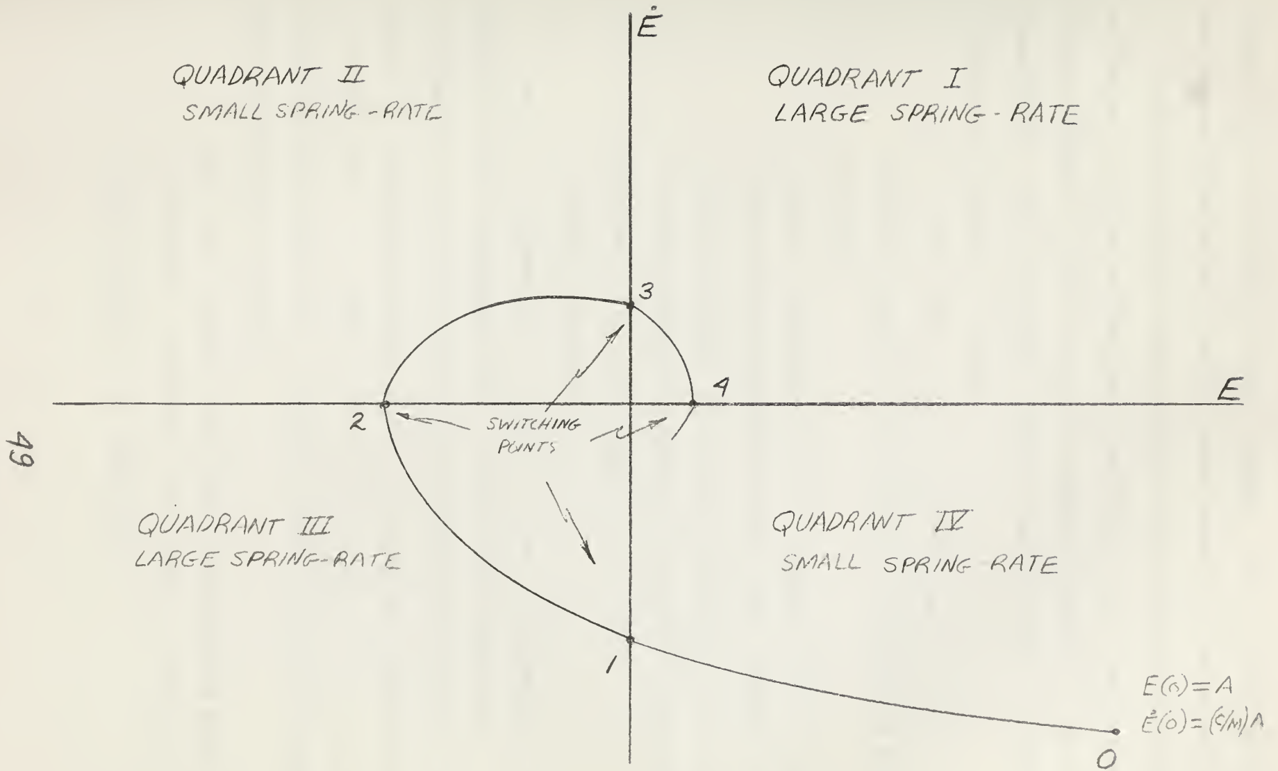
Fig. 7-1 Typical Phase Portrait for the Two-rate Spring Suspension
