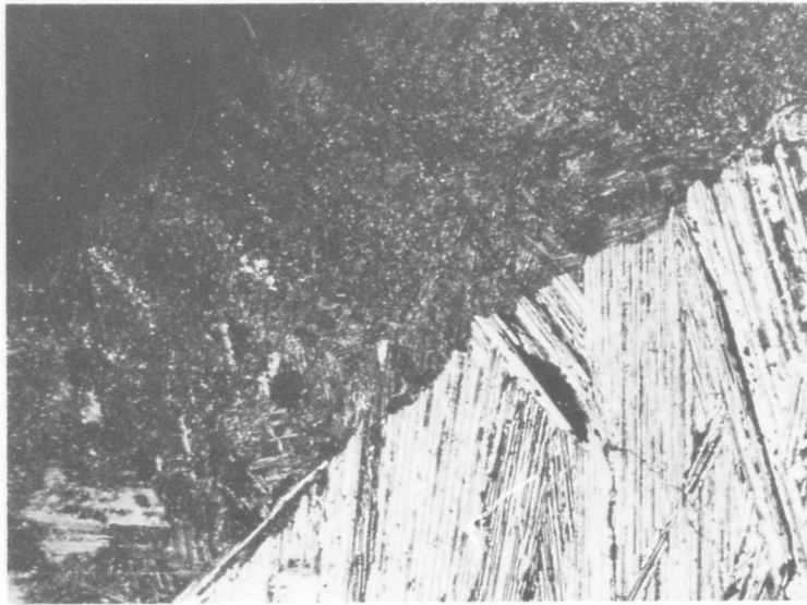
Figure 20. Diffusion Couple (W + 32 At% C)-- Graphite X100 (10 Minutes at 2680°C, Radiation-Cooled)
