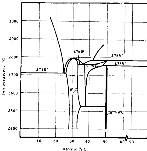
Figure 3. Tungsten-Carbon Phase Diagram. (R. T. Doloff and R. V. Sara, 1962)
