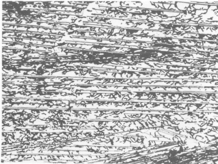
Figure 21. W-C (33.5 At% C), Quenched at \sim 100^\circ C per X250 Second from 2650°C.
