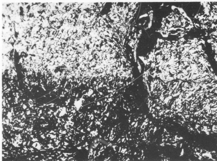
Figure 24. Diffusion Couple (W-32 At% C) -Graphite X150 10 Minutes at 2680°C, Radiation-Cooled
