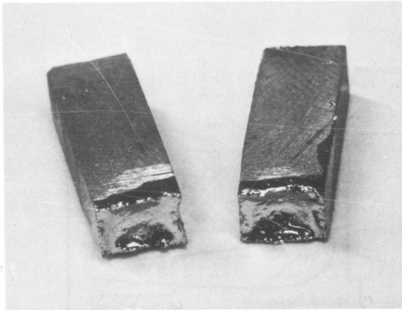
Figure 7. Tungsten Melting Point Specimen After the Run.
