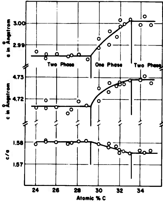
Figure 29. Lattice Parameters of W_2C . (Alloys Quenched from 2200^\circ C )
