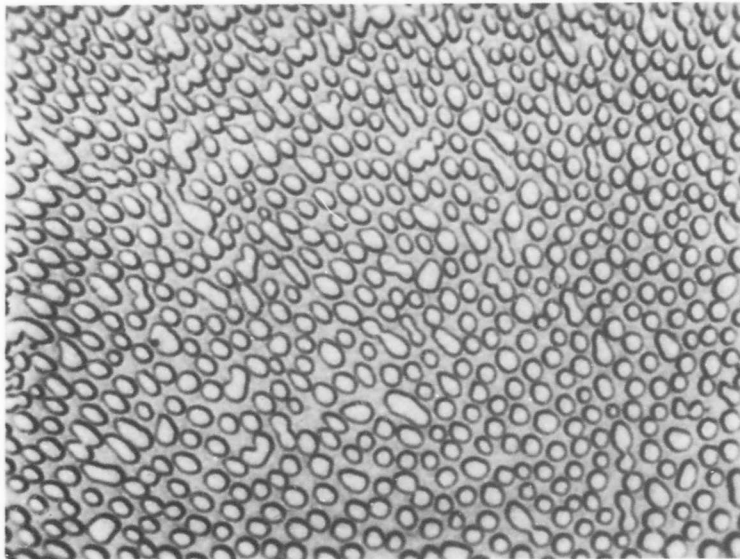
Figure 14. W-C (21.5 At% C), Quenched at \sim 80^\circ\text{C} per Second from 2720^\circ\text{C} . X2500
