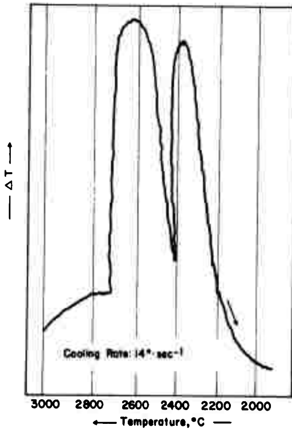
Figure 39. DTA-Thermogram of a W-C Alloy with 43 Atomic Percent Carbon.
