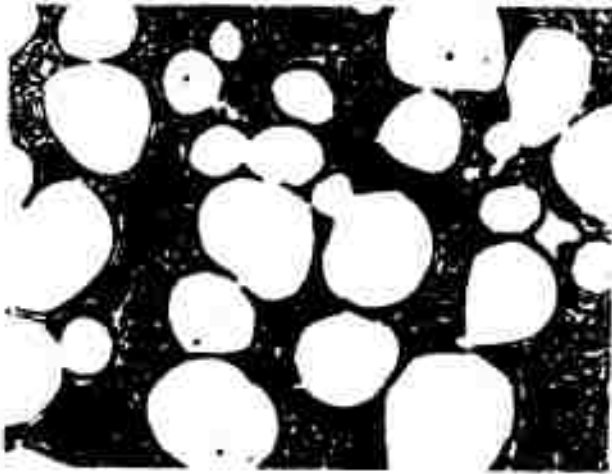
Figure 9. W-C (15 At% C), Cooled at \sim 80^{\circ}\text{C} per Second from 2820^{\circ}\text{C} . X1000 Primary Crystallized Tungsten in a W + \text{W}_2\text{C} Eutectic Matrix.
