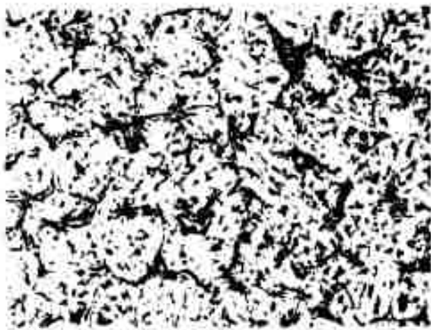
Figure 9. Zr-B (5 At% B), Tin-Quenched from 1740°C. X200 Primary \beta -Zirconium(Transformed), and \text{Zr} + \text{ZrB}_2 Eutectic.
