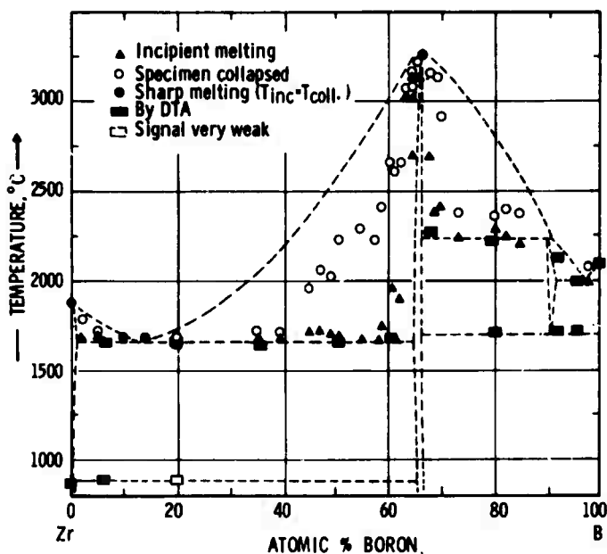
Figure 7. Melting Temperatures and Solid State Reaction Isotherms in the Zirconium-Boron System
