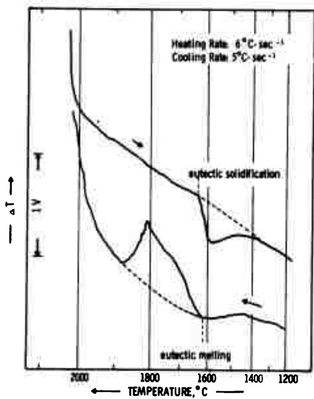
Figure 8. DTA-Thermogram of a Zirconium-Boron Alloy with 50 Atomic Percent Boron.
