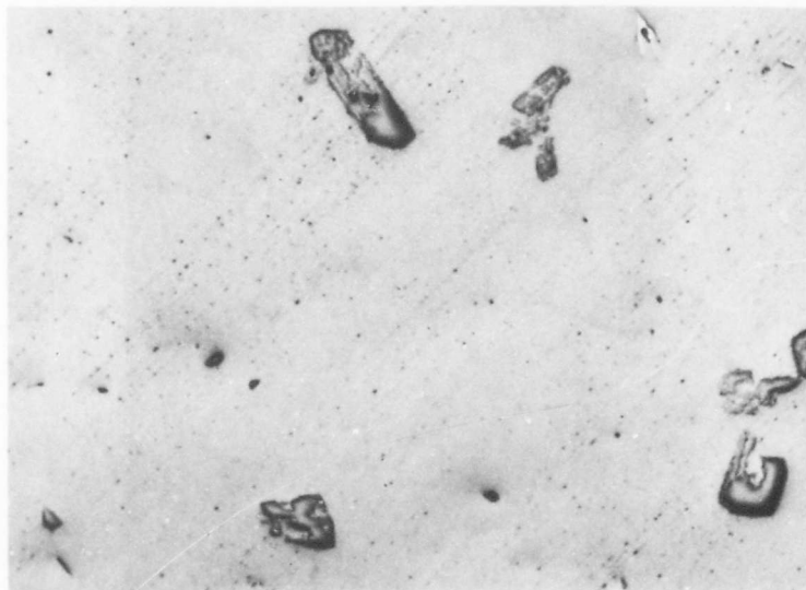
Figure 27. Zr-B (99 At% B), Cooled with Approximately 10°C per Second from 2100°C. X250
