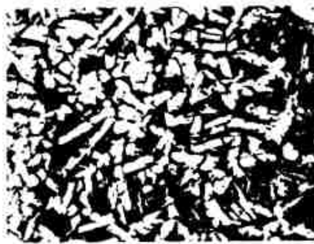
Figure 3. Zr-B (1.8 At% B), Quenched with \sim 80^\circ\text{C} per Second from 1790^\circ\text{C} . X500
