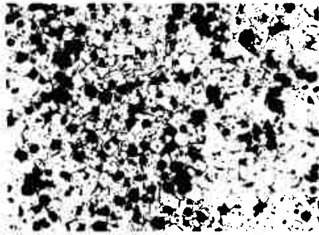
Figure 5. Zr-B (50 At% B), with 3 At% Carbon Added Alloy Quenched from 1800°C.
