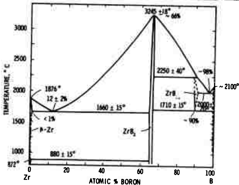
Figure 1. Constitution Diagram Zirconium-Boron
