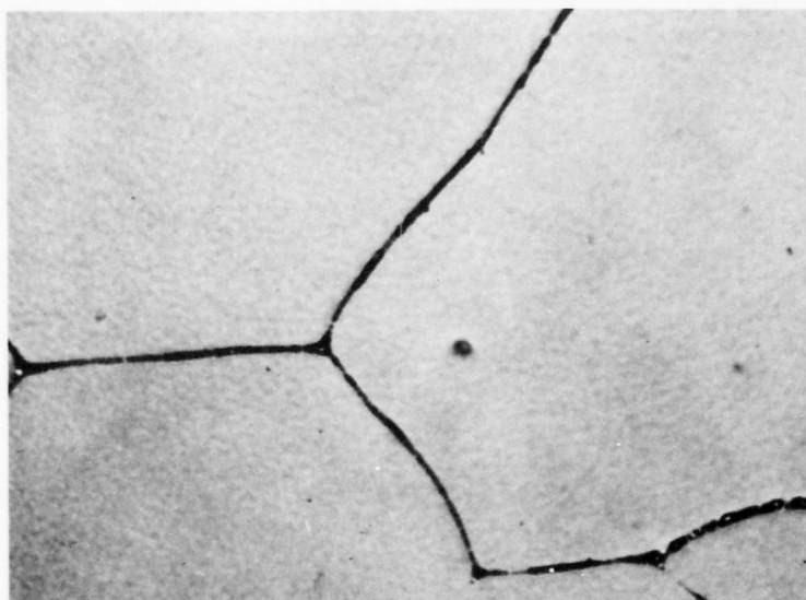
Figure 14. Zr-B (65.4 At% B), Quenched from 2600°C. X1000 \text{ZrB}_2 , and Small Amounts of Grain-Boundary Zirconium.
