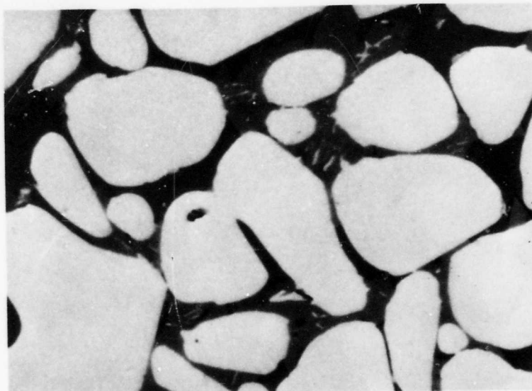
Figure 21. Zr-B (80 At% B), Cooled with Approximately 20°C per Second from 2280°C. X950 Primary \text{ZrB}_2 (Light), \text{ZrB}_{12} , and Boron.
