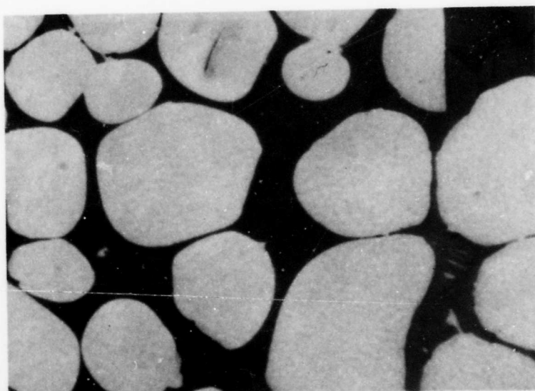
Figure 22. Zr-B (80 At% B), Partially Melted at 2280°C, X1000 Reannealed at 2200°C, and Quenched. \text{ZrB}_2 (Light), \text{ZrB}_{12} (Matrix), and Small Amounts of Boron.
