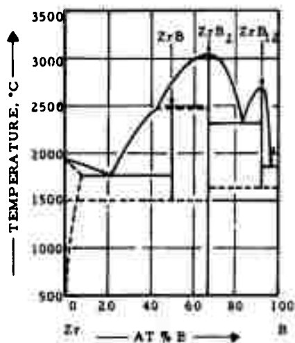
Figure 2. Phase Diagram Zirconium-Boron (F. W. Glaser and B. Post, 1963, W. Schedler 1951; Work Quoted by R. Kieffer and F. Benesovsky, 1963)
