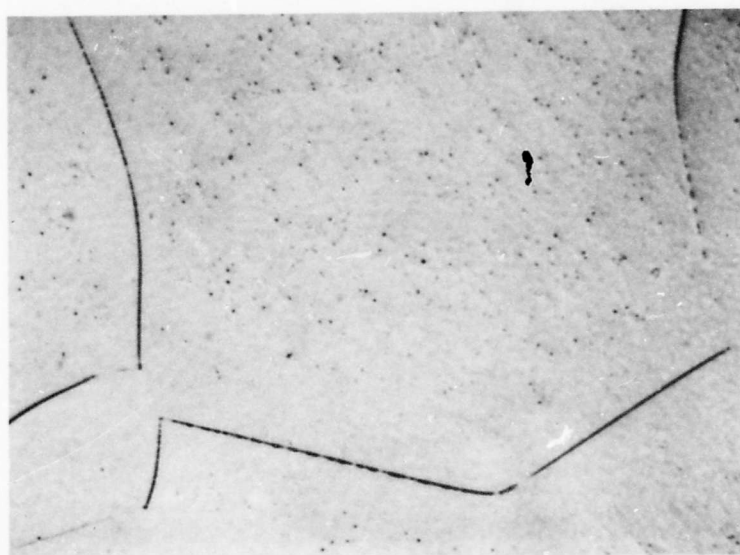
Figure 15. Zr-B (65.8 At% B), Quenched from 3000°C. X850 Low-Boron Boundary of \text{ZrB}_2 ; Minute Traces of Second Phase Zirconium are Still Visible at the Grain Boundaries.
