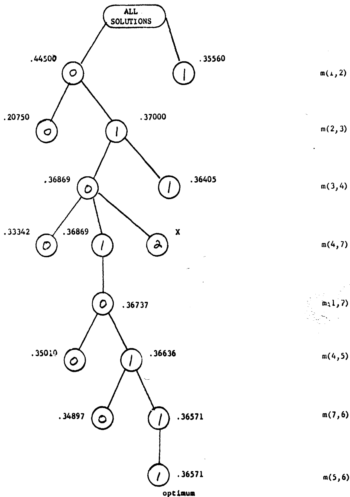
Figure 7. Tree for network example. Labels on the nodes are the calculated upper bounds on the objective function. The objective function is a weighted sum of arterial bandwidths. Numbers inside the nodes are values for the m_i shown at right. Cycle constraints have been used to limit the possible choices of m(1,7) and m(5,6) .
