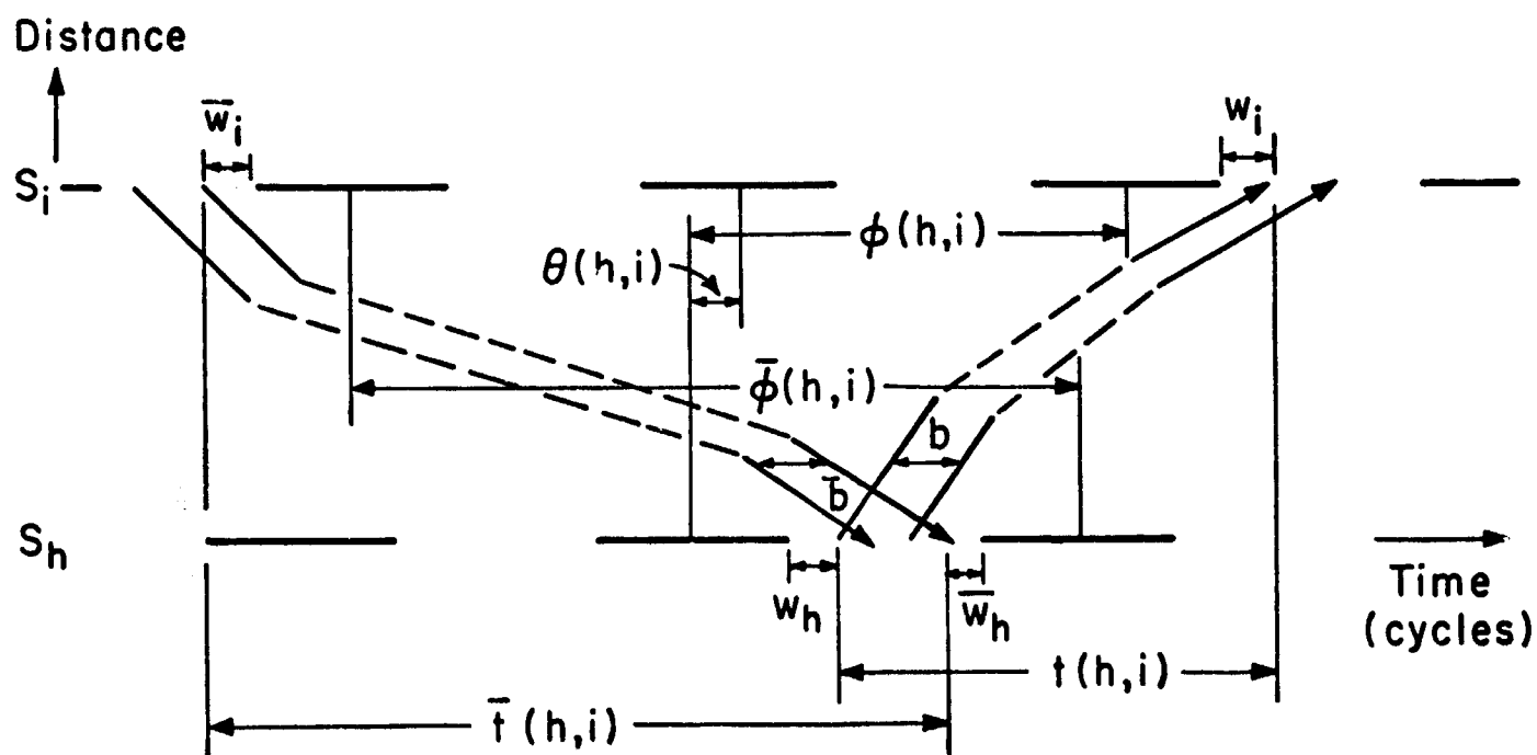
Figure 2. Geometry of green bands. Notice that \theta(h,i) + \bar{\theta}(h,i) must equal an integer.
