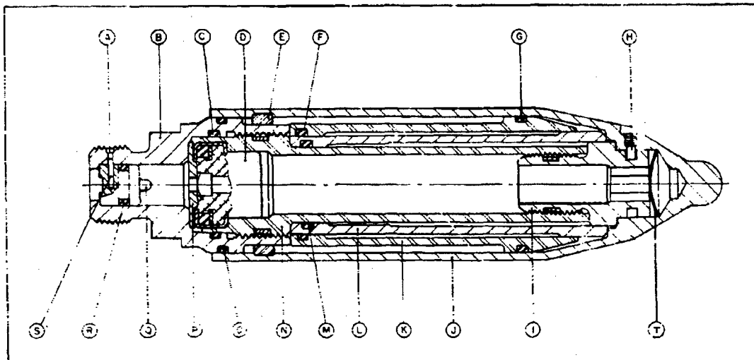
CROSS-SECTION DRAWING
