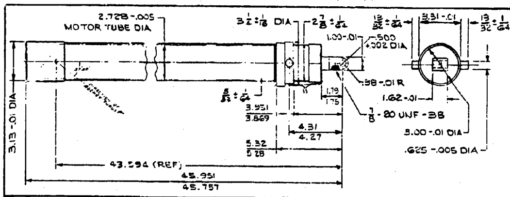
ENVELOPE DRAWING
