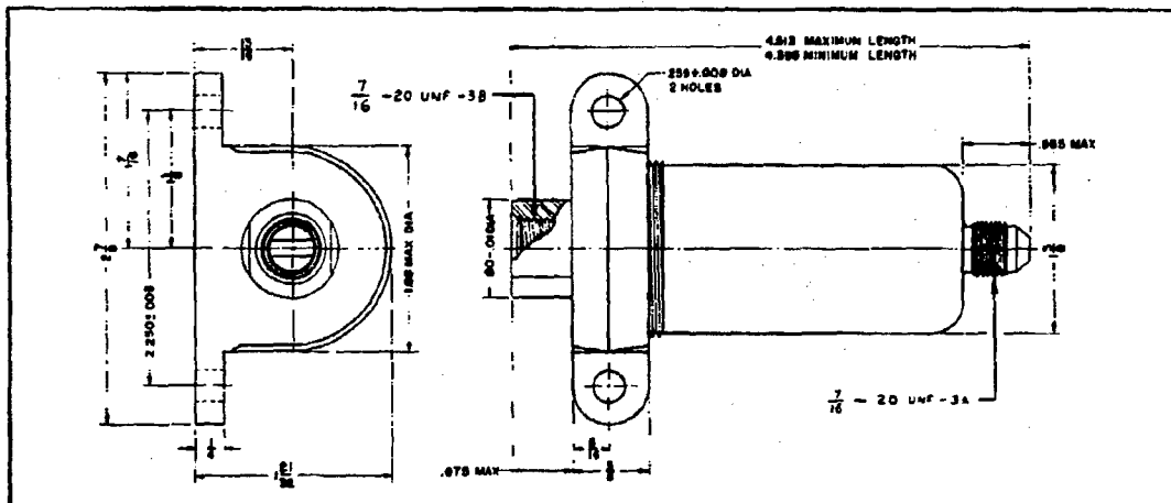
ENVELOPE DRAWING
