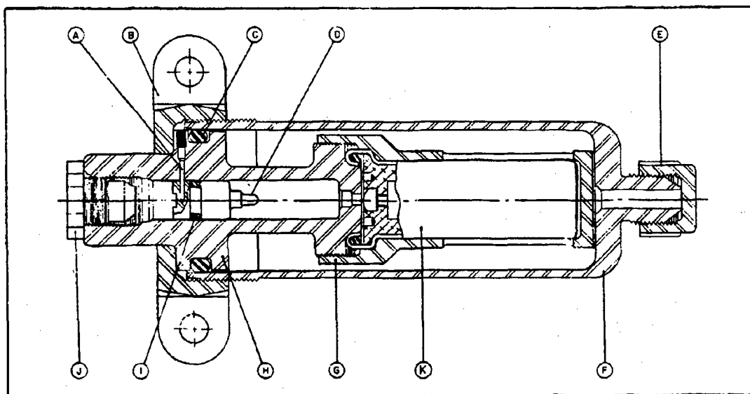
CROSS-SECTION DRAWING
