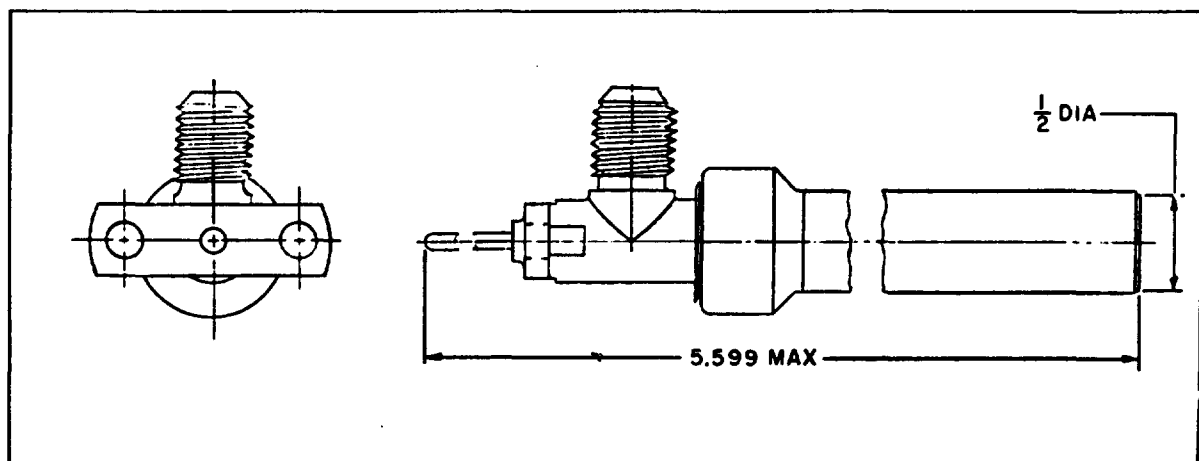
ENVELOPE DRAWING
