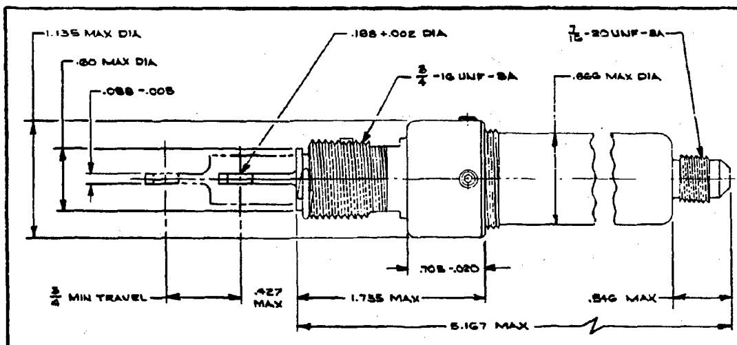
ENVELOPE DRAWING
