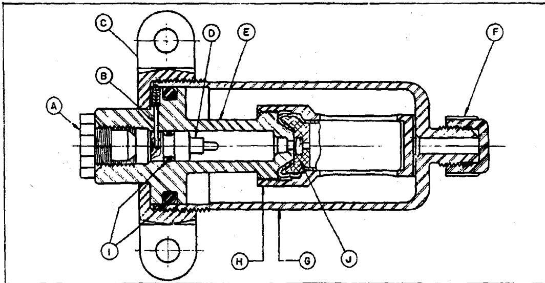
CROSS-SECTION DRAWING
