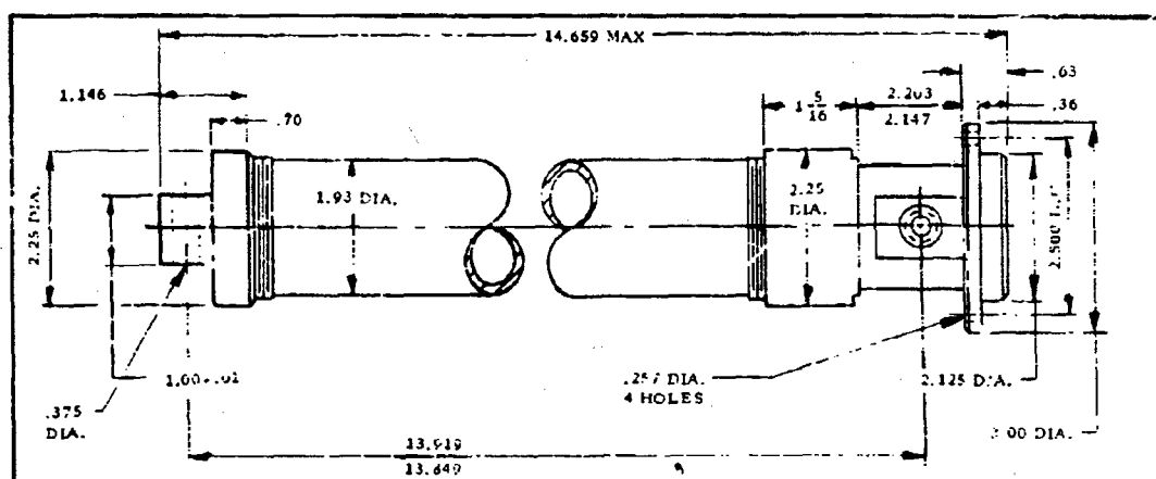
ENVELOPE DRAWING
