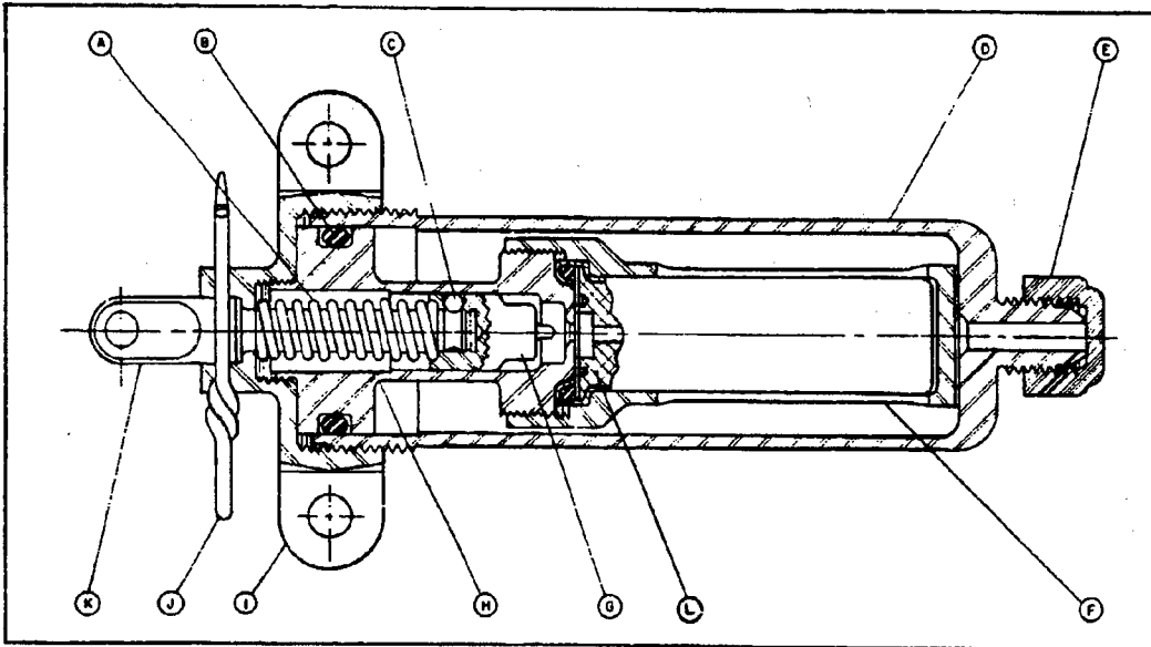
CROSS-SECTION DRAWING
