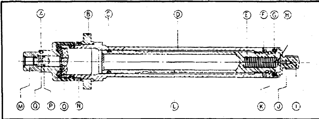
CROSS-SECTION DRAWING
