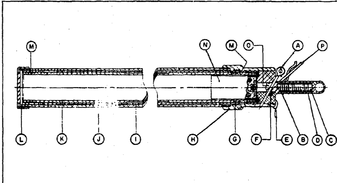
CROSS-SECTION DRAWING
