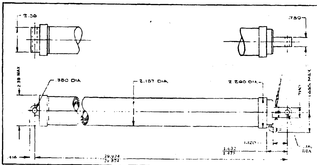
ENVELOPE DRAWING
