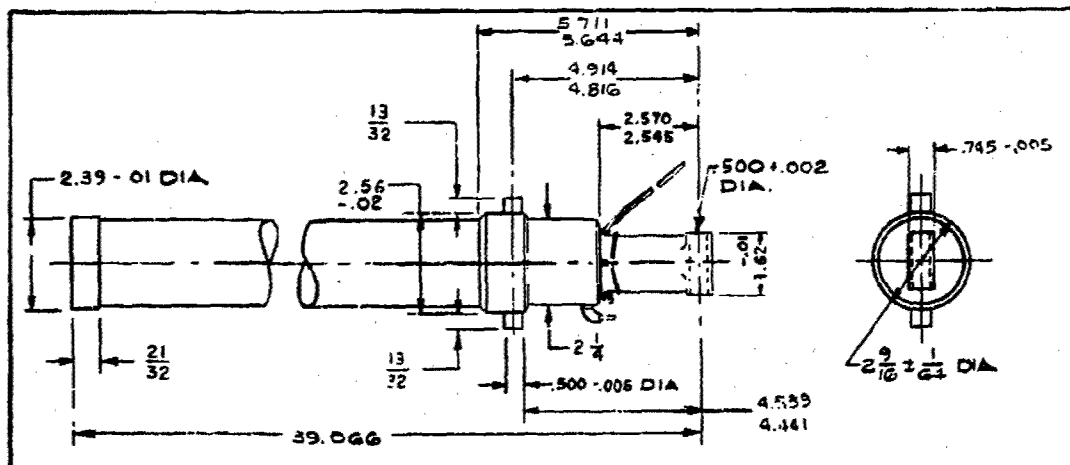
ENVELOPE DRAWING
