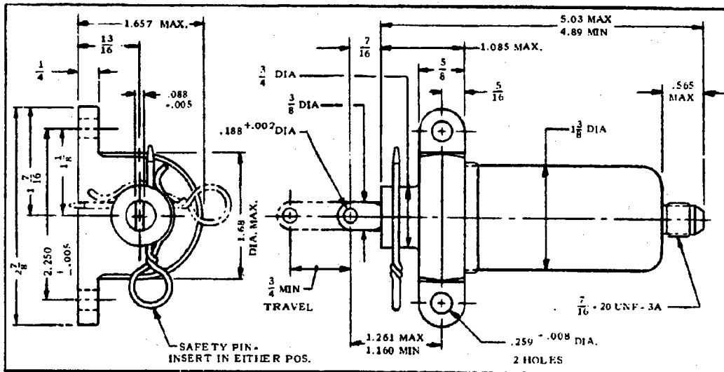
ENVELOPE DRAWING
