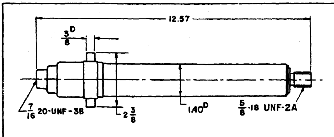
ENVELOPE DRAWING
