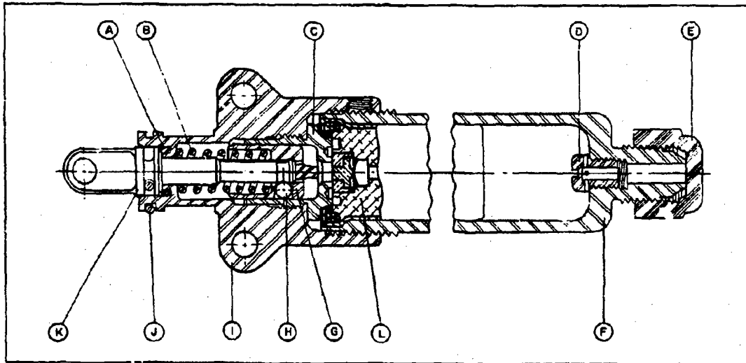
CROSS-SECTION DRAWING
