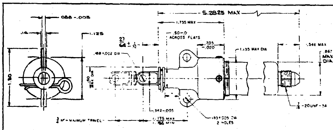
ENVELOPE DRAWING
