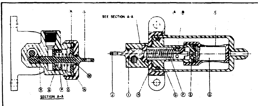
CROSS-SECTION DRAWING
