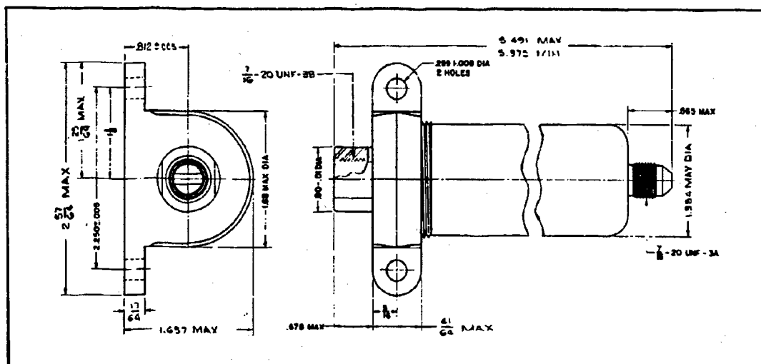
ENVELOPE DRAWING
