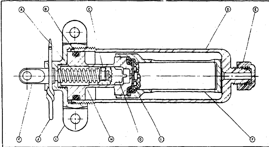
CROSS-SECTION DRAWING
