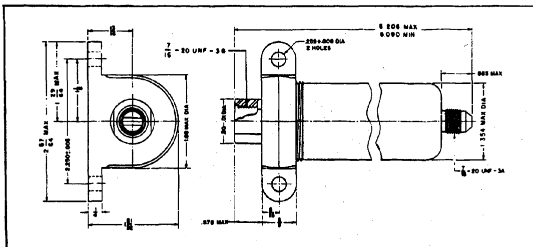
ENVELOPE DRAWING
