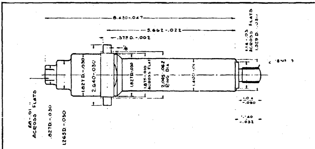
ENVELOPE DRAWING
