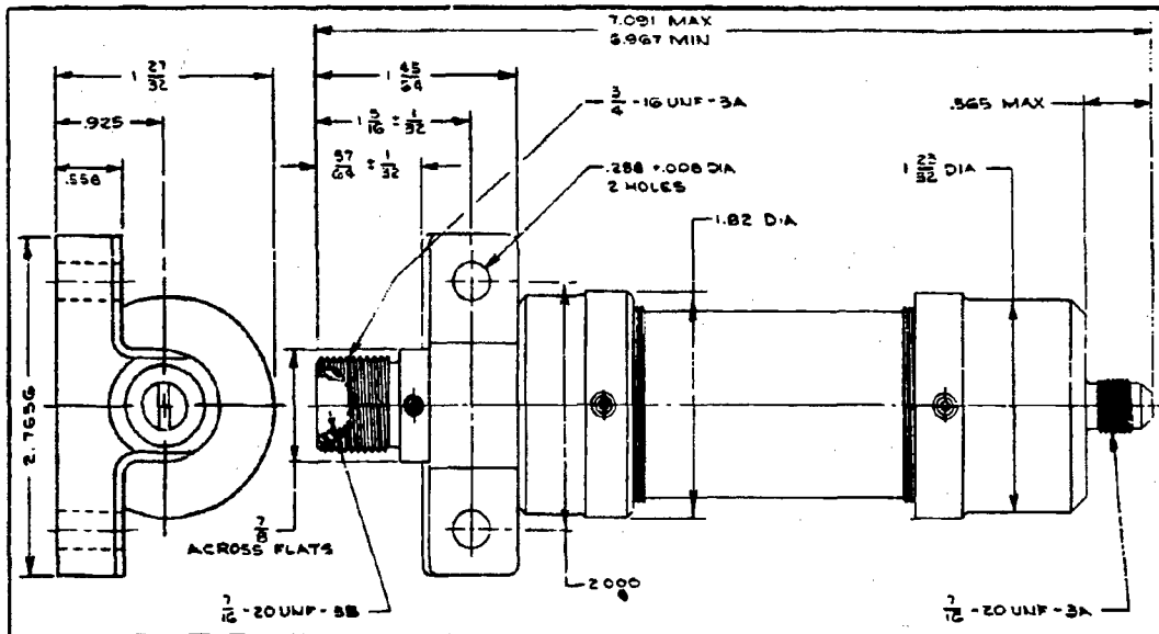
ENVELOPE DRAWING
