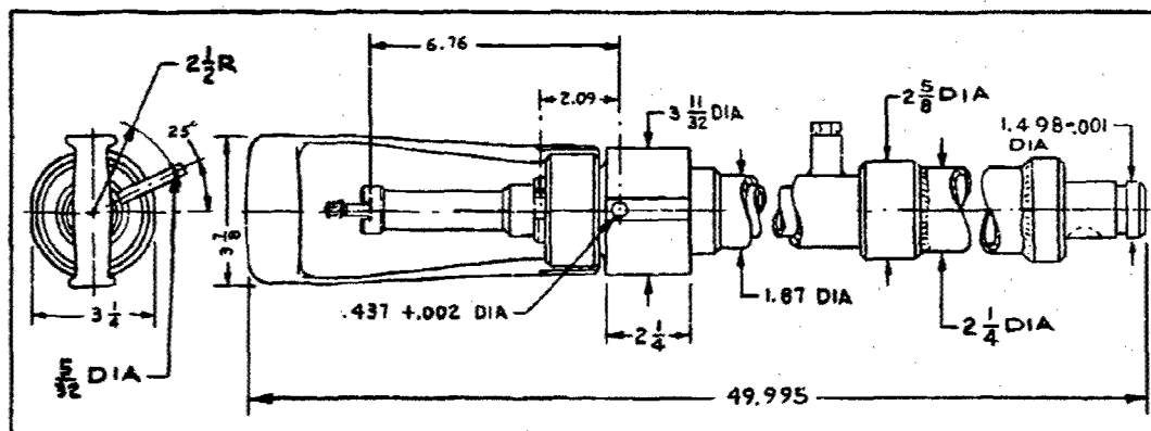
ENVELOPE DRAWING
