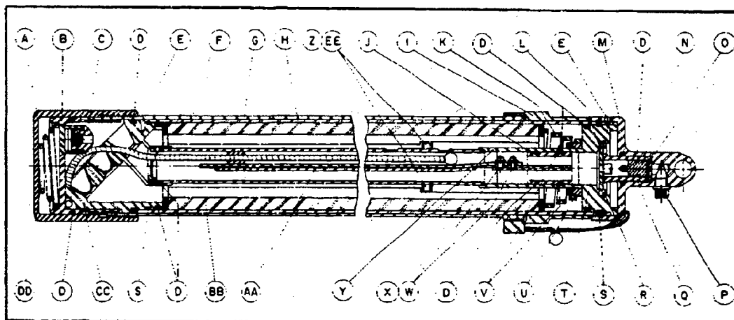
CROSS-SECTION DRAWING
