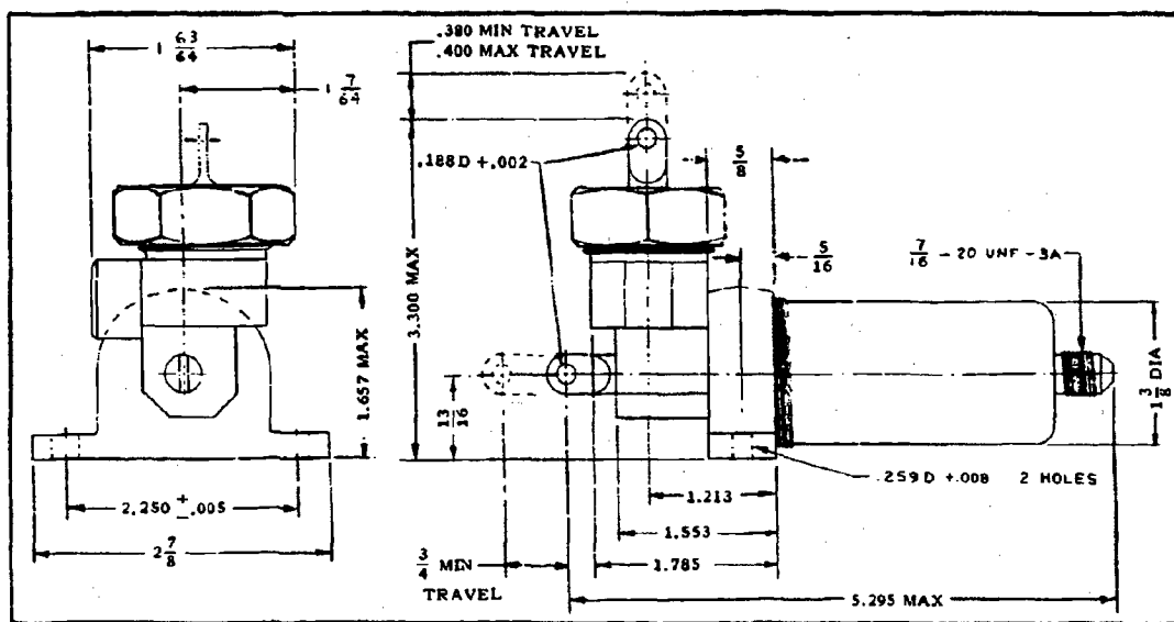
ENVELOPE DRAWING
