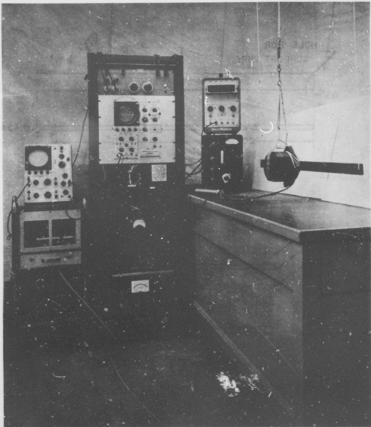
TEST SET-UP FIGURE (4)
