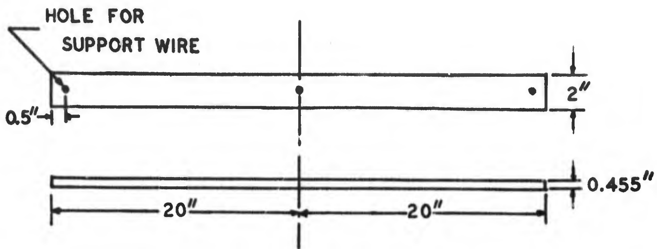
BEAM DIMENSIONS
