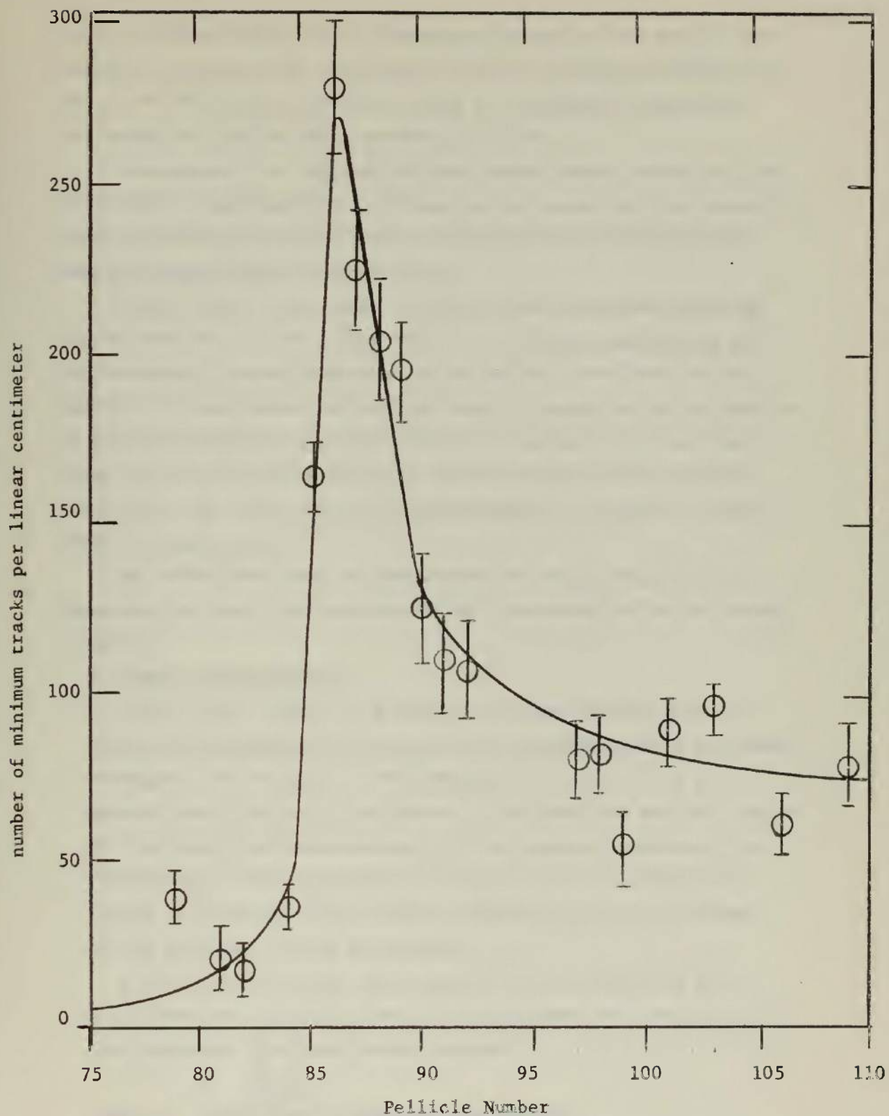
Figure 3. Experimental determination of the number of minimum tracks per linear centimeter at the center of the face as a function of pellicle number.
