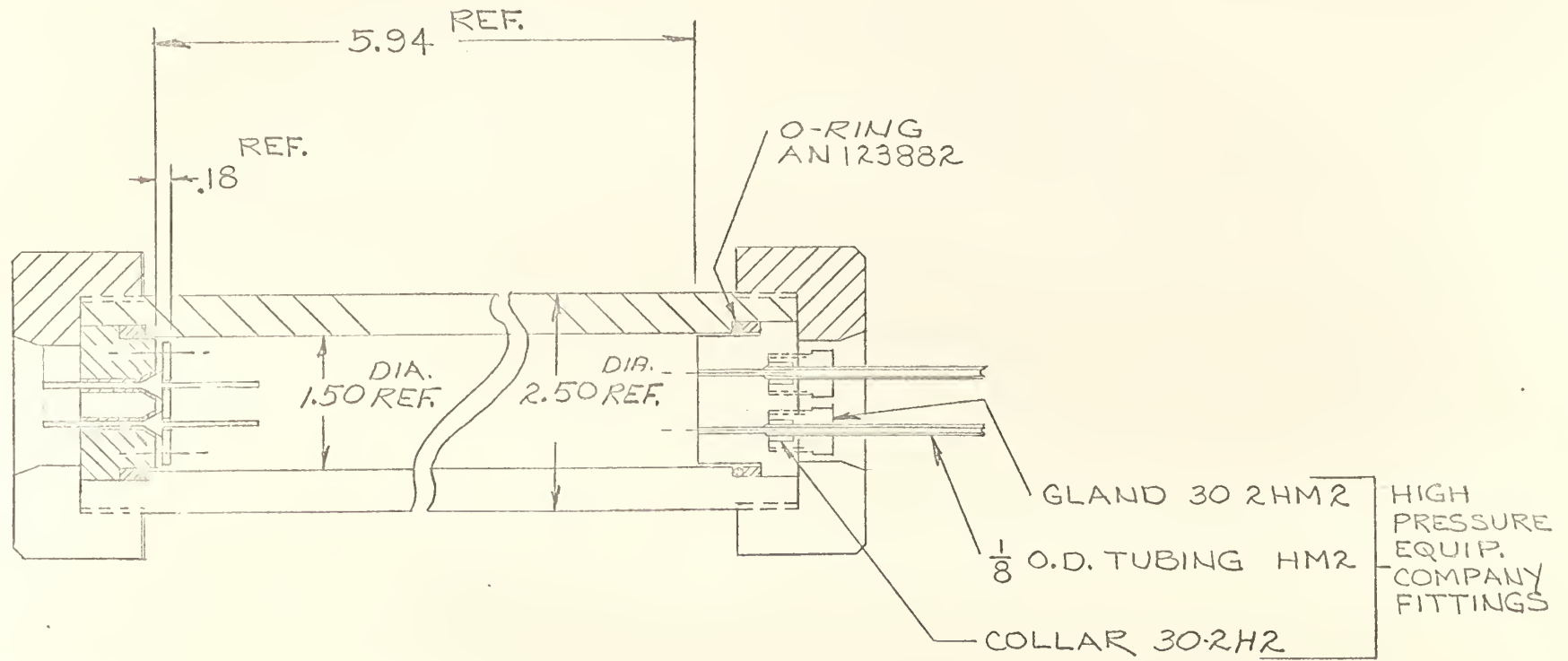
Figure 29. Detailed Drawing of Cylindrical Transducer
