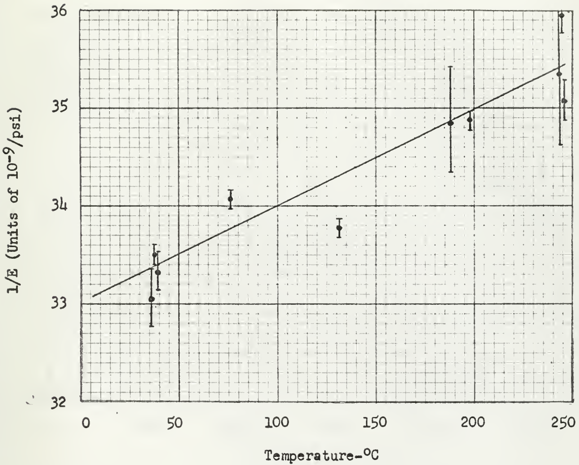
Figure 5. 1/E versus temperature. Values shown were determined from a statistical study of experimental points of stress-strain tests at constant temperatures (see Appendix I). Dot in center of \bar{I} indicates most probable value. One standard deviation above and below most probable value is indicated by vertical line through dot.
