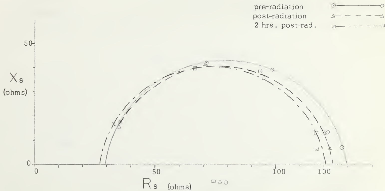
Figure 8. Series Impedance Locus of a Typical Unirradiated Control Sample Measured at Times Corresponding to Those of the X-Irradiated Sample of Figure 7.
