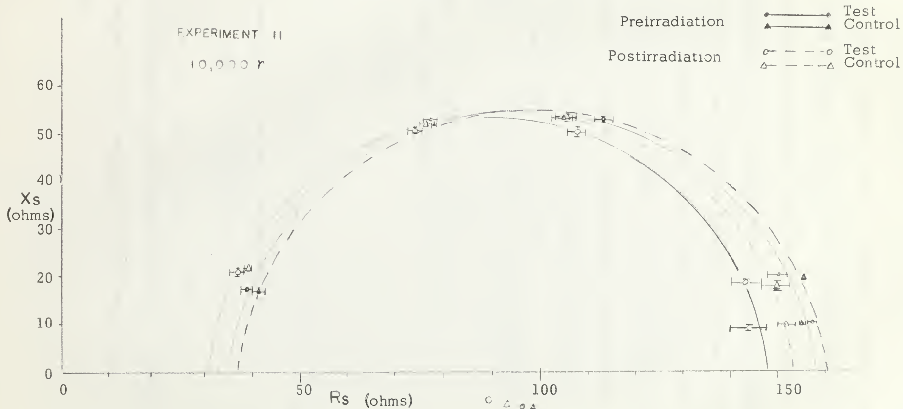
Figure 9. Series Impedance Locus on Irradiated Sample and Irradiated Control for One X-Irradiation of 10,000 r. (Mean Values of Six Samples).
