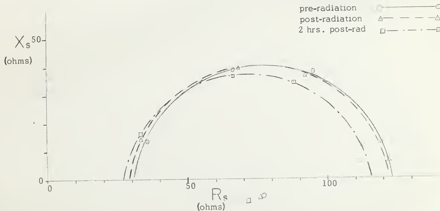
Figure 7. Series Impedance Locus of a Typical Irradiated Before and After 10,000 r of X-Irradiation
