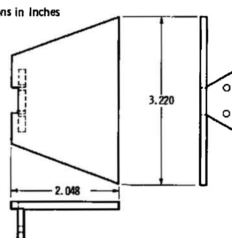
Trim Tab No. 3
