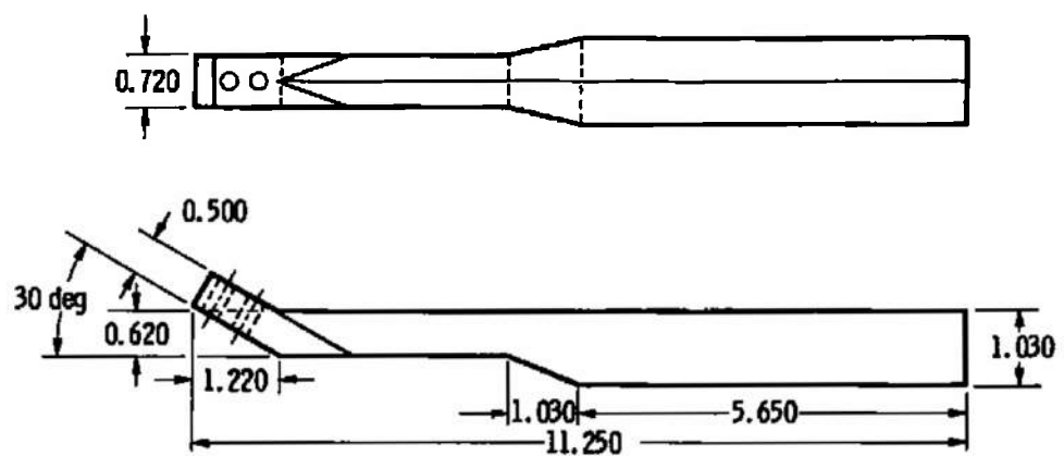
Lower Boom (2 Required)
