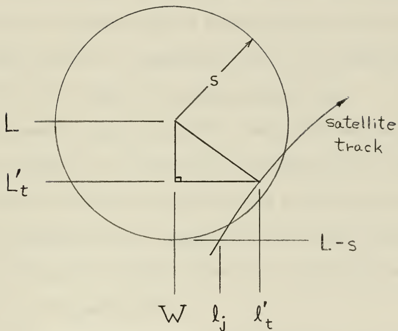
Fig.A-3: Mercator projection of track; special case
