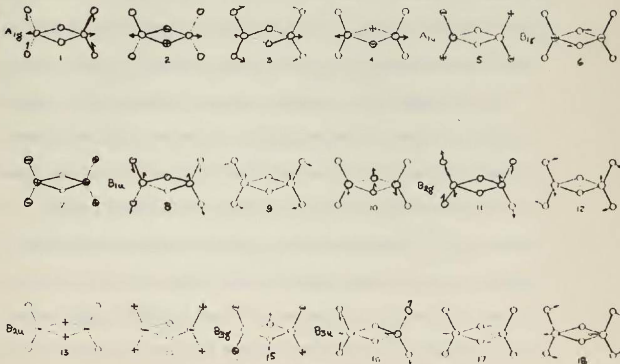
FIG. 9 The character of the normal vibrations of "bridge" diborane. After Behr and Longuet-Elg (33, 35.)
