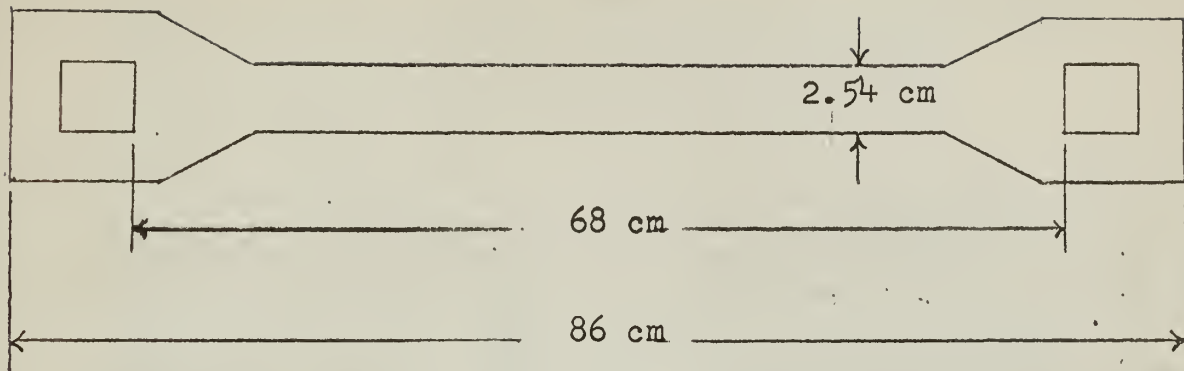
Discharge Tube I
