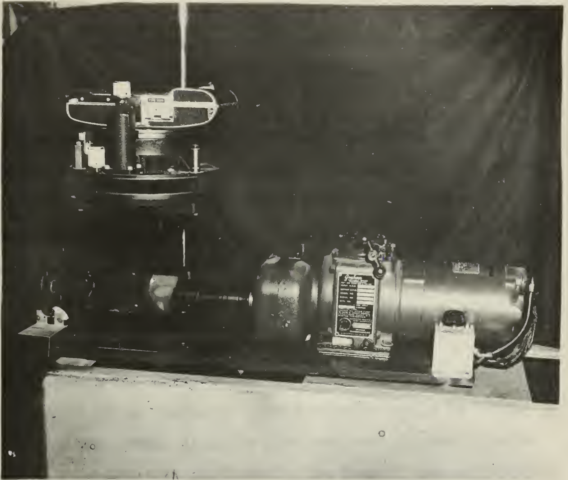
Figure 8 - Rotating mirror and camera assemblies
