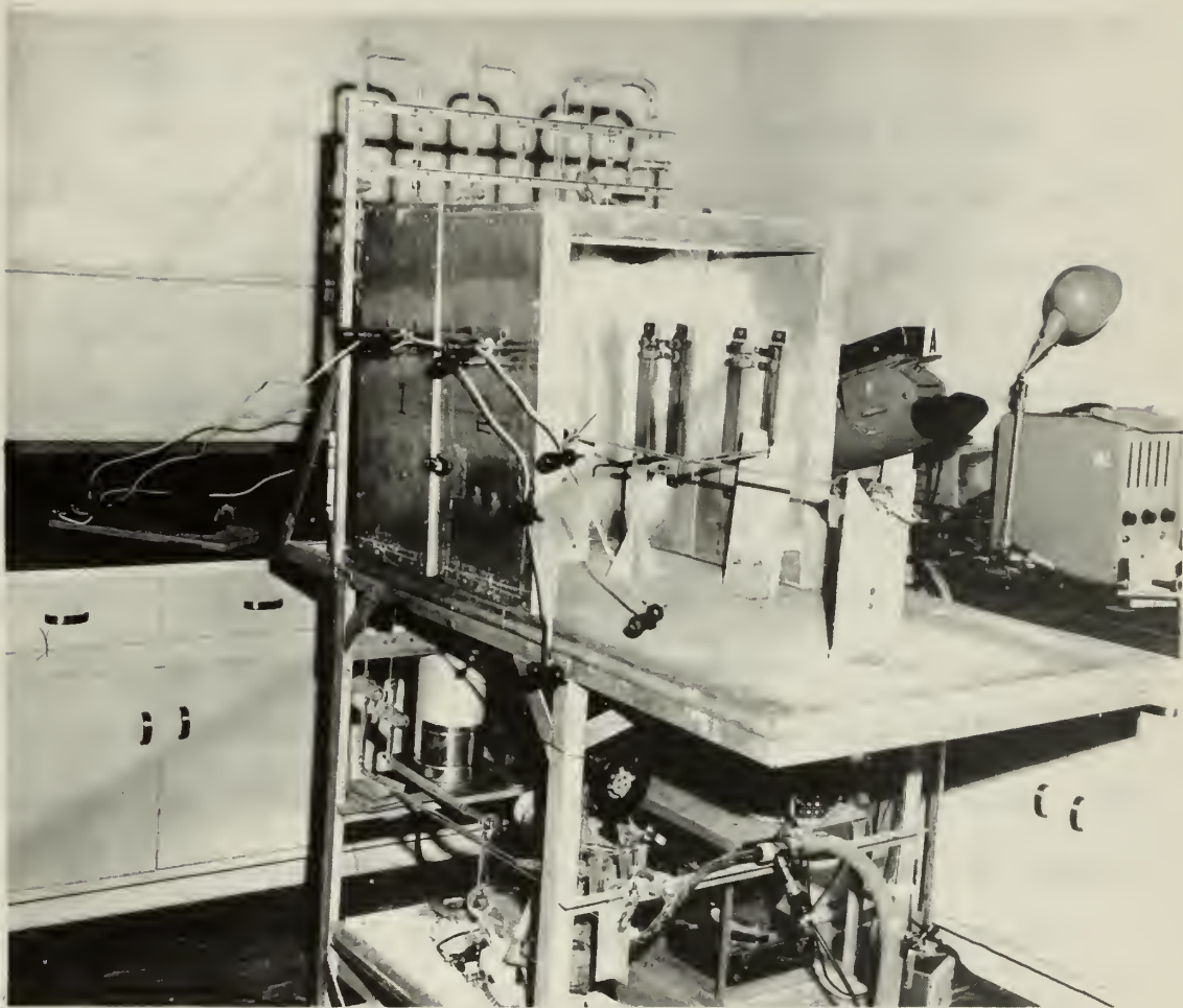
Figure 3 - Partially assembled over B position.
