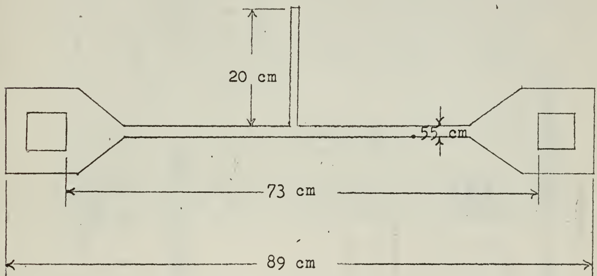
Discharge Tube II
