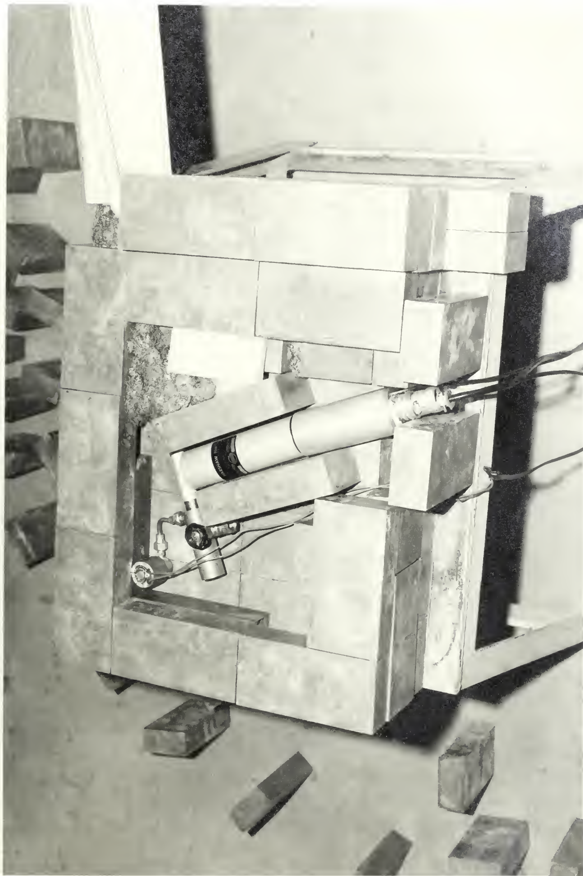
Figure 5. Two-Way Valve and Actuator (Top View)
