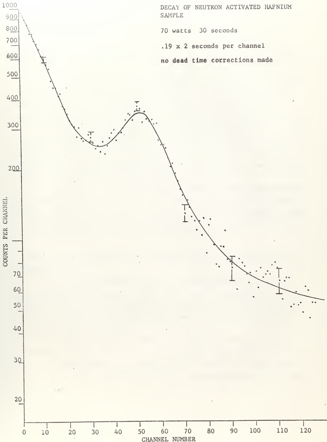
Figure 13. Decay of Neutron Activated Hf Sample
