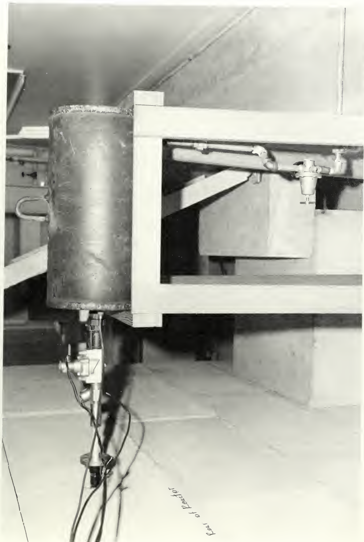
FIGURE 4. PRESSURE TANK (SIDE VIEW)
