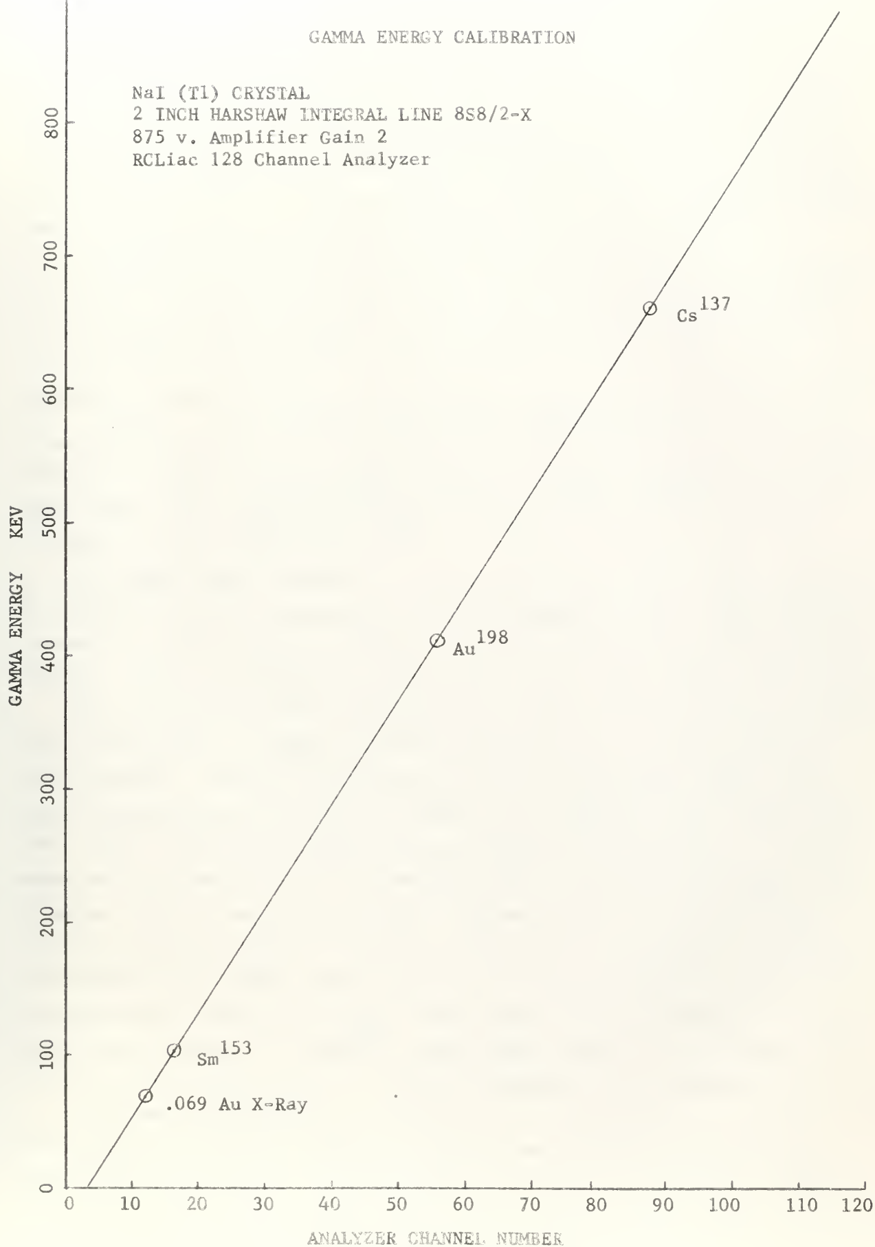
Figure 10. Gamma Energy Calibration
