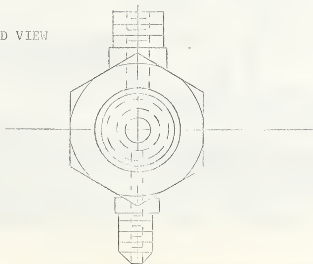
Figure 2. One Way Valve and Seat Assembly
