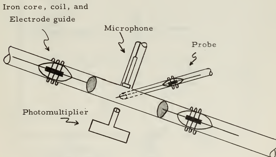
Fig 1B Discharge Tube and Probes (Schematic)
