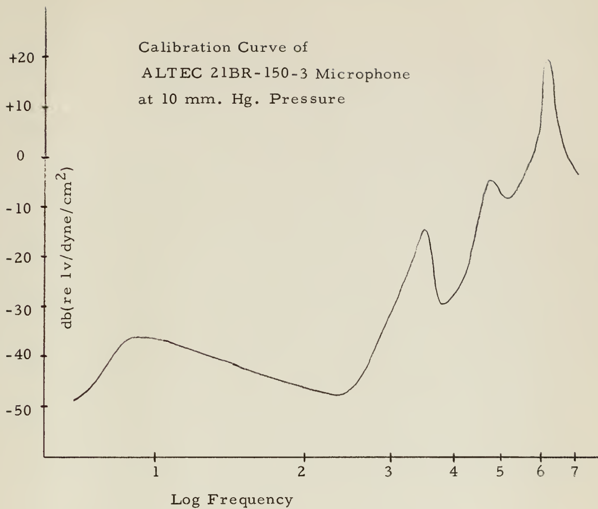
Fig 4. Microphone Calibration Curve
