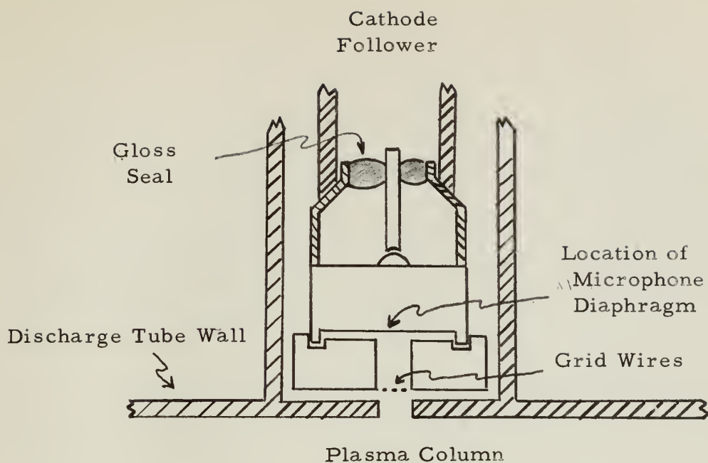
Fig 1A Microphone Detail (Schematic)
