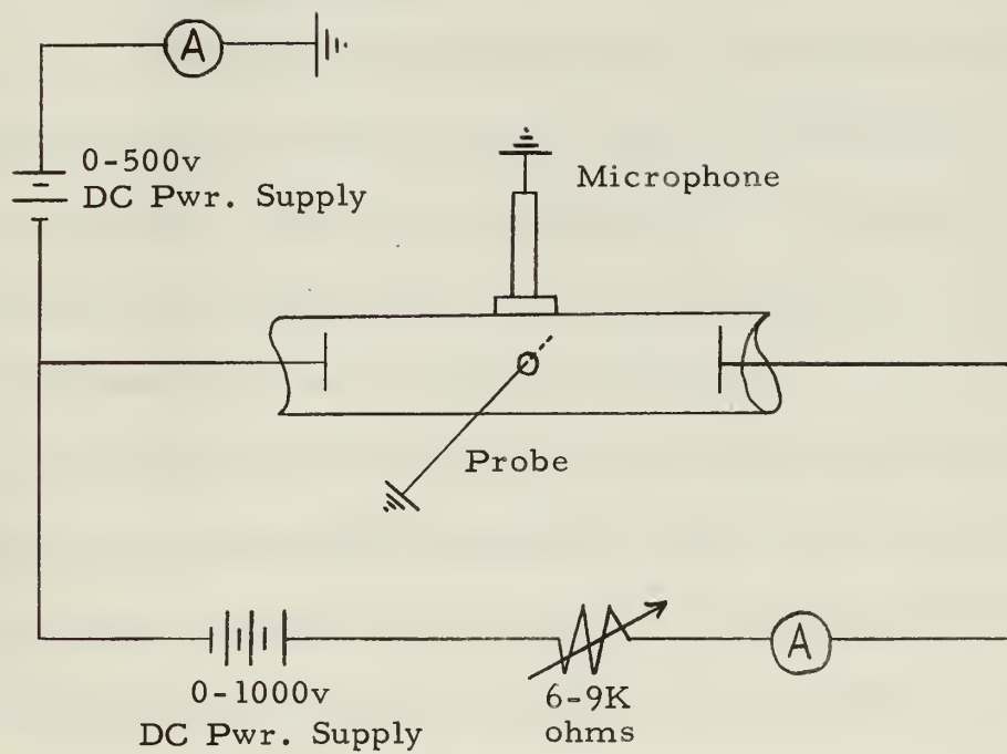
Fig 2. Electrical Discharge Circuit
