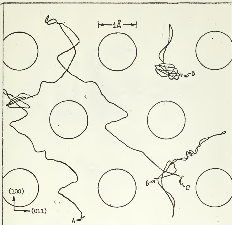
Fig. 2. ROBINSON AND OEN "... (011) channel trajectories onto (01\bar{1}) surface for f.c.c. Cu...(1Kev Cu primaries)...Bohr potential." 13 Points A,B,C and D penetrated 300\text{ \AA} in part of trajectory shown.
