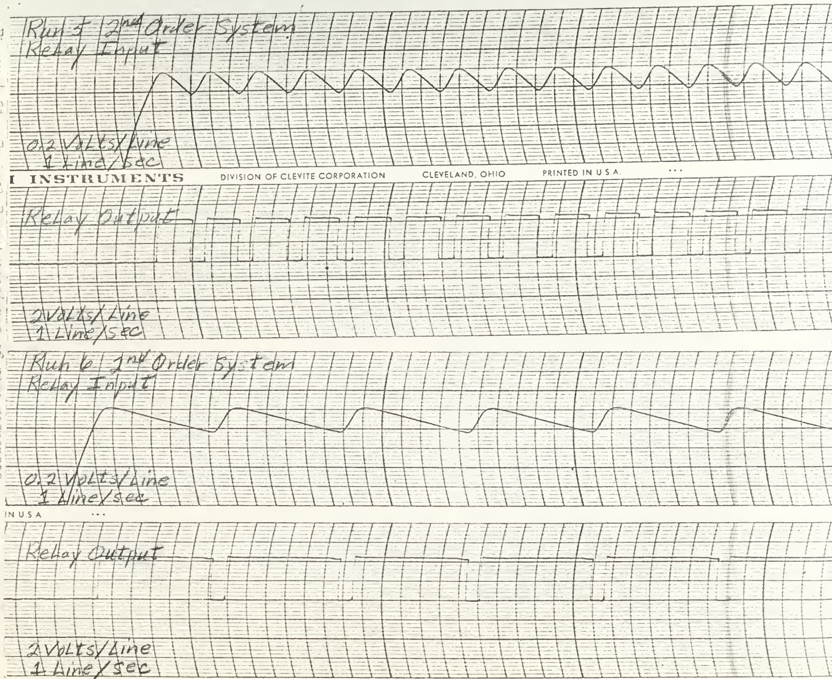
Figure 4.21. Typical Muscovite recordings of ramp responses.
