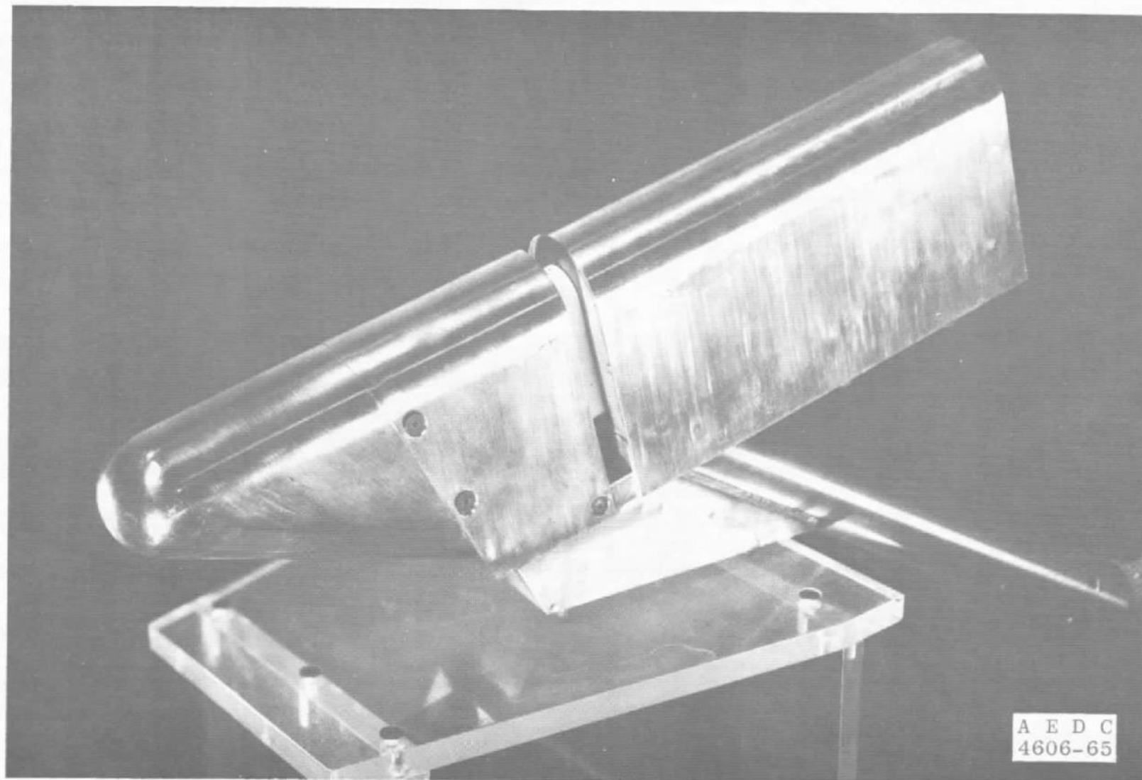
b. Photograph of the Heat-Transfer Model with 0.50-in.-wide Slot
