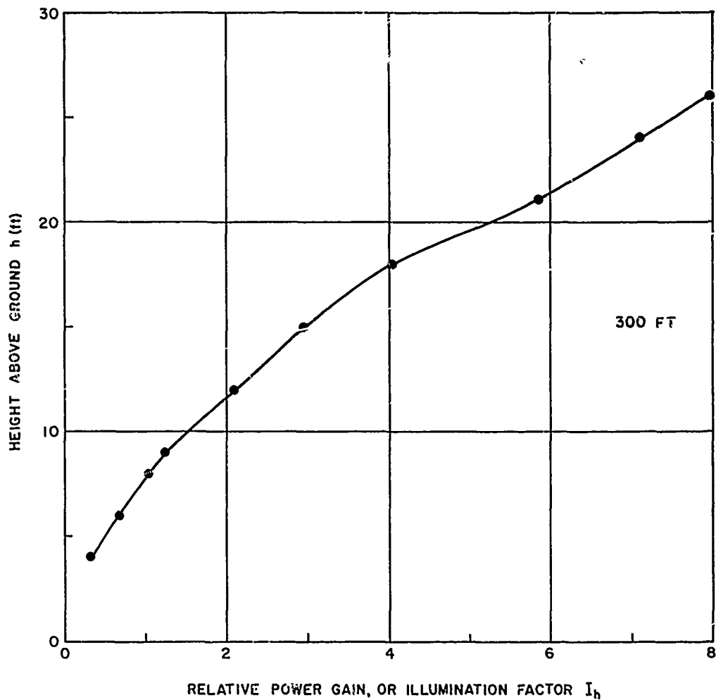
FIG. 12. RELATIVE POWER GAIN OF TRANSMITTING ANTENNA AT VARIOUS HEIGHTS ABOVE THE GROUND, FOR HORIZONTAL POLARIZATION.
