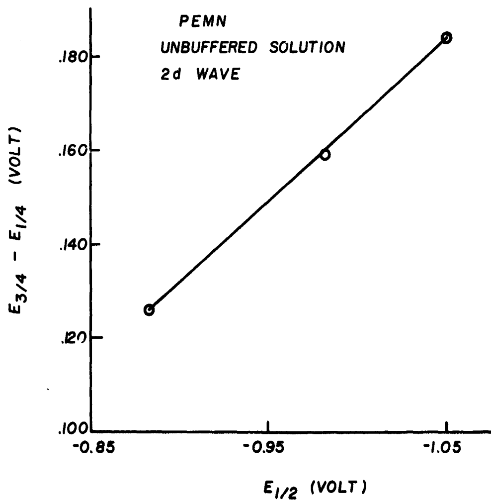
FIG.8 VARIATION OF E_{3/4}, 1/4 WITH E_{1/2}
