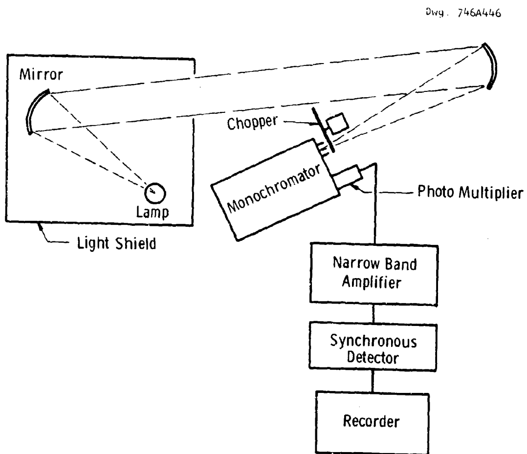
Fig. 96—Arrangement used for taking high resolution spectra
