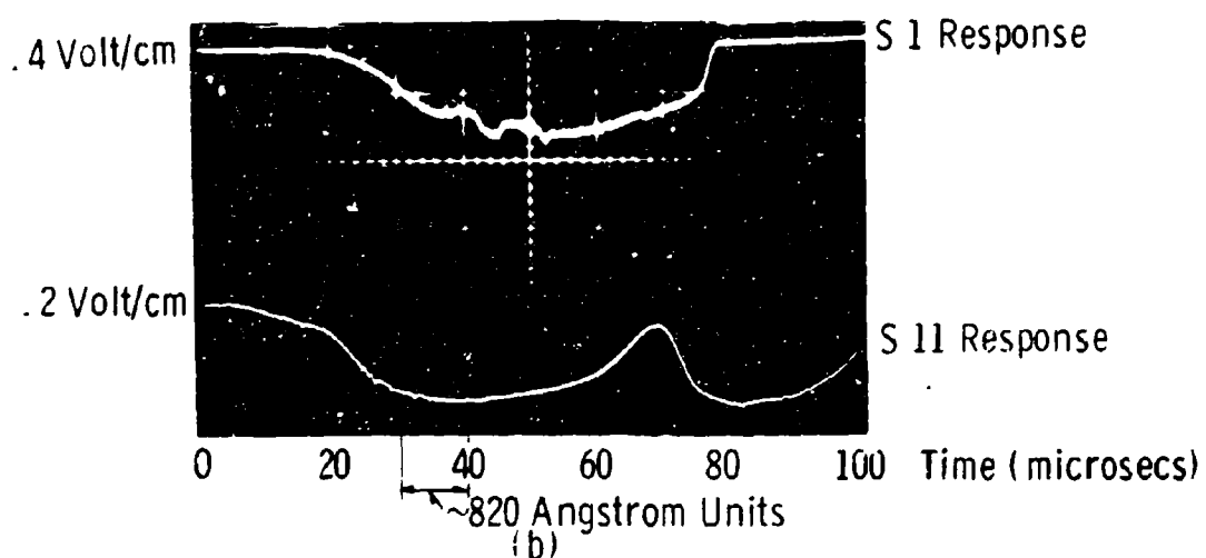
Fig. 82—Xenon flashlamp Energy input 600 joules (1.7KV, 400 \mu f, 100 \mu h)
