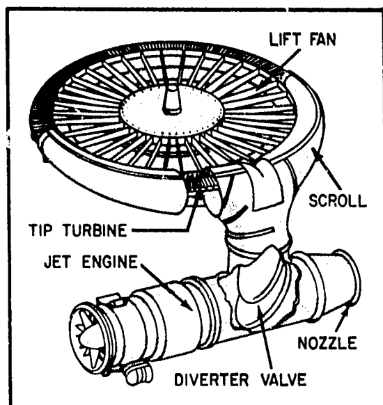
X353-5 WING FAN PROPULSION SYSTEM
