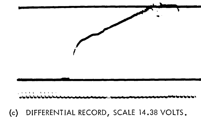
FIG.1 THREE VOLTAGE - TIME RECORDS FOR SHOT 5 ON CAST COMP B WITH 130 CARD GAP
