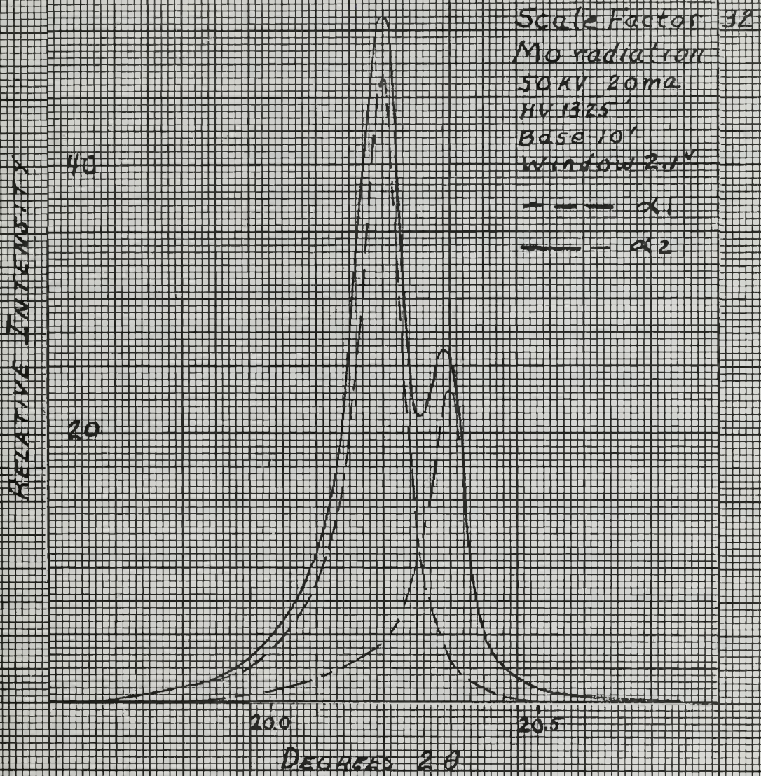
Figure 10: (110) α Peak Ductile specimen
