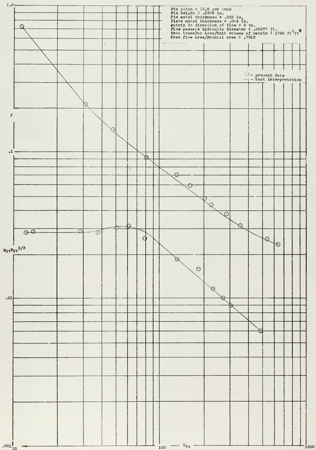
N_{St} N_{Pr}^{2/3} and f versus N_{Re} for 430 stainless steel plate-fin Figure 3
