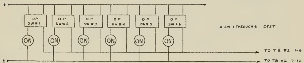
b. Diffusion Pump Heater Switch and Indicator Circuit
