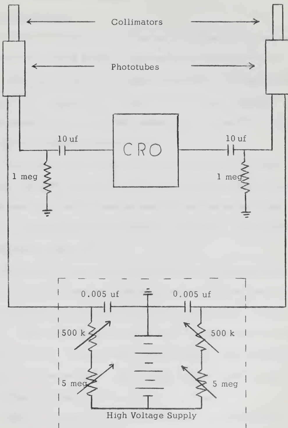
Fig. 7. Photomultiplier Circuitry
