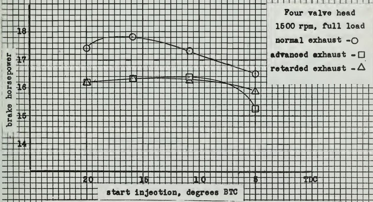
Fig. 33. Brake horsepower versus injection point for various exhaust timings.
