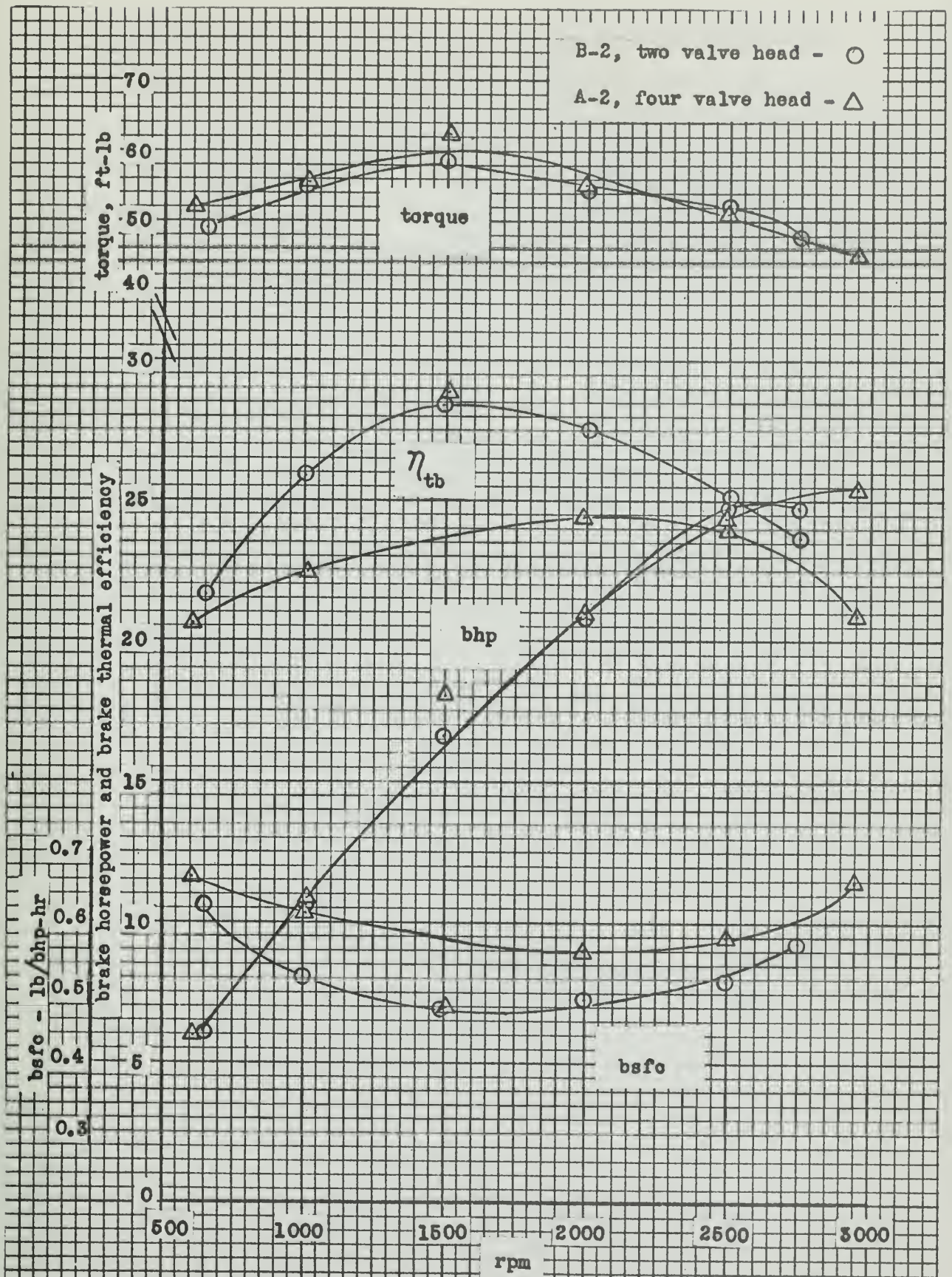
Fig. 30. Performance curves of A-2, B-2; Full load.
