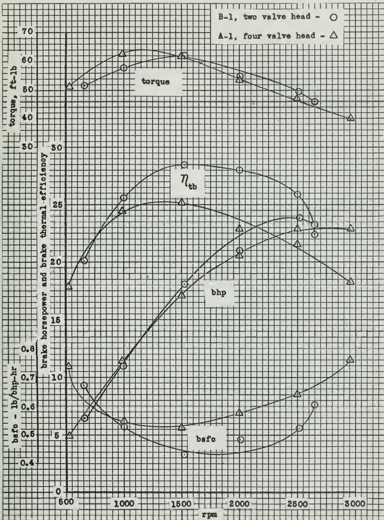
Fig. 29. Performance curves of A-1, B-1; full load.
