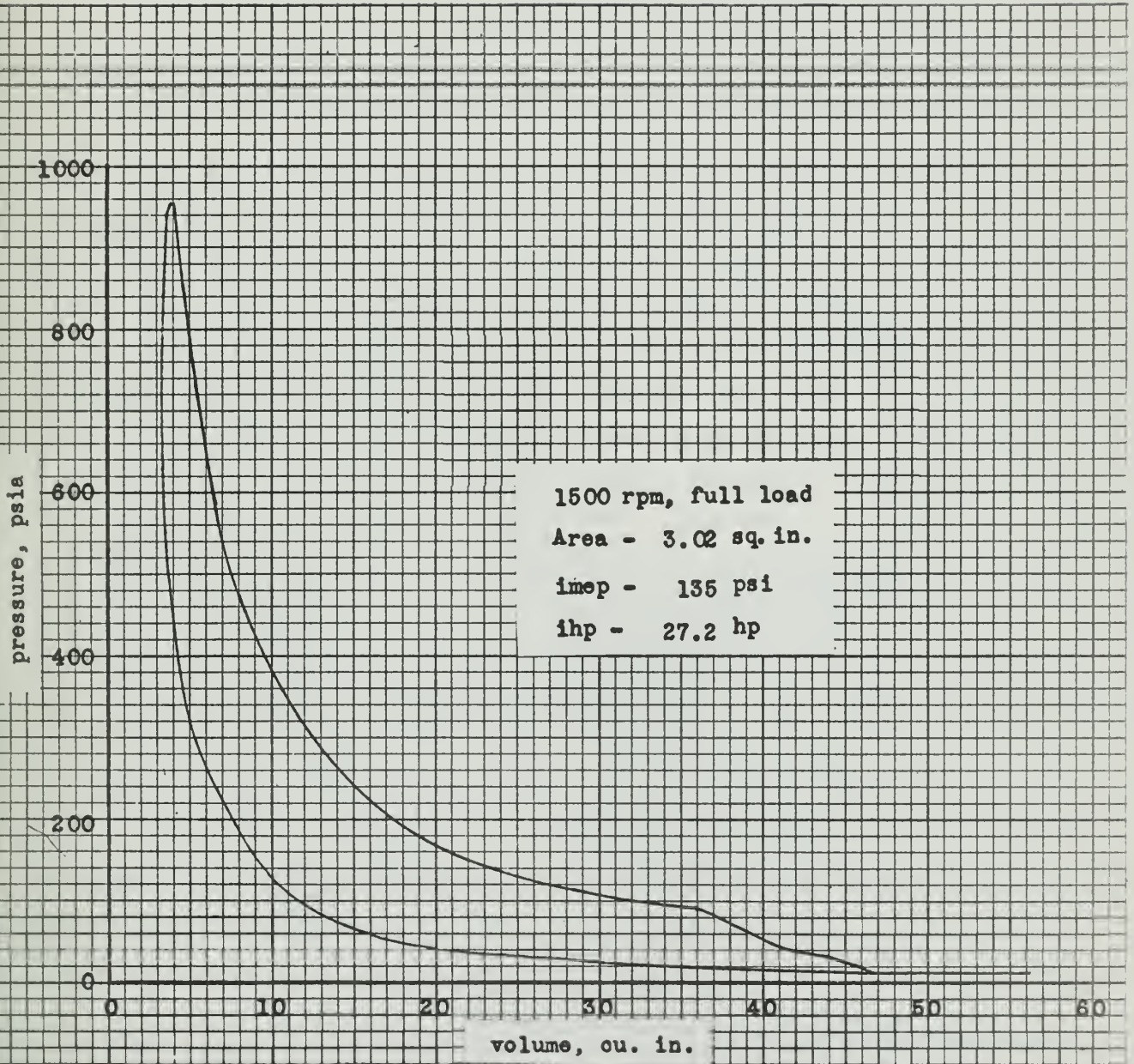
Fig. 40. Pressure-volume diagram, injection at 10.8 °BTC (A-1).
