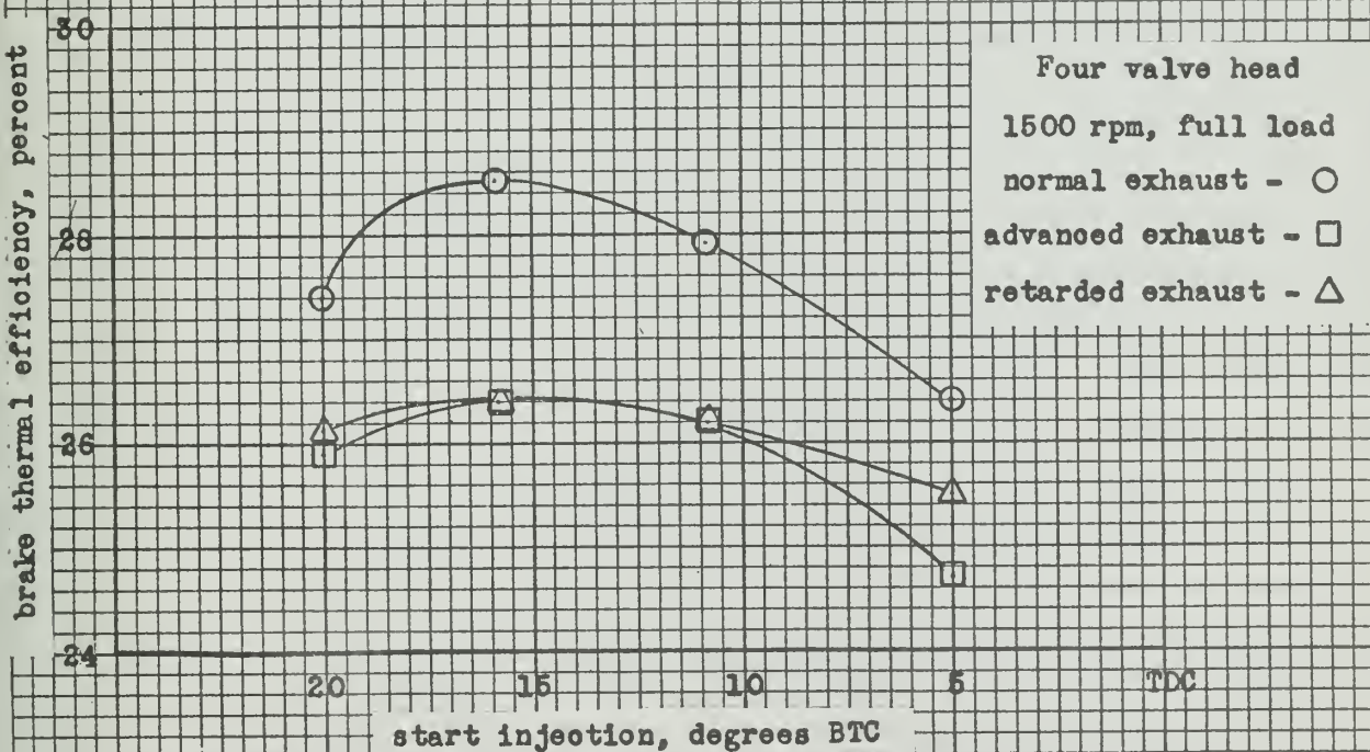
Fig. 37. Brake thermal efficiency versus injection point for various exhaust timings.
