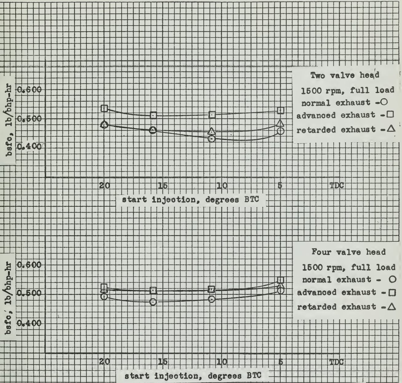
Fig. 36. Brake specific fuel consumption versus fuel injection point for various exhaust timings.
