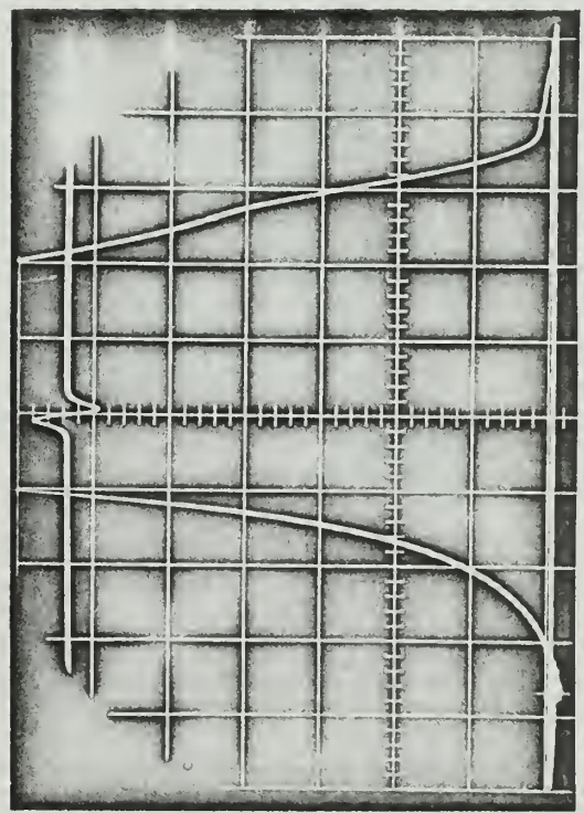
Four valve; exhaust open 097 °ATC, shut 222 °ATC
