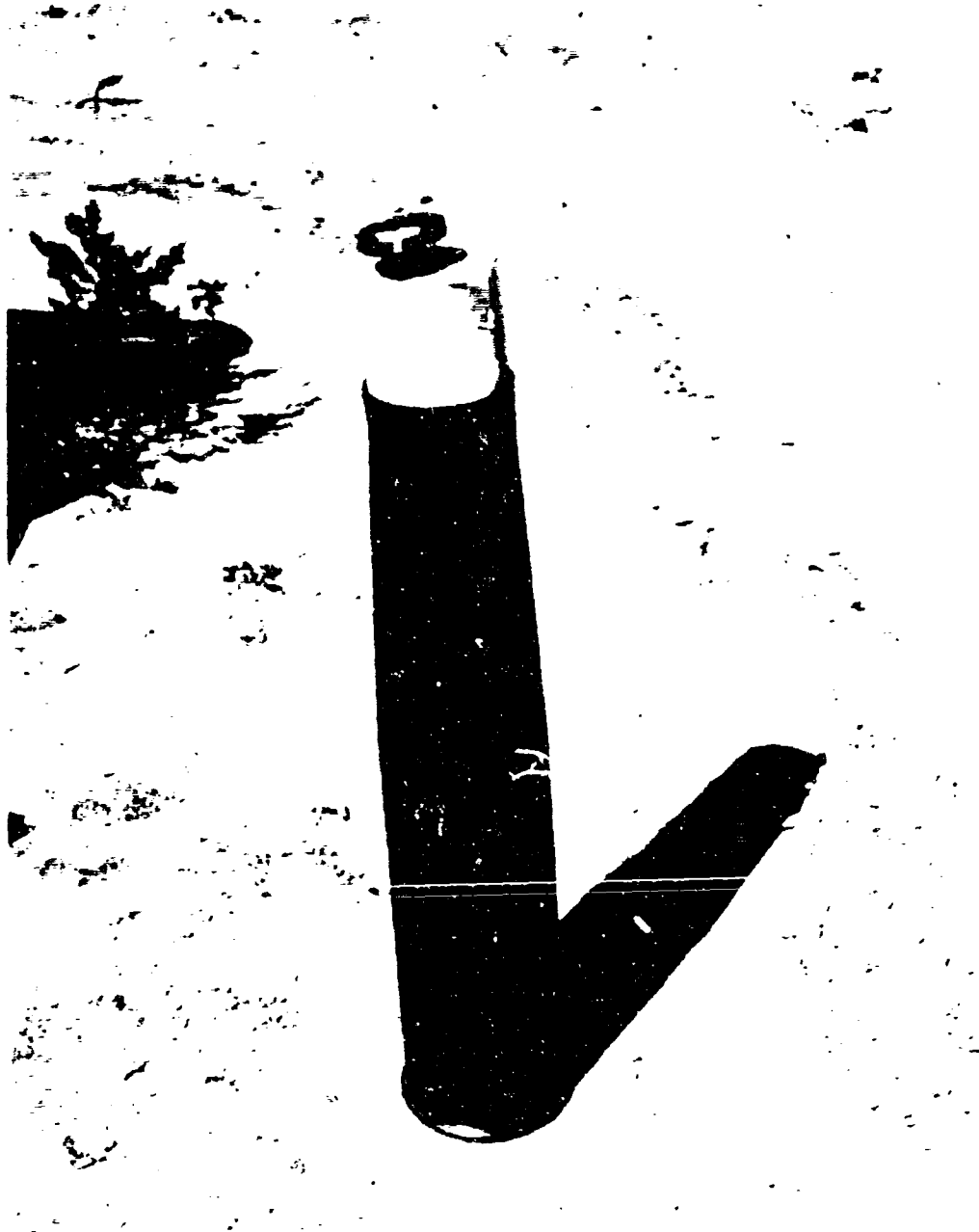
Figure 2 A standard 120 mm cartridge case loaded with a triple-web mixture of M-17 gunpowder and a sheet additive coolant constitute the propellant for the gun-probe vehicle. Powder temperature is monitored with a probe thermometer which is removed immediately prior to loading.
