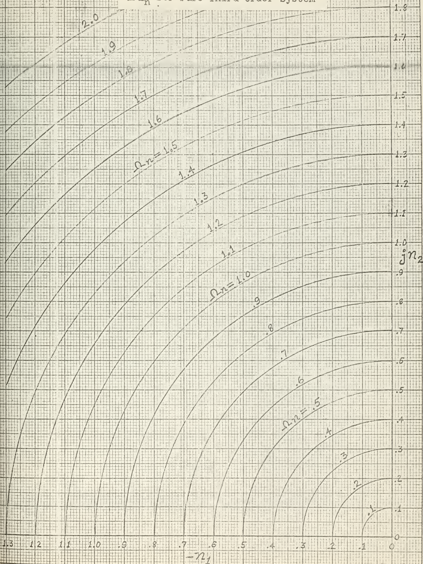
Fig. 5-8 \Omega_n for Pure Third Order System
