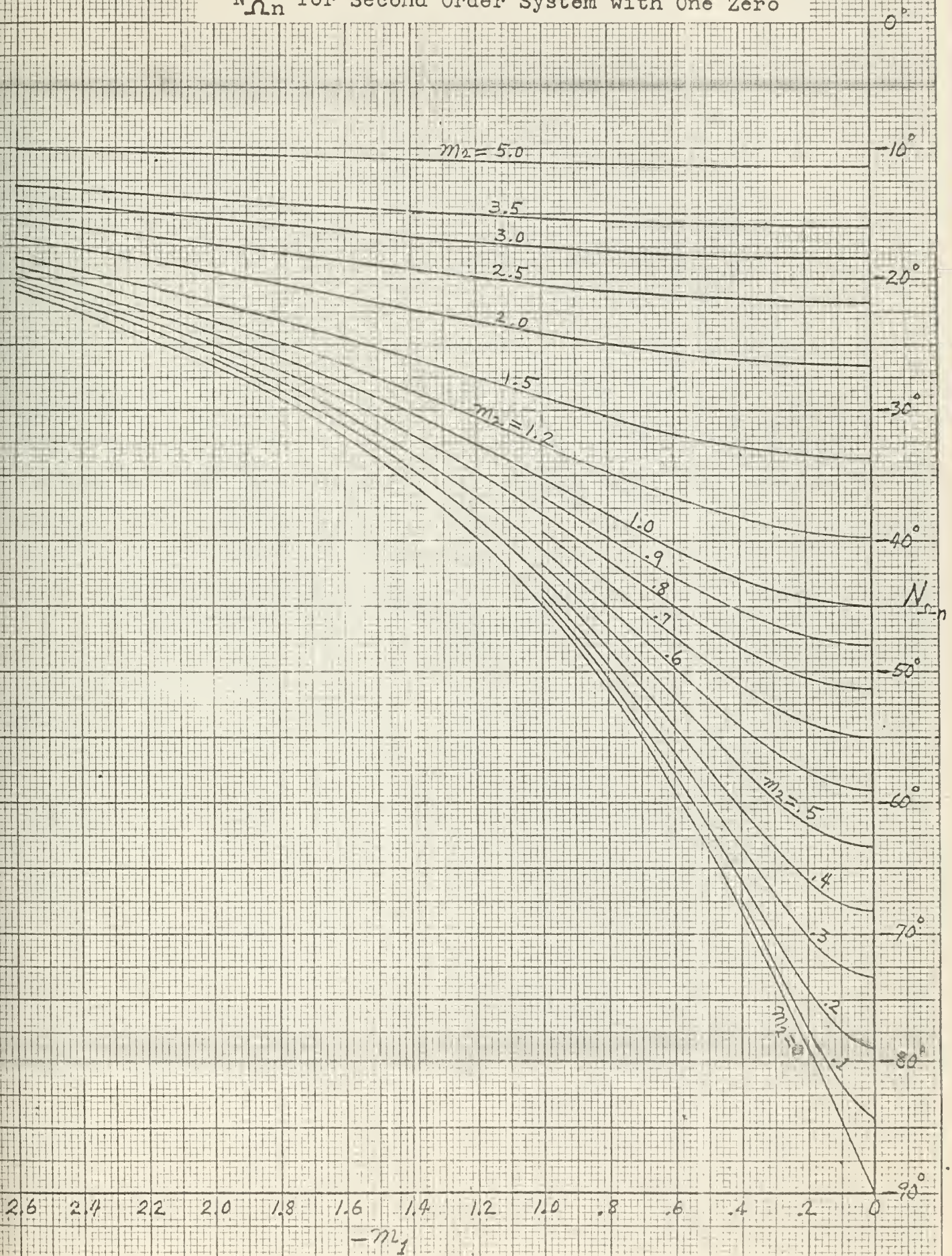
Fig. 4-16 N_{\Omega n} for Second Order System with One Zero
