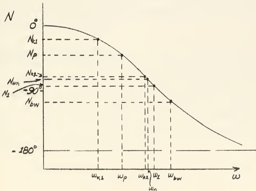
Fig. 2-1 General M and N Contours Showing Parameters Chosen
