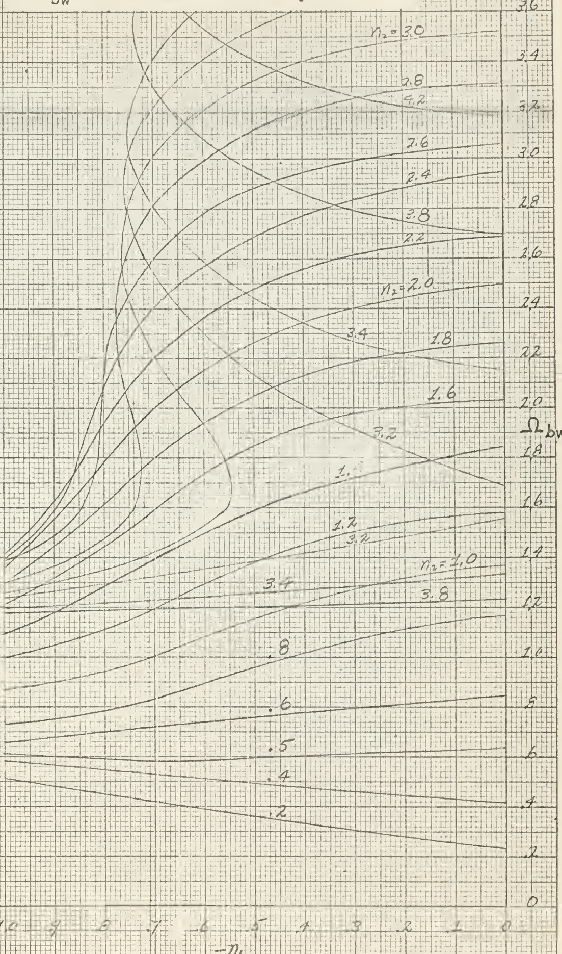
Fig. 5-7 \Omega_{bw} for Pure Third Order System
