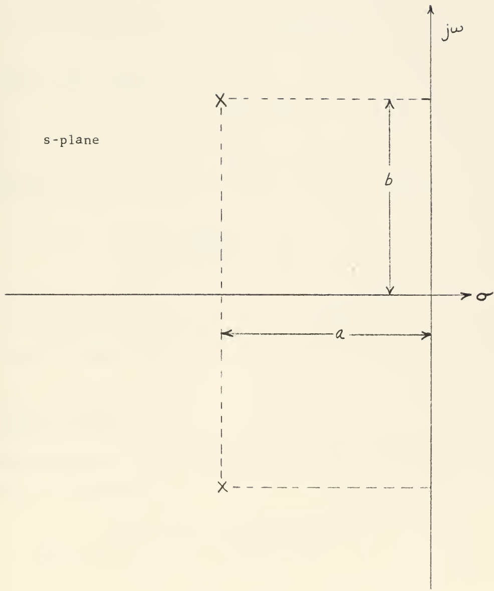
Fig. 3-1 Poles of the Pure Second Order System (s-plane)
