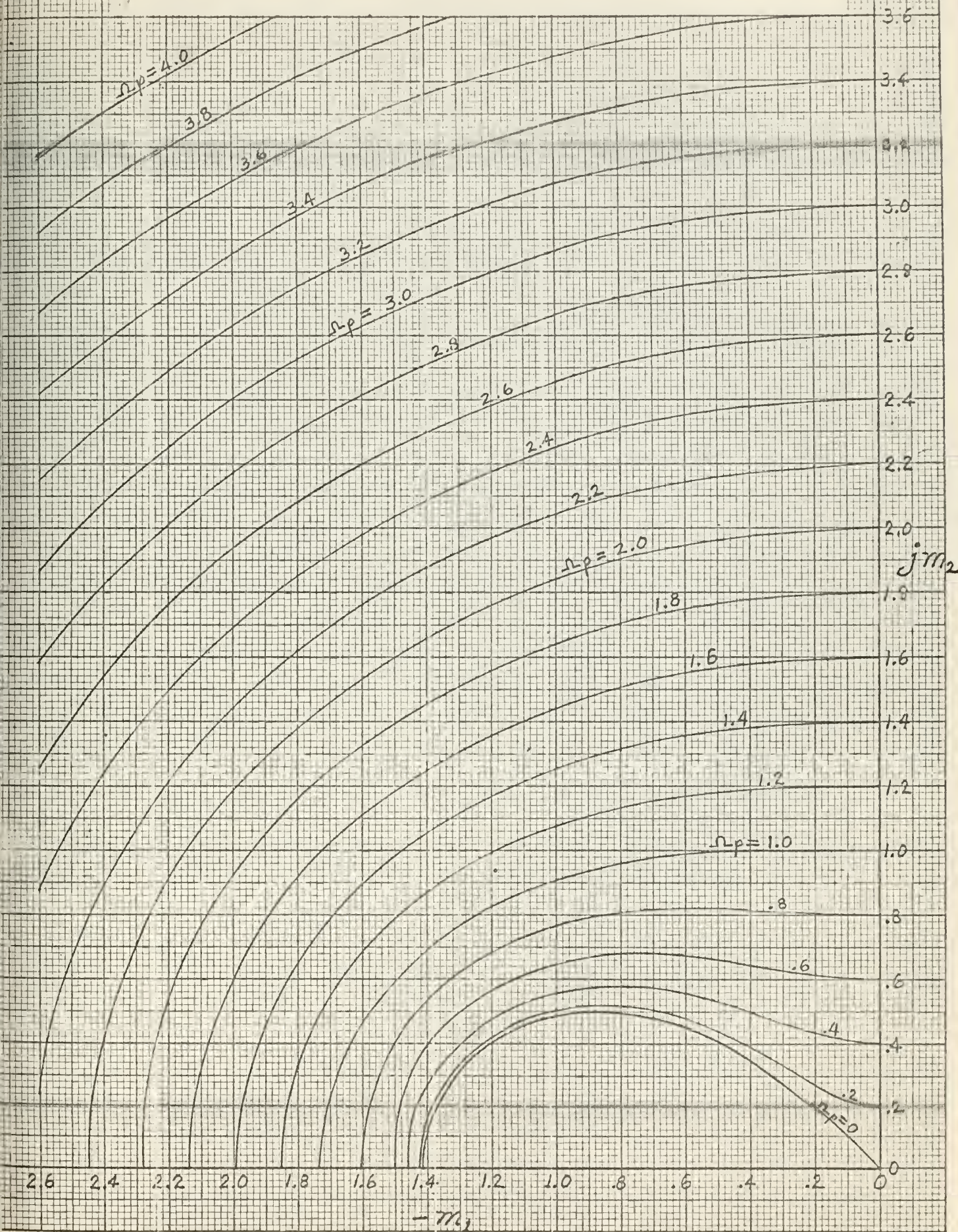
Fig. 4-4. \Omega_p for Second Order System with One Zero
