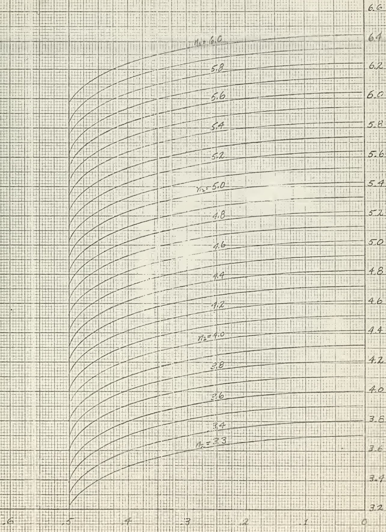
Fig. 5-10b \Omega_1 for Pure Third Order System Extended
