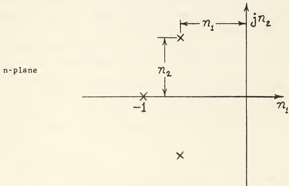
Fig. 5-2 Referred Quantities n_1 and n_2 , Pure Third Order System
