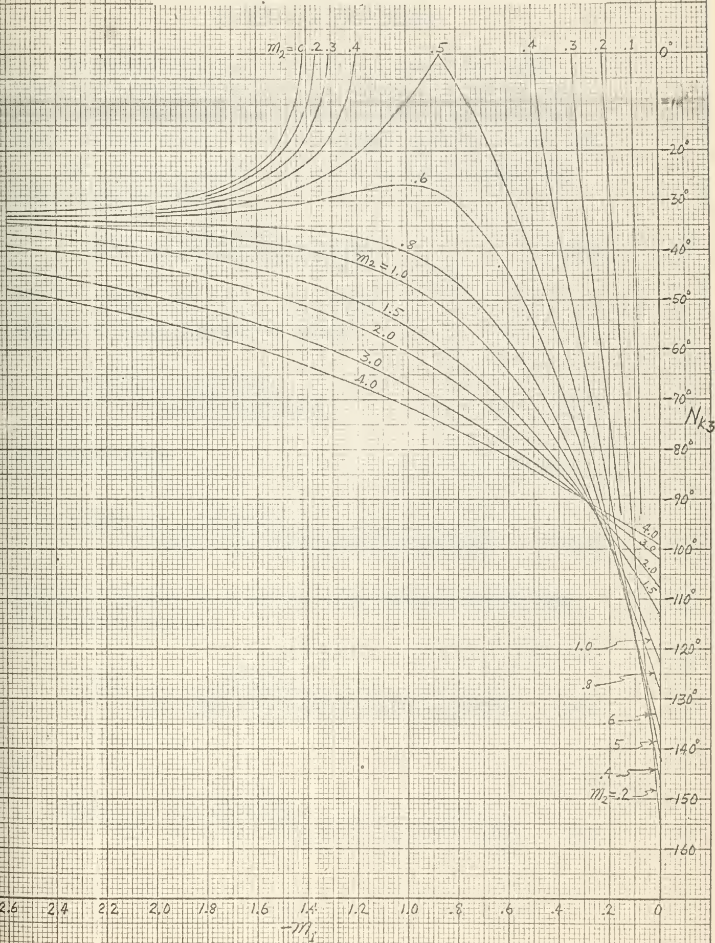
Fig. 4-20 N_{k3} for Second Order System with One Zero
