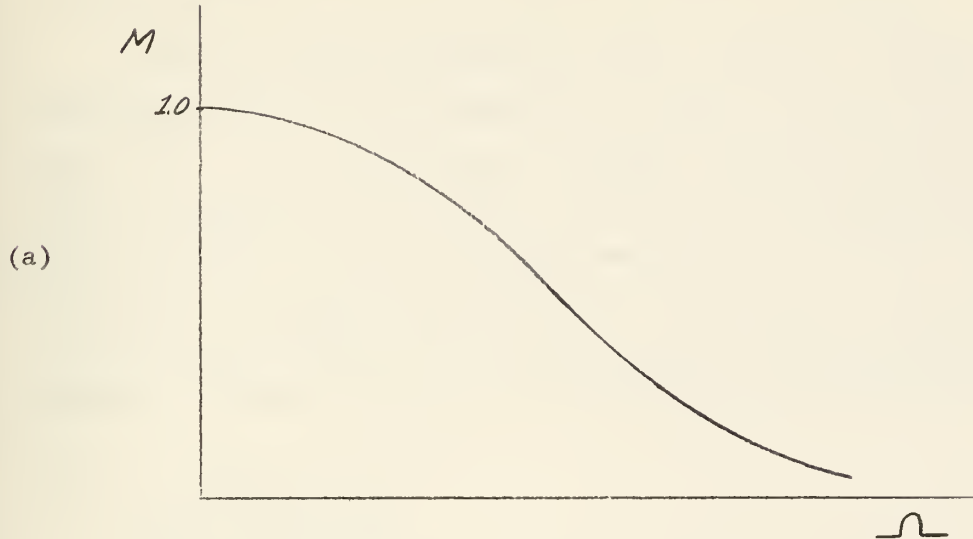
Fig. 5-3 The Three Basic M Curve Shapes for Pure Third Order System
