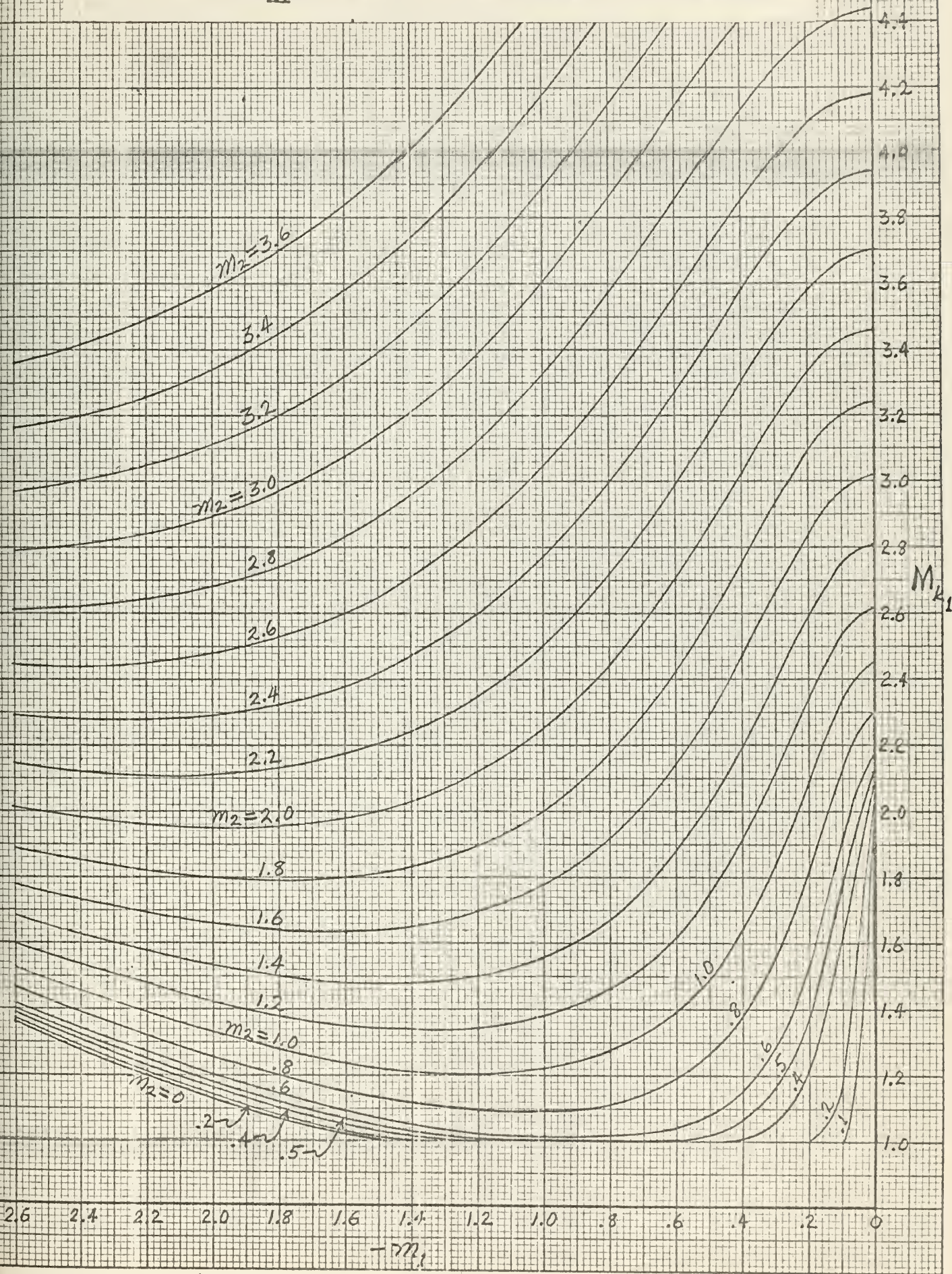
Fig. 4-11. M_{K1} for Second Order System with One Zero
