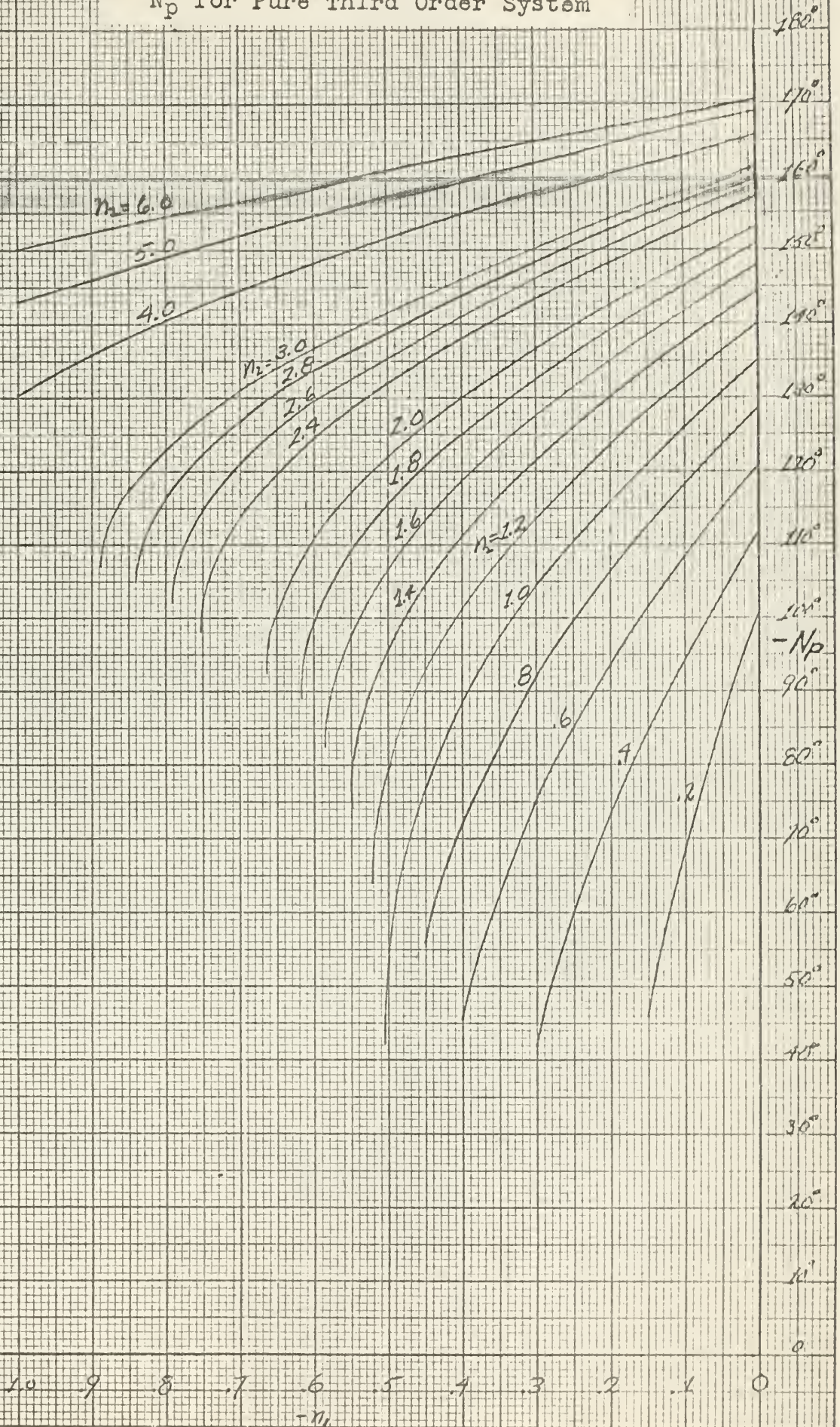
Fig. 5-15a N_p for Pure Third Order System
