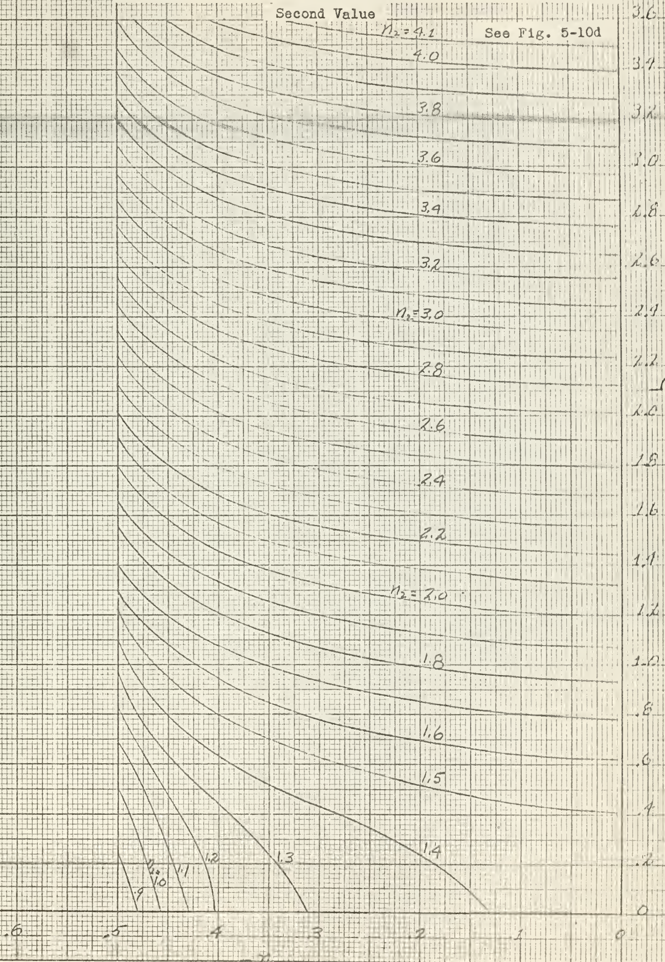
Fig. 5-10c. \Omega_1 for Pure Third Order System
