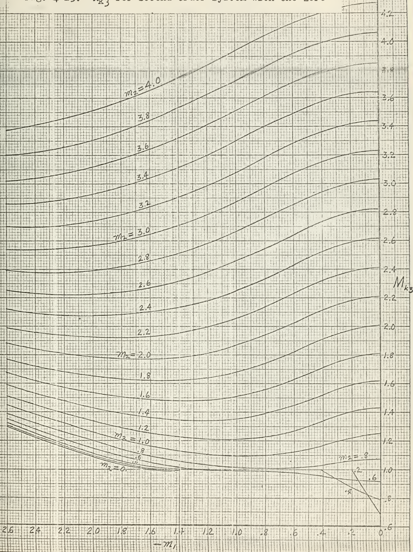
Fig. 4-13. M_{k3} for Second Order System with One Zero
