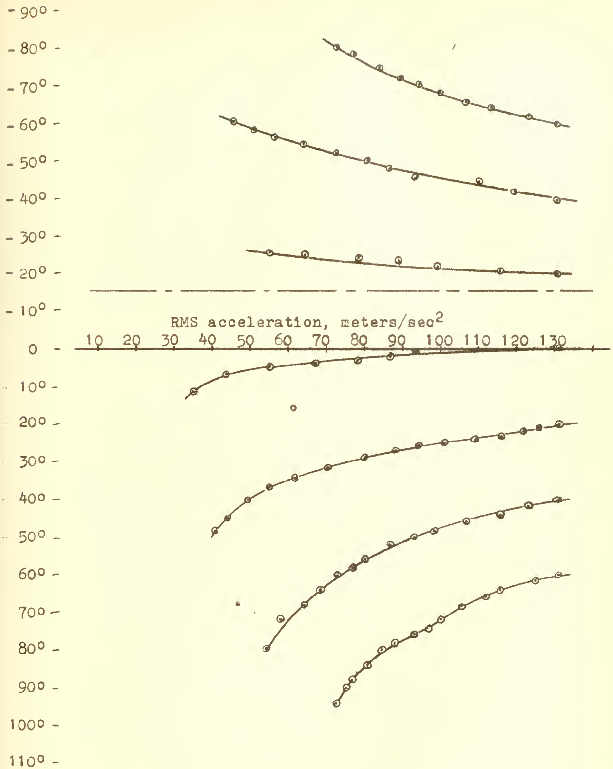
Figure 12. Variation of \Delta as A is reduced. f_1 = 200 cps.
