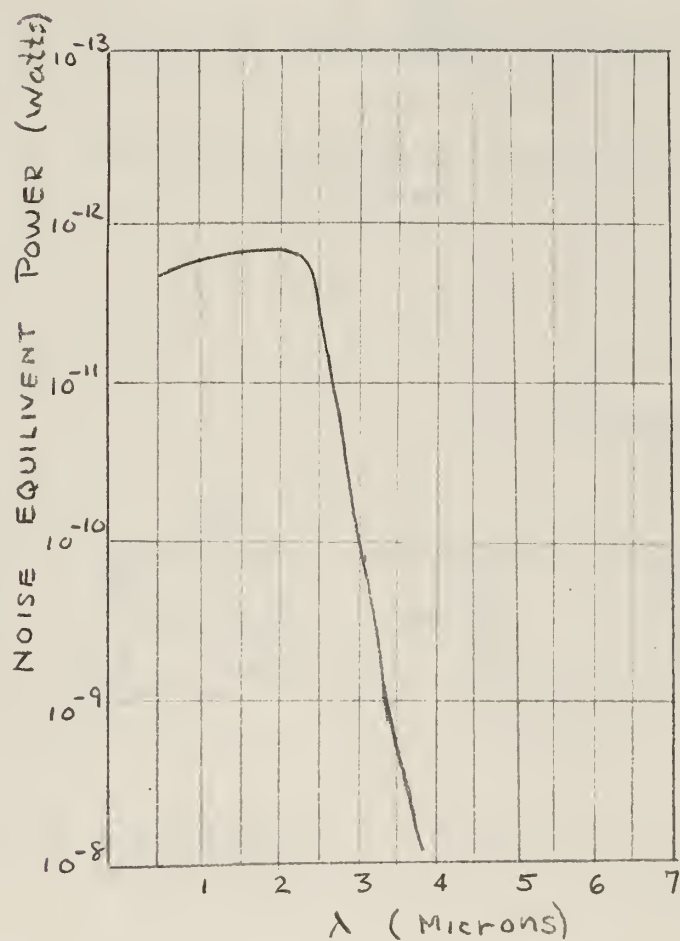
Fig. 2-3 Optimum NEP vs. Wavelength for PbS Detector at 25°C
