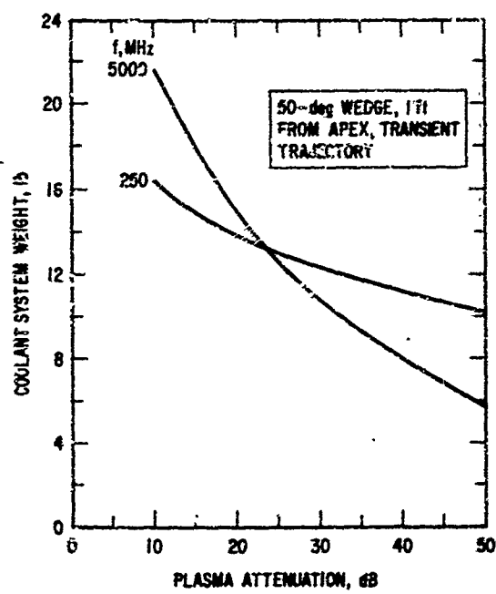
Fig. 38. Coolant System Theoretical Weight at Two Signal Frequencies
