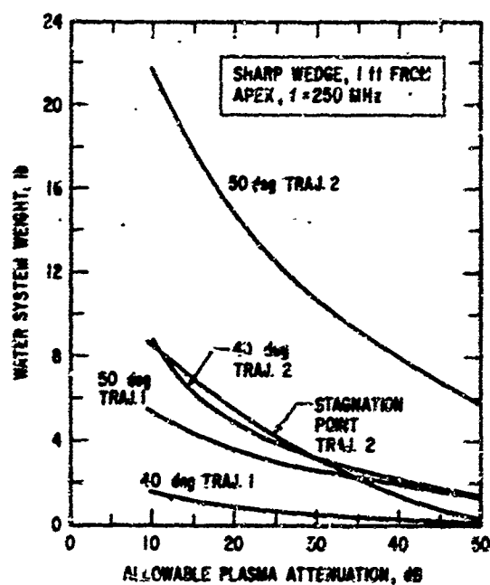
Fig. 36. Coolant System Theoretical Weight Requirements
