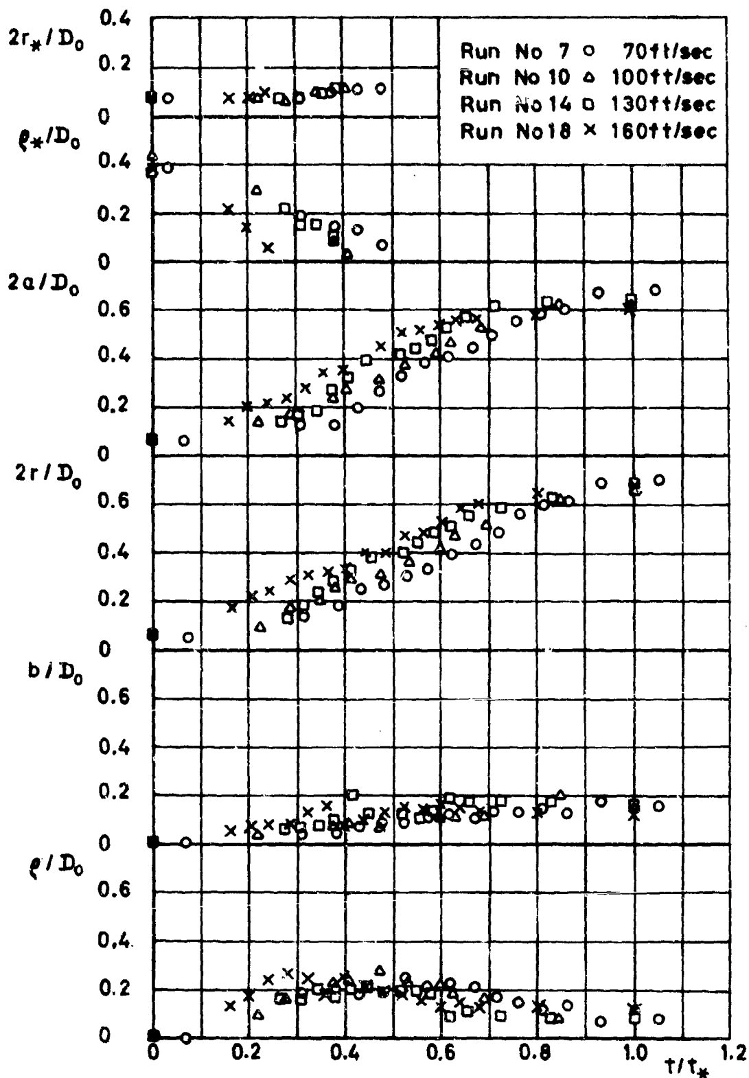
Figure 83 Parameters of Idealized Photographic Shape Versus Time for Ringslot
