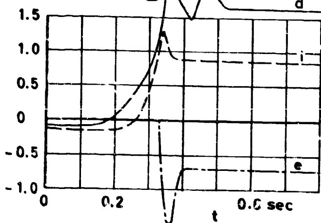
Figure 95 c_p versus time for differential, internal and external pressure
