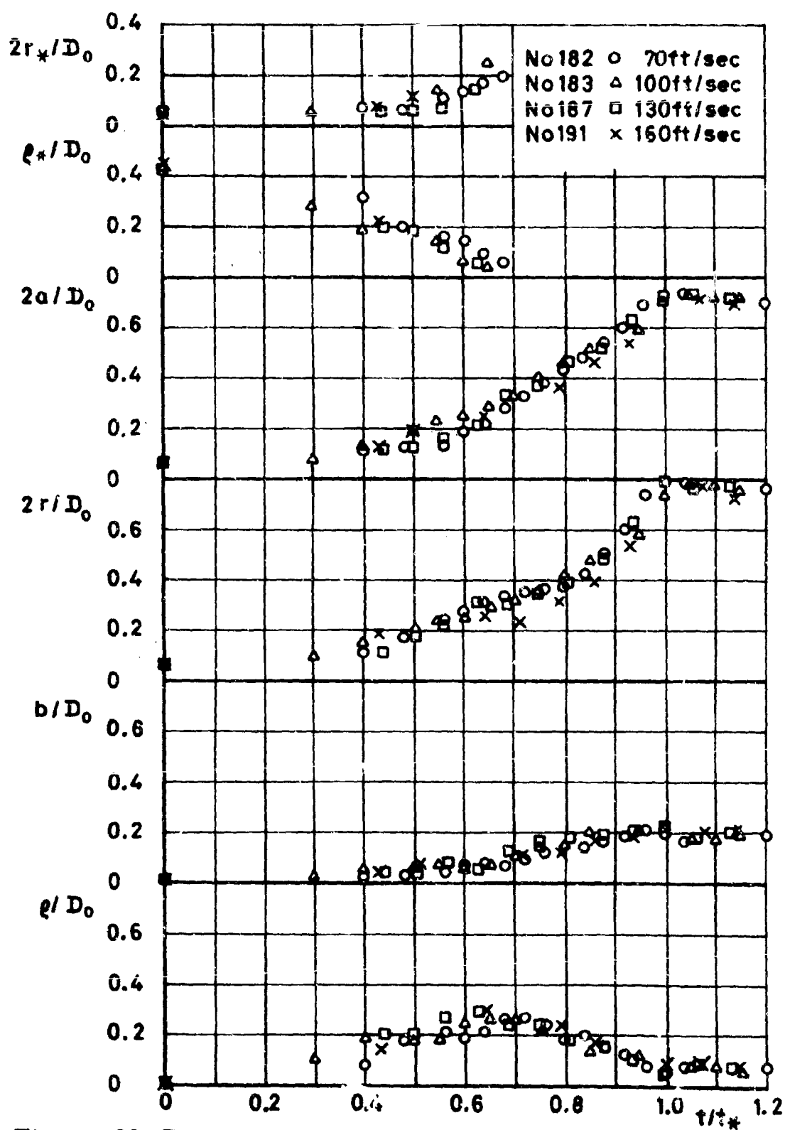
Figure 80 Parameters of Idealized Photographic Shape Versus Time for Circular Flat
