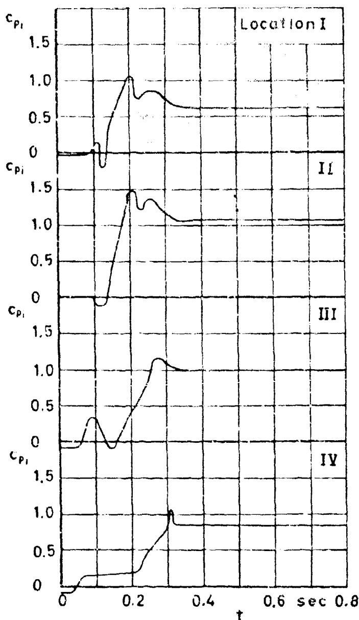
Figure 45 c_{pi} and filling versus time v_0 = 100 ft/sec Run N: 30
