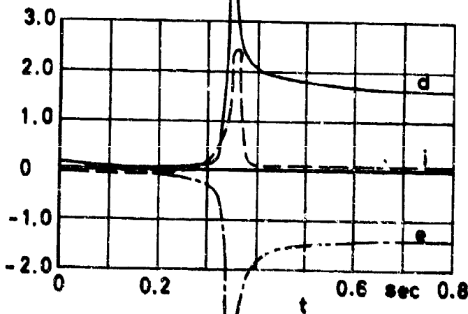
No. 221 p_e external pressure
