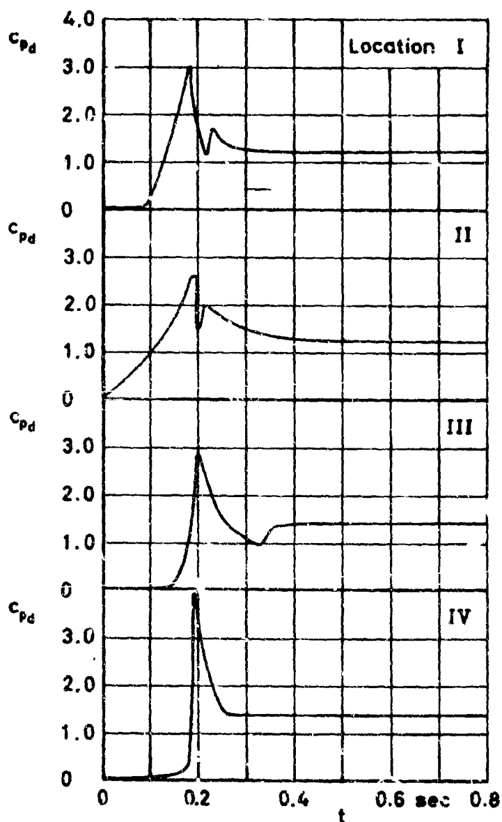
Figure 26 c_{pD} and filling versus time
