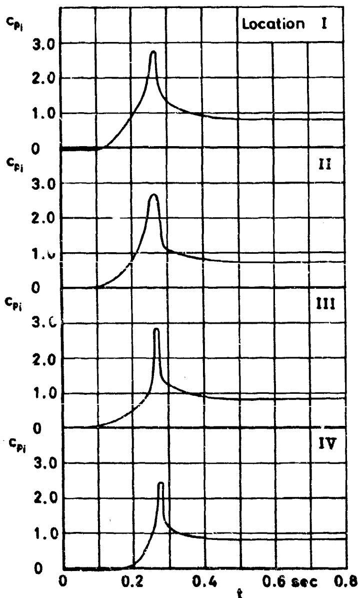
Figure 21 c_{pi} and filling versus time v_0 = 100 ft/sec Run No.160
