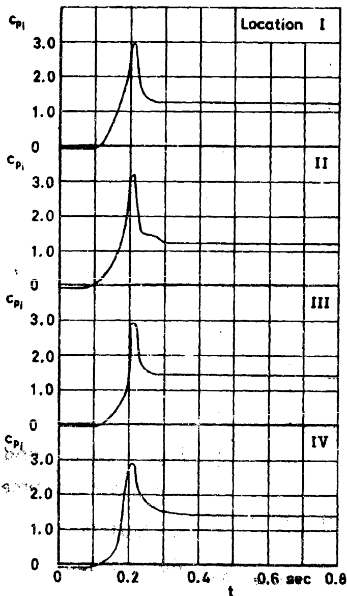
Figure 27 c_{pi} and filling versus time v_0 = 160 \text{ ft/sec} Run No 166
