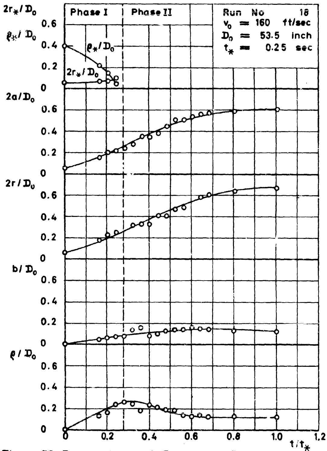
Figure 79 Parameters of Idealized Photographic Shape Versus Time for Ringslot
