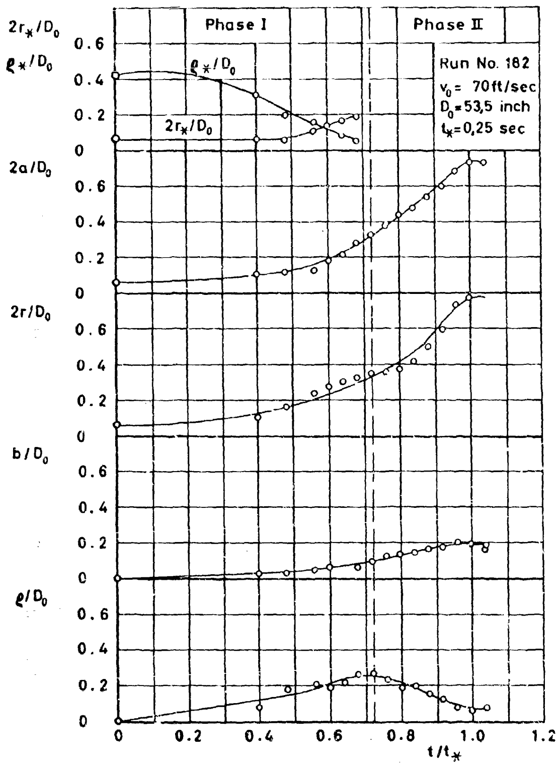
Figure 64 Parameters of Idealized Photographic Shape Versus Time for Circular Flat
