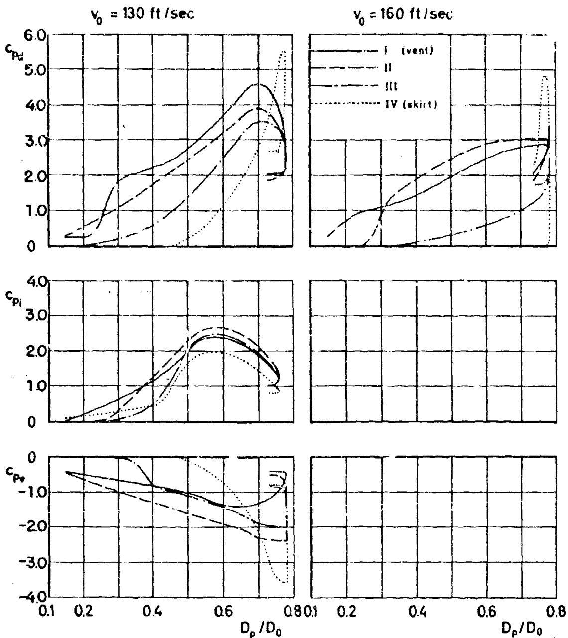
Figure 54 c_p versus D_p/D_0 for Circular Flat
