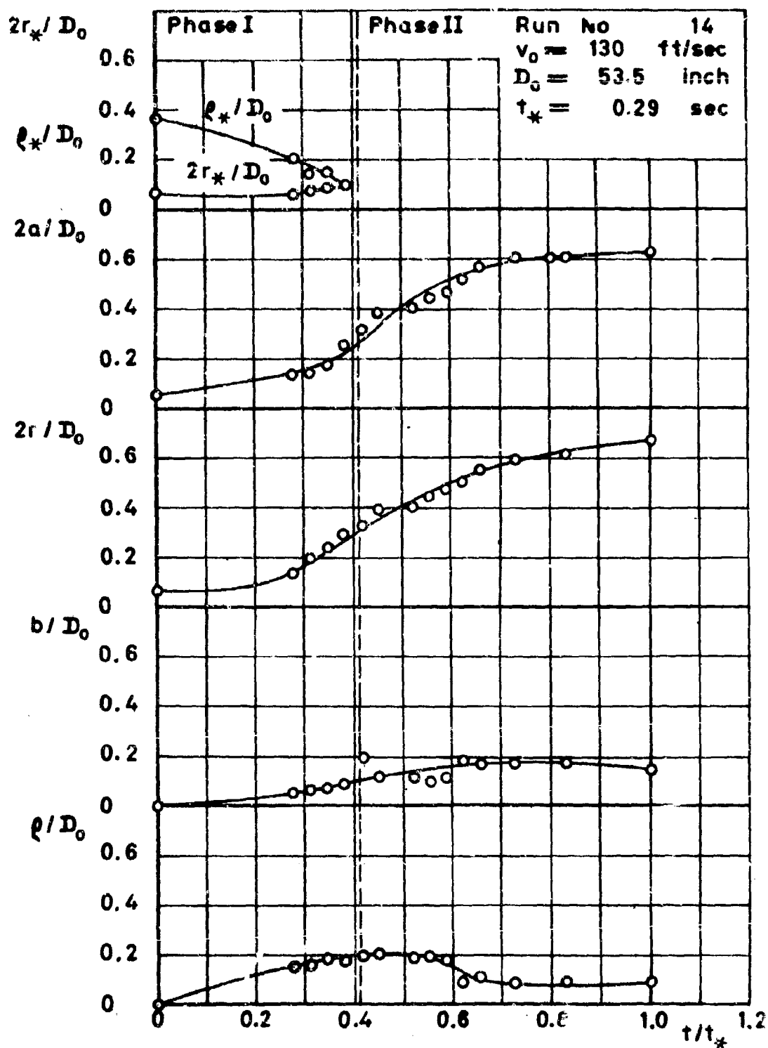
Figure 78 Parameters of Idealized Photographic Shape Versus Time for Ringslot
