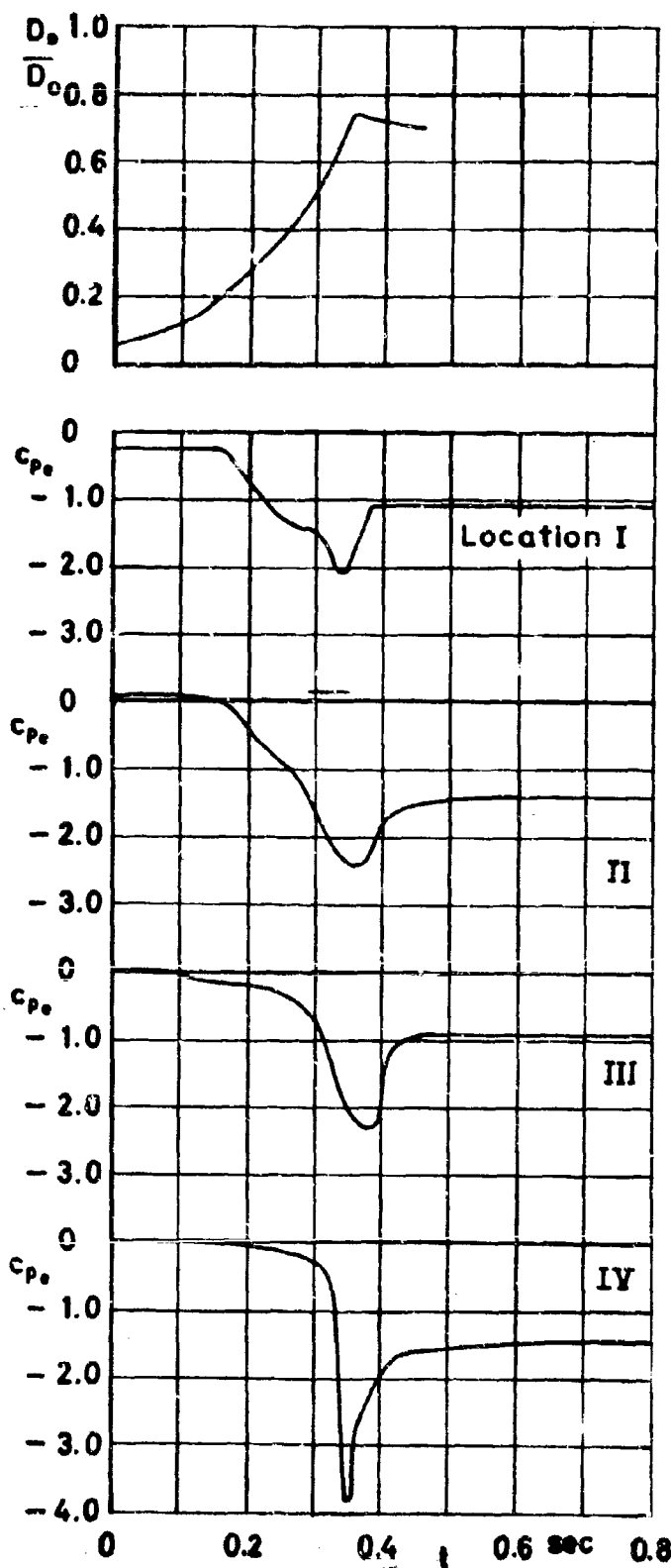
Figure 19 c_p and filling versus time v_0 = 70 ft/sec Run No 221
