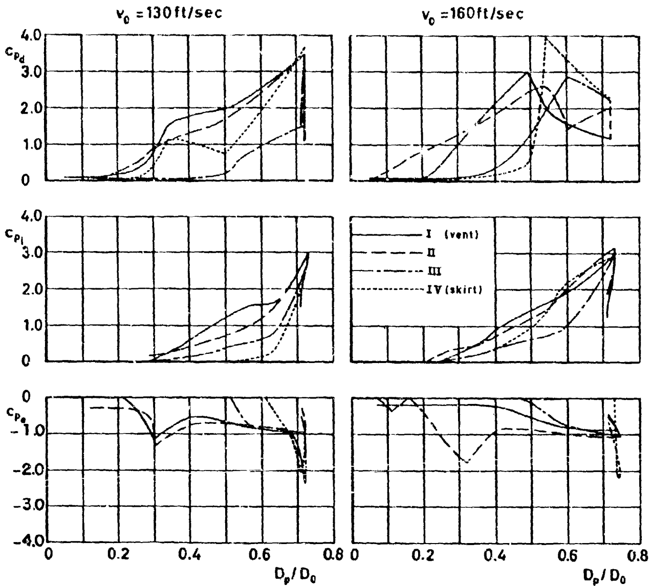
Figure 56 c_p versus D_p/D_0 for Extended Skirt Run No. 148; 163; 231; 153; 166; 235
