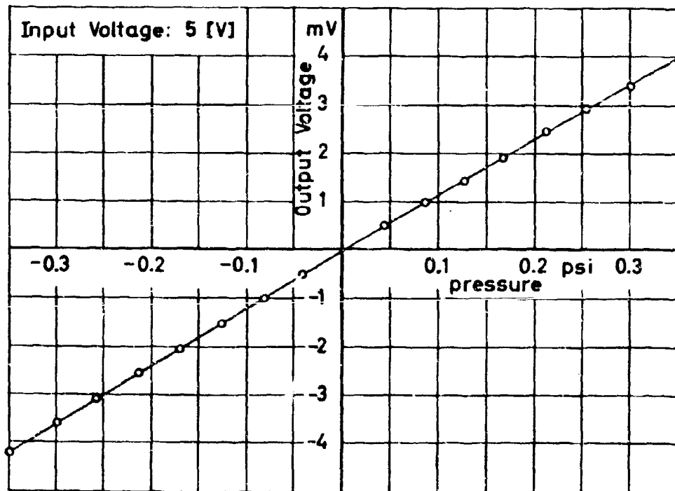
Figure 5 Linearity and Calibration of Pressure Transducer
