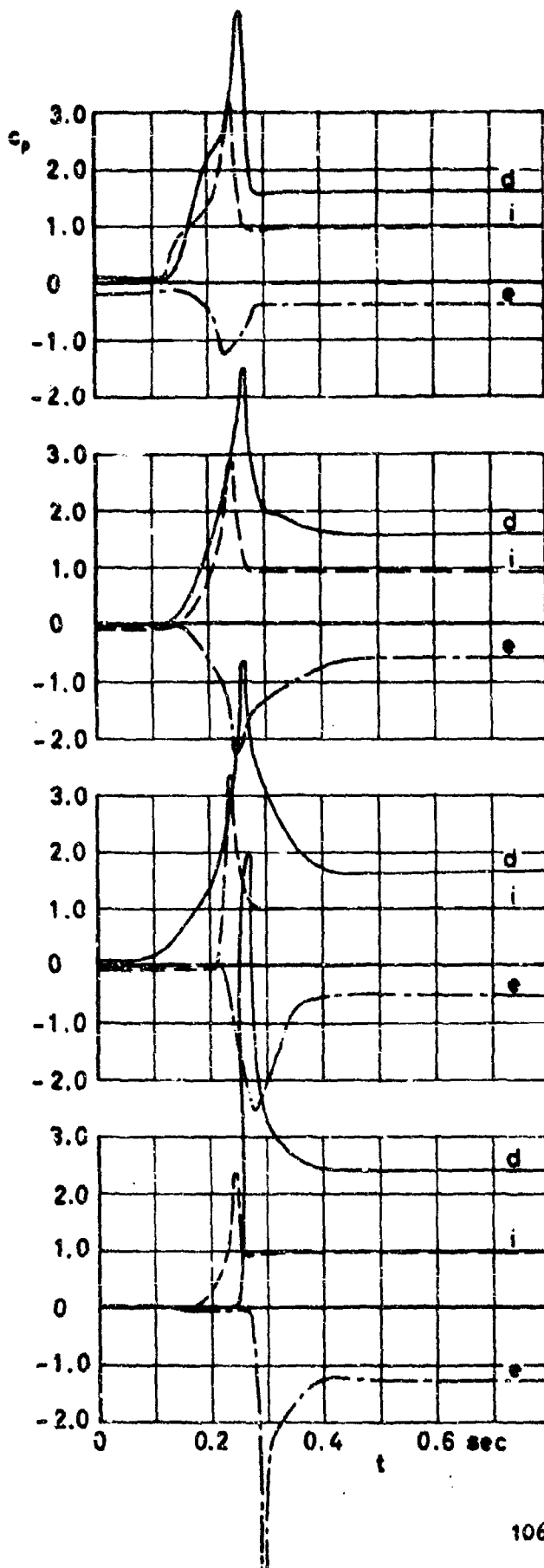
No.182 p_d differential pressure
