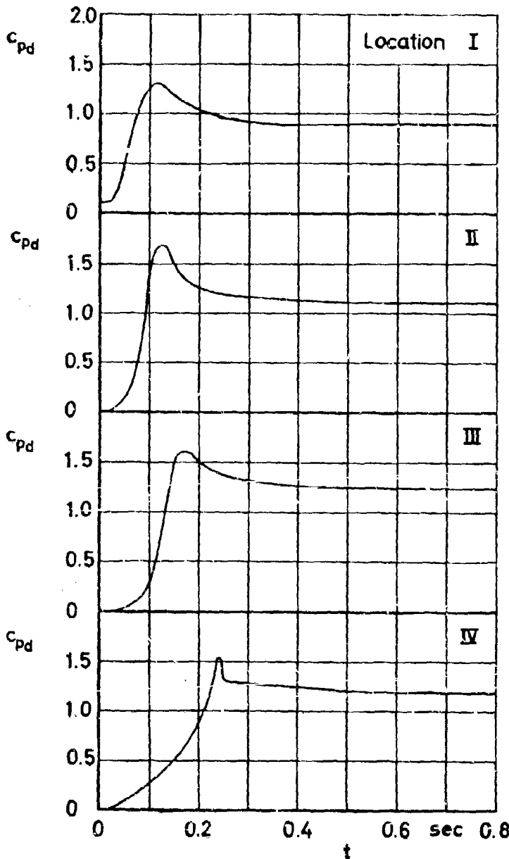
Figure 50 c_{pd} and filling versus time
