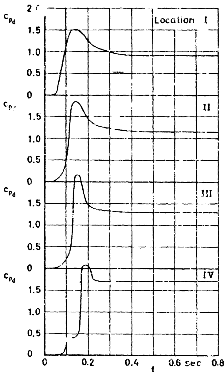
Figure 38 c_{p_d} and filling versus time
