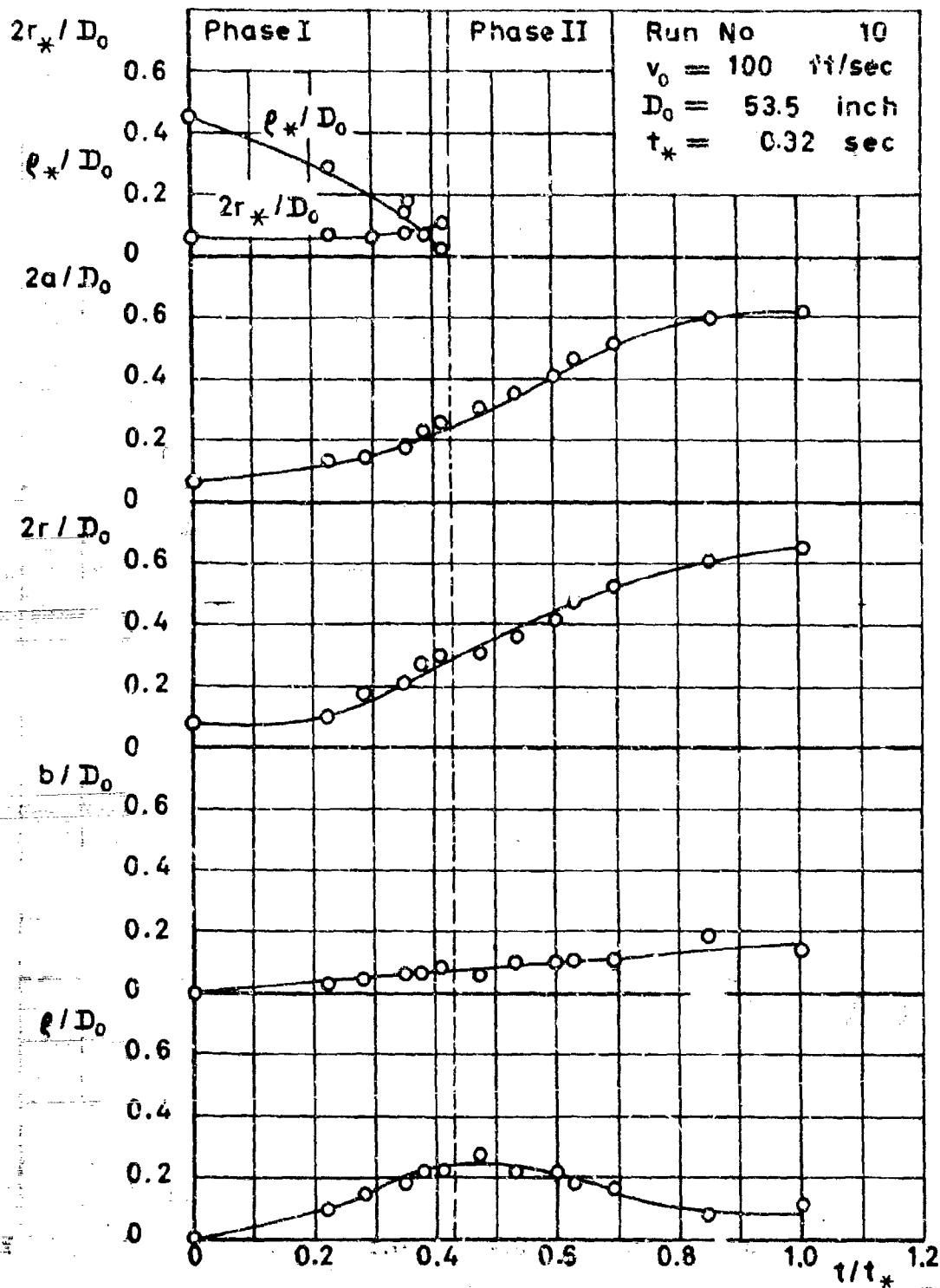
Figure 77 Parameters of Idealized Photographic Shape Versus Time for Ringslot
