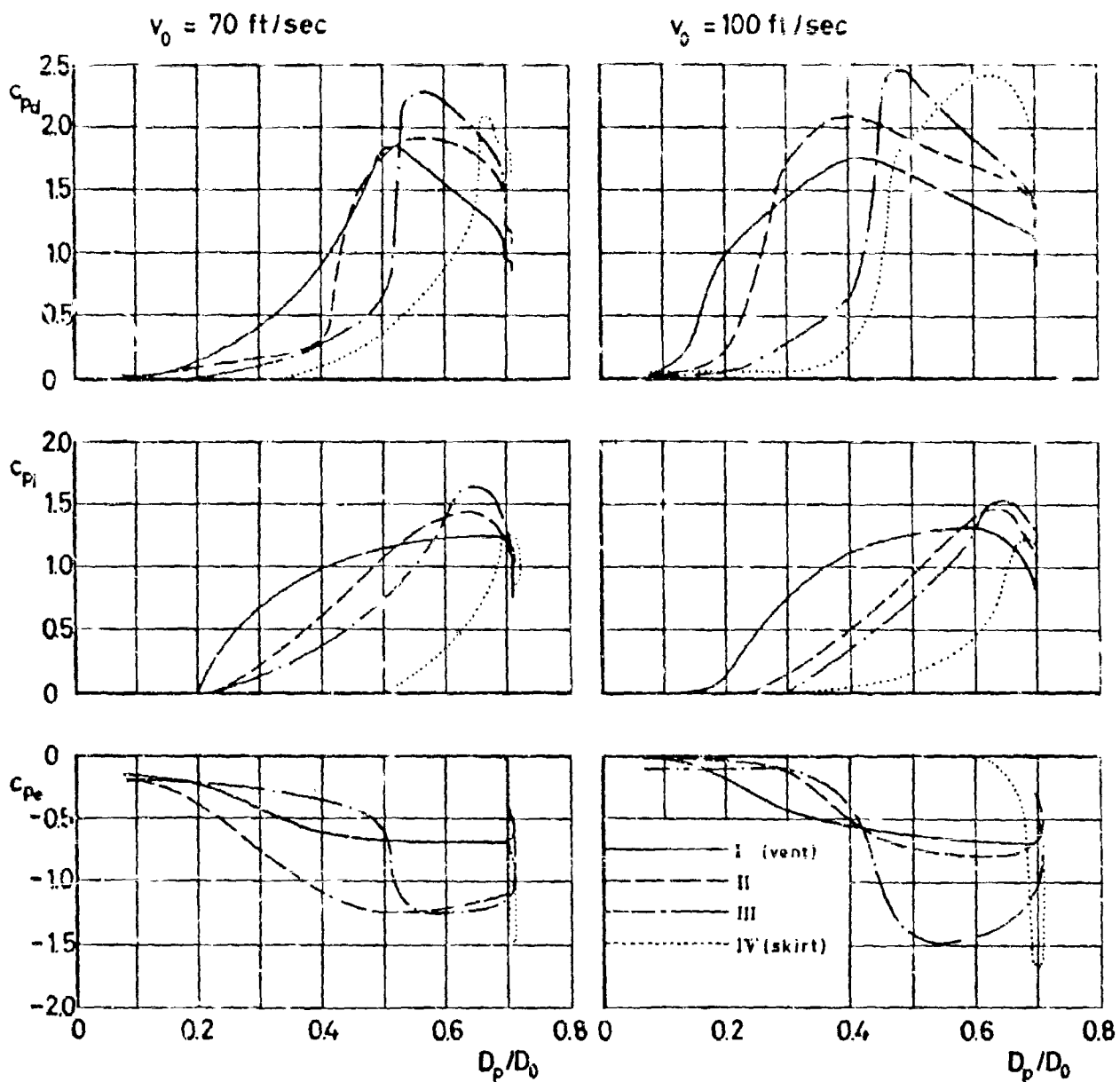
Figure 57 c_p versus D_p/D_0 for FIST
