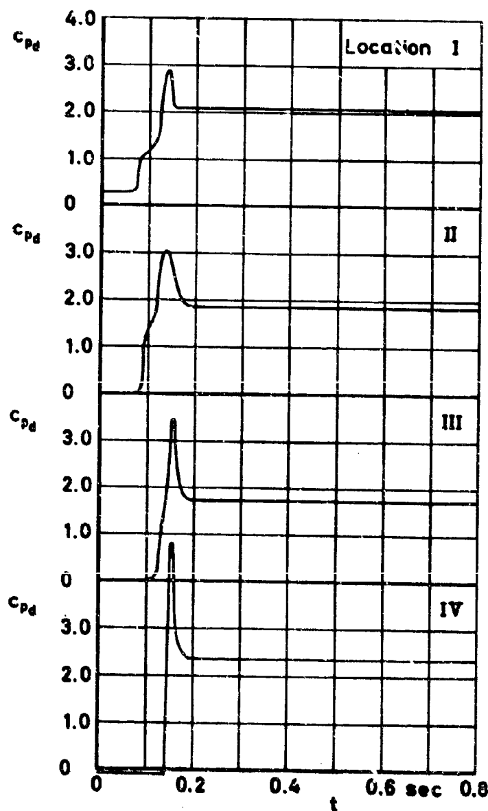
Figure 16 c_{pd} and filling versus time
