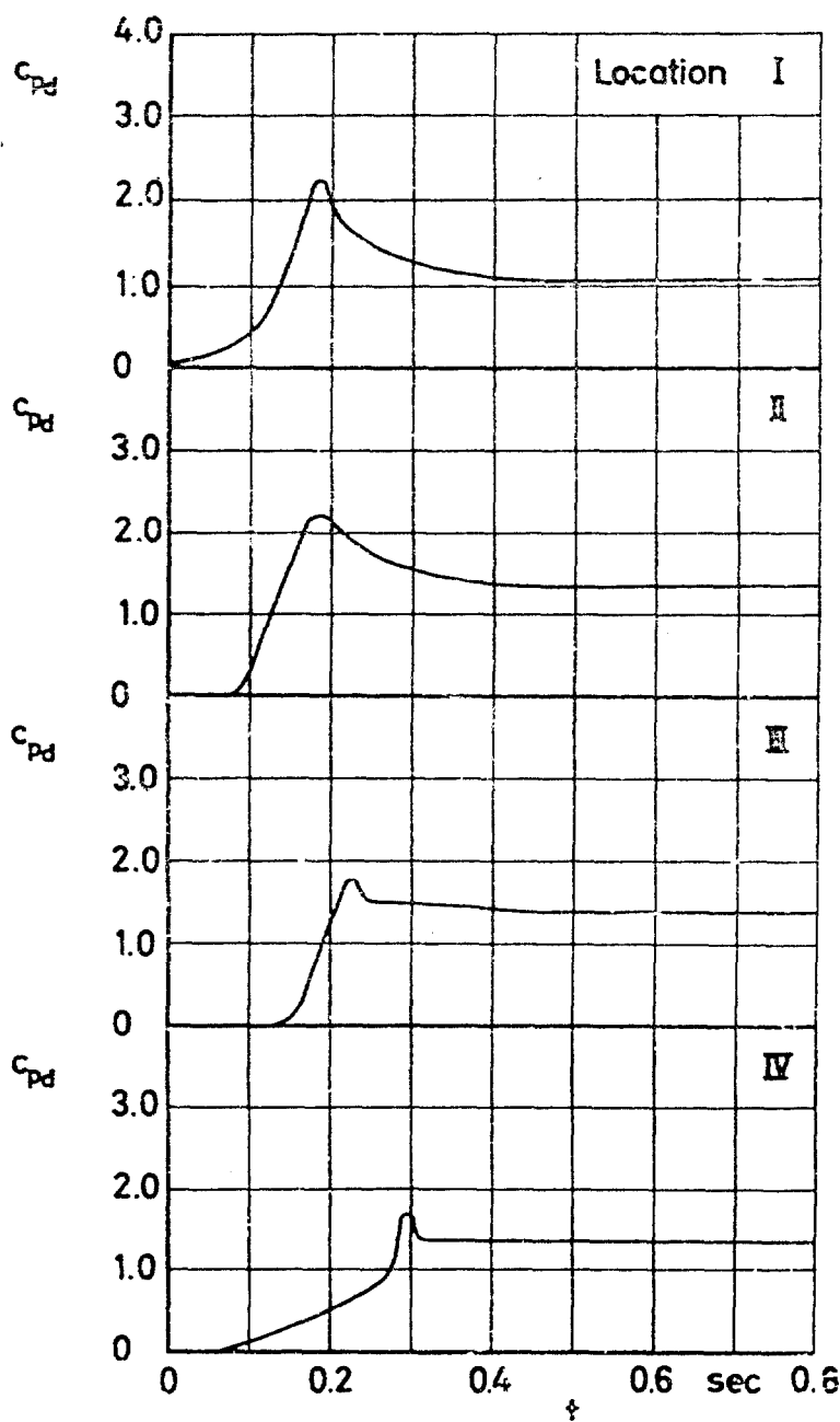
Figure 105 c_{pd} and filling versus time
