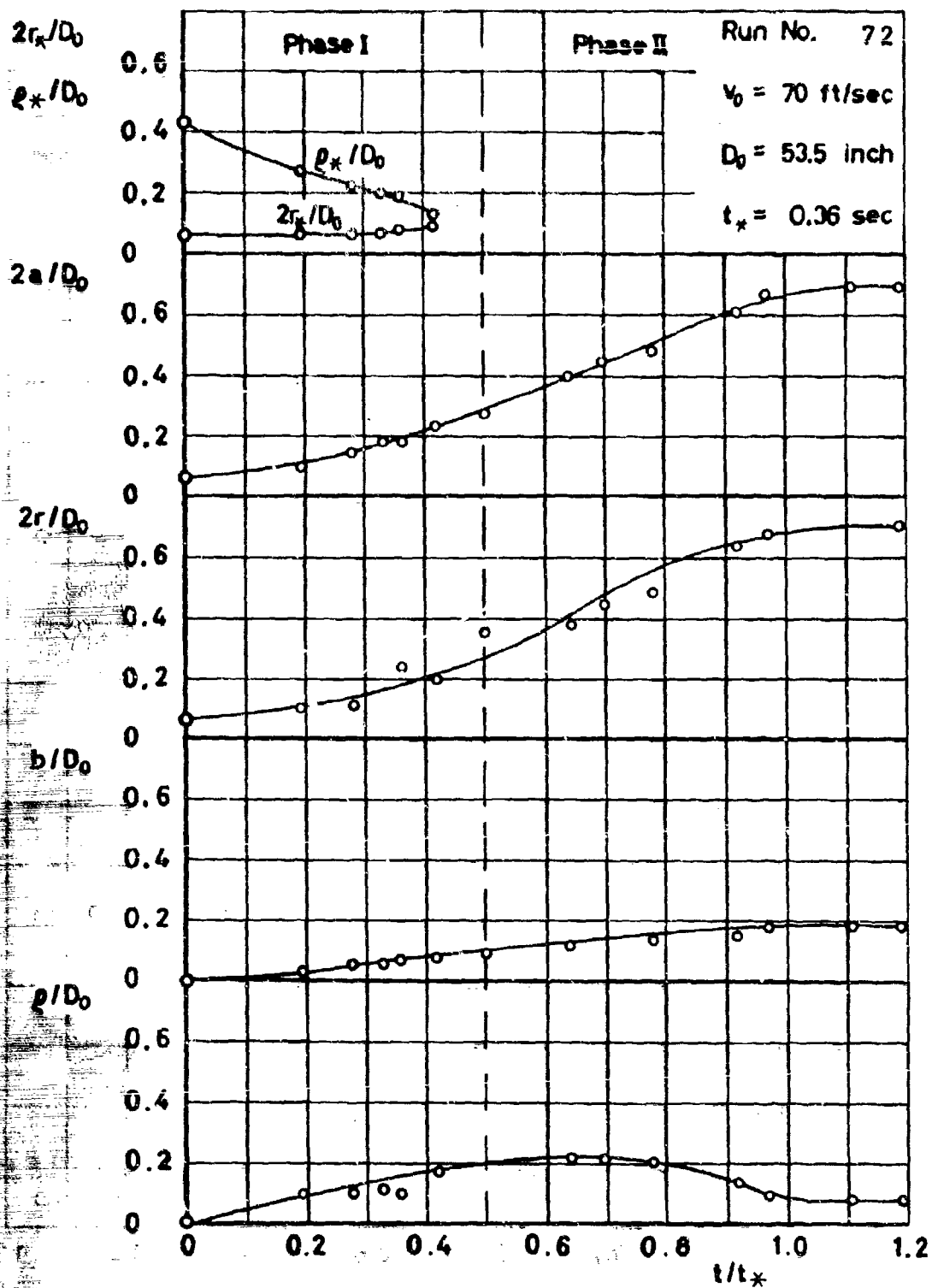
Figure 72 Parameters of Idealized Photographic Shape Versus Time for FIST
