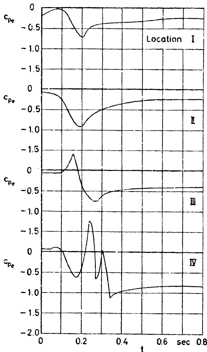
Figure 46 c_{pe} and filling versus time
