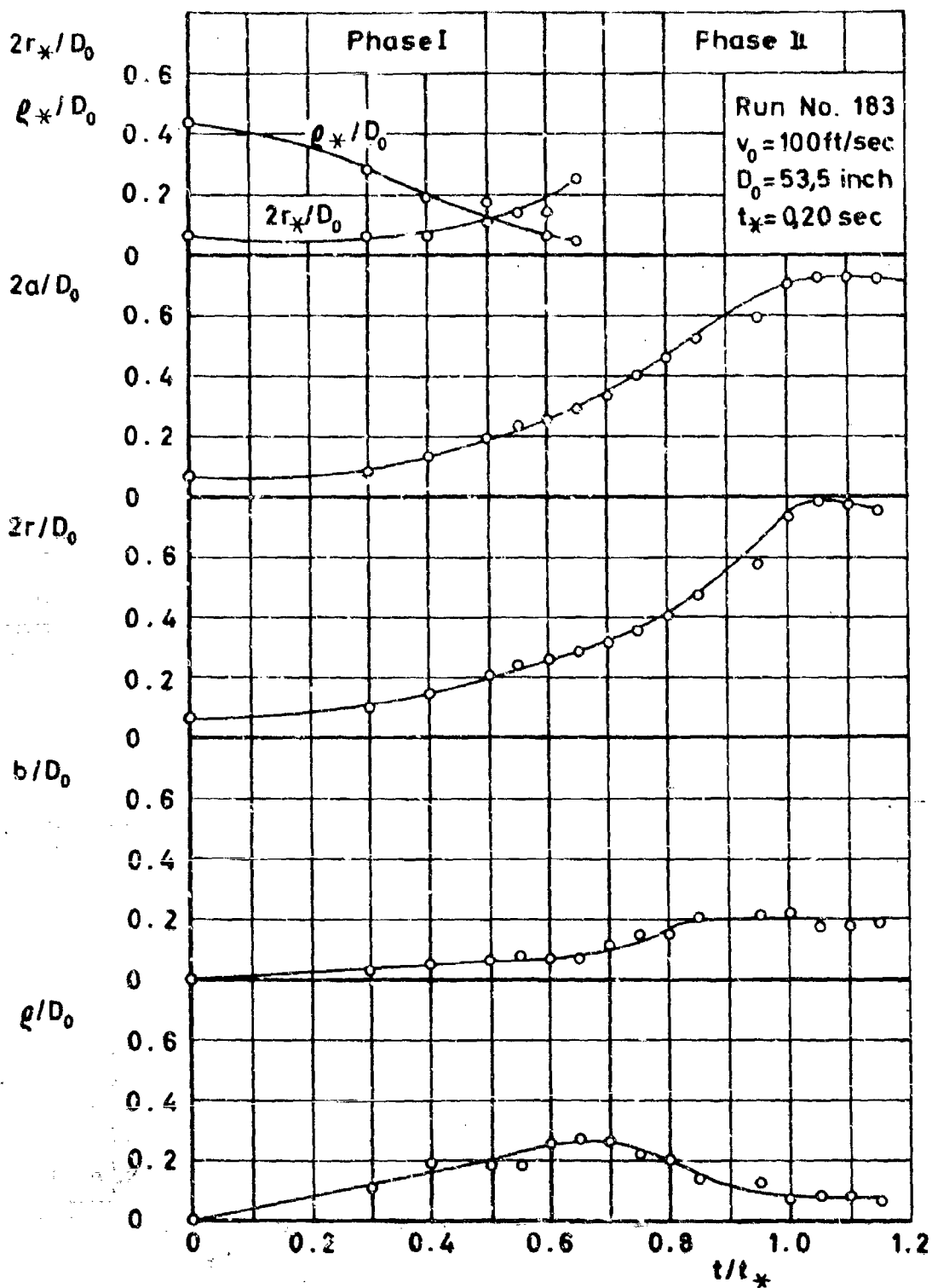
Figure 65 Parameters of Idealized Photographic Shape Versus Time for Circular Flat
