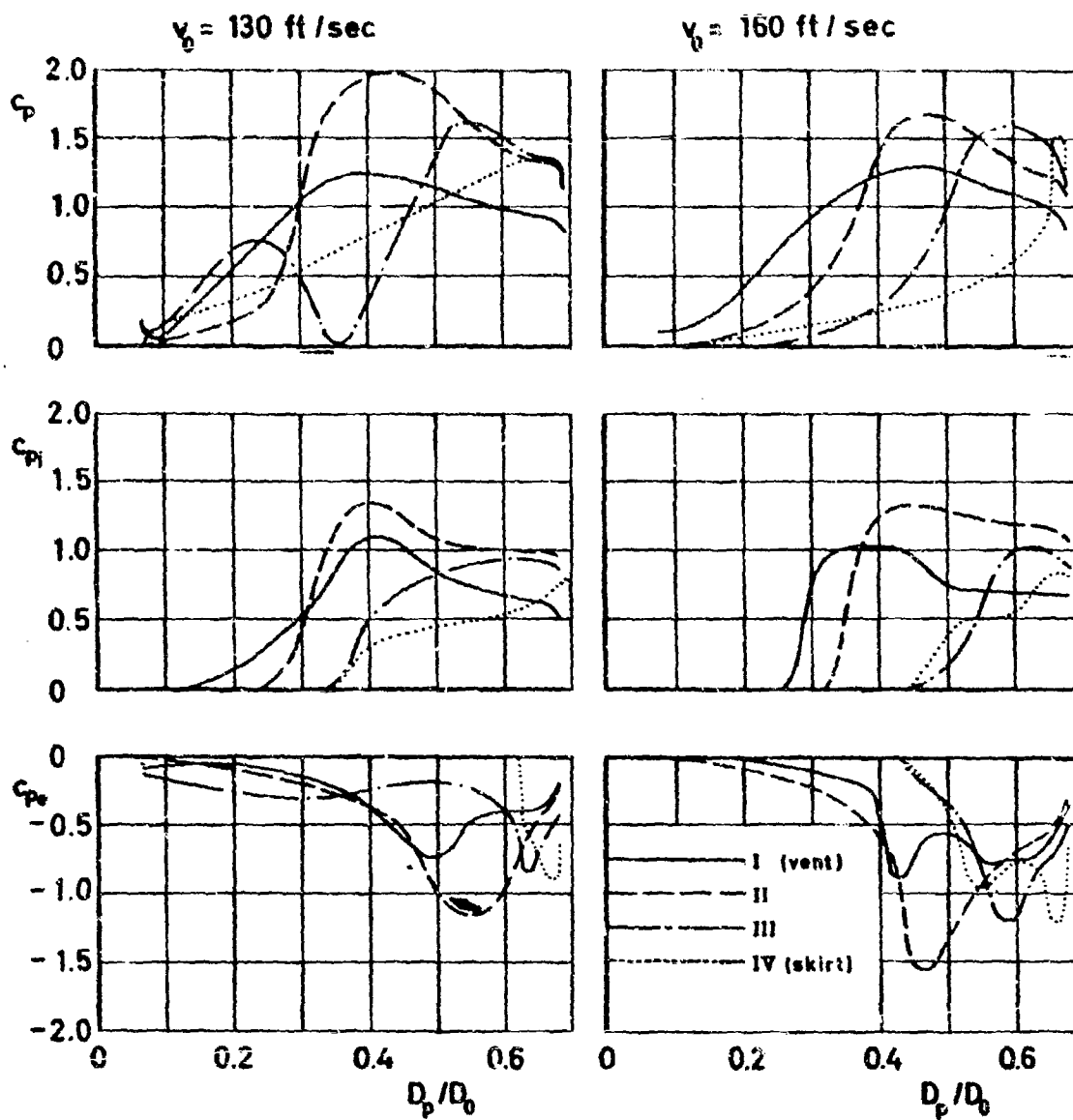
Figure 60 c_p versus D_p/D_0 for Ringslot
