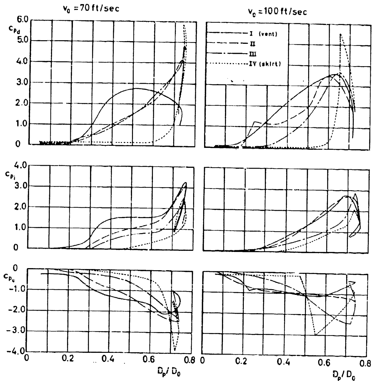
Figure 55 c_p versus D_p/D_0 for Extended Skirt
