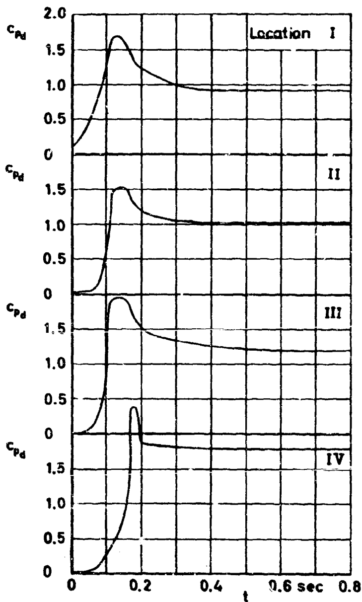
Figure 35 c_{pd} and filling versus time
