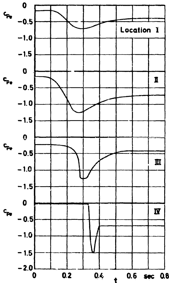
Figure 31 c_{pe} and filling versus time
