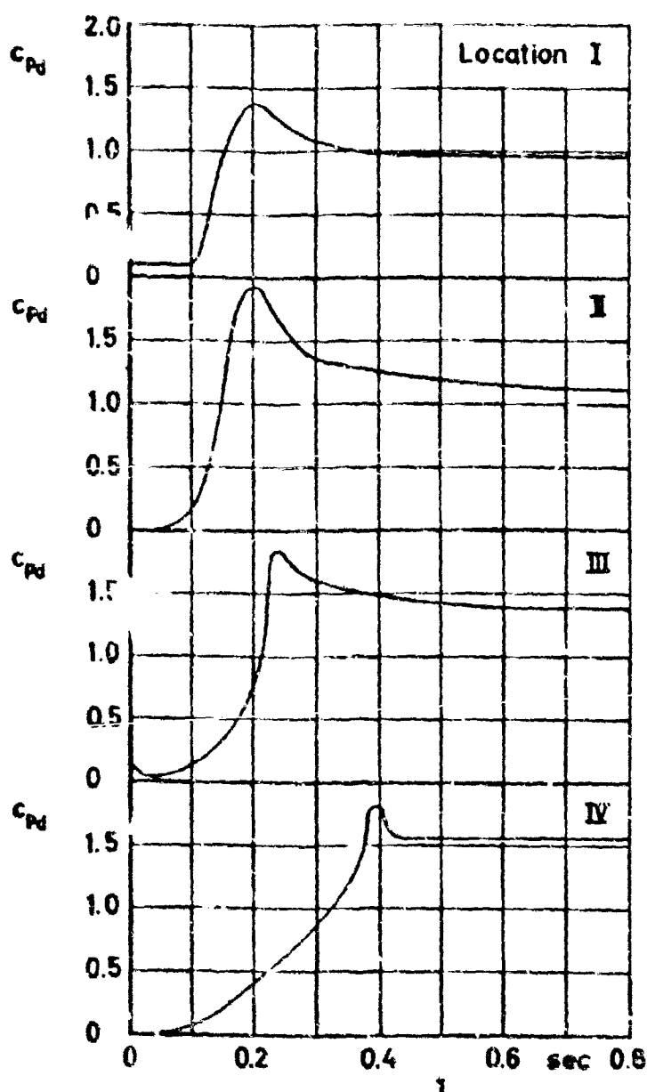
Figure 44 c_{pd} and filling versus time
