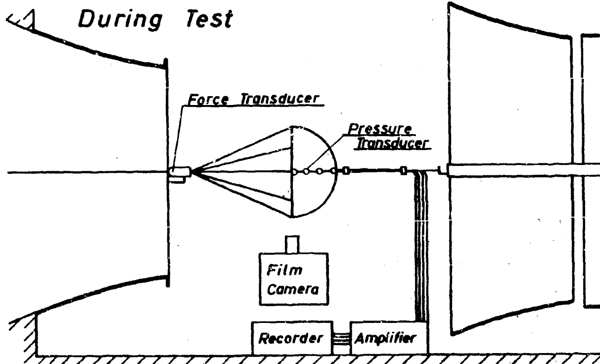
Figure1 Test Arrangement in the Windtunnel
