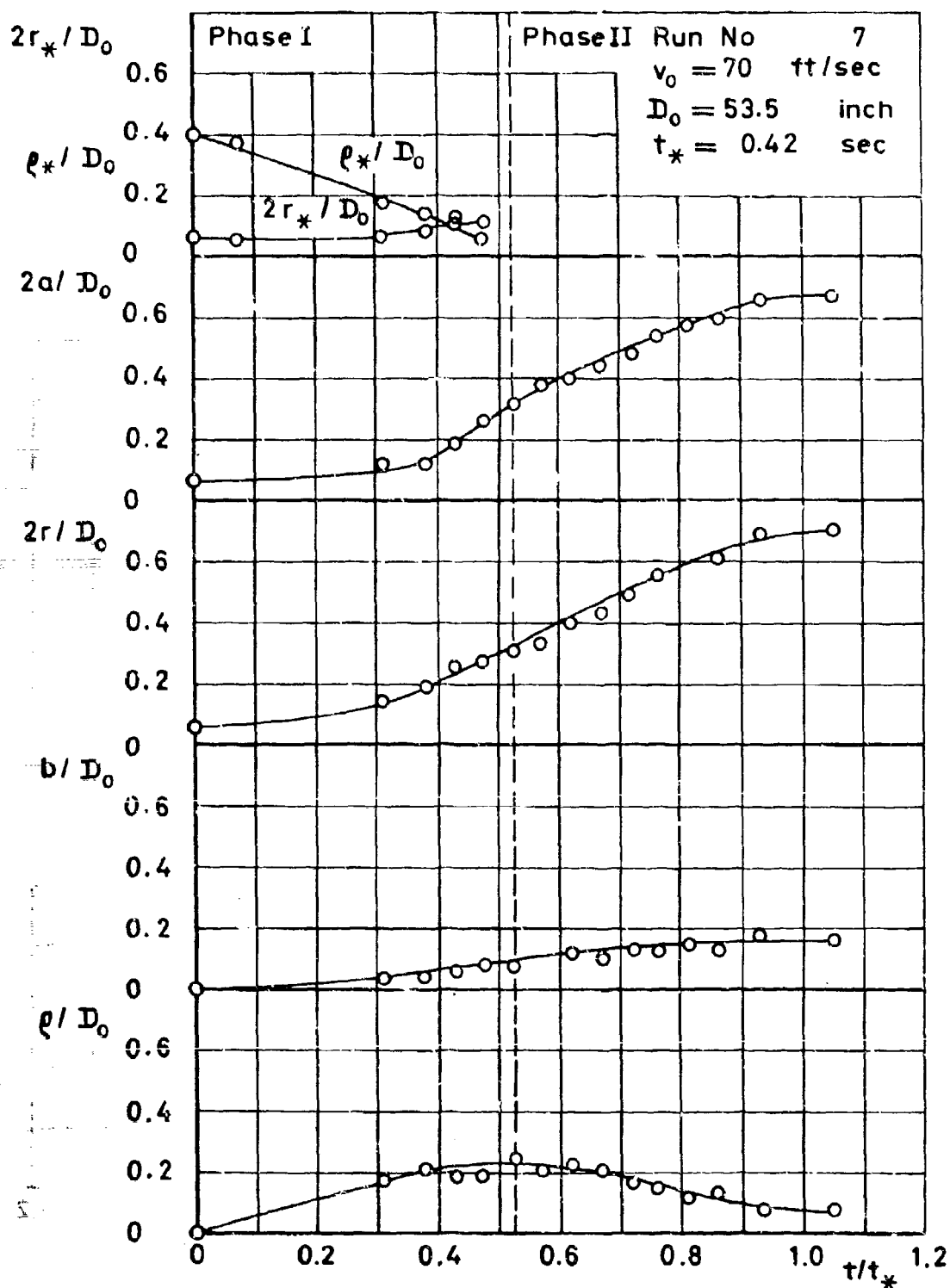
Figure 76 Parameters of Idealized Photographic Shape Versus Time for Ringslot
