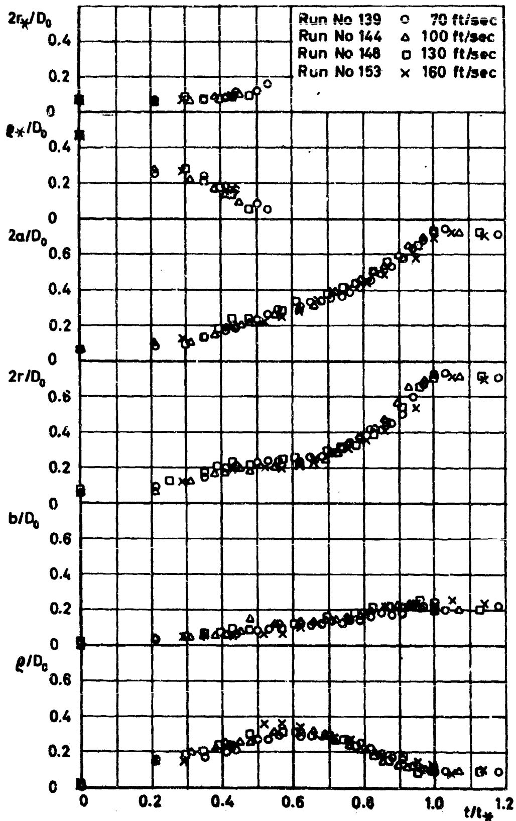
Figure 81 Parameters of Idealized Photographic Shape Versus Time for Extended Skirt
