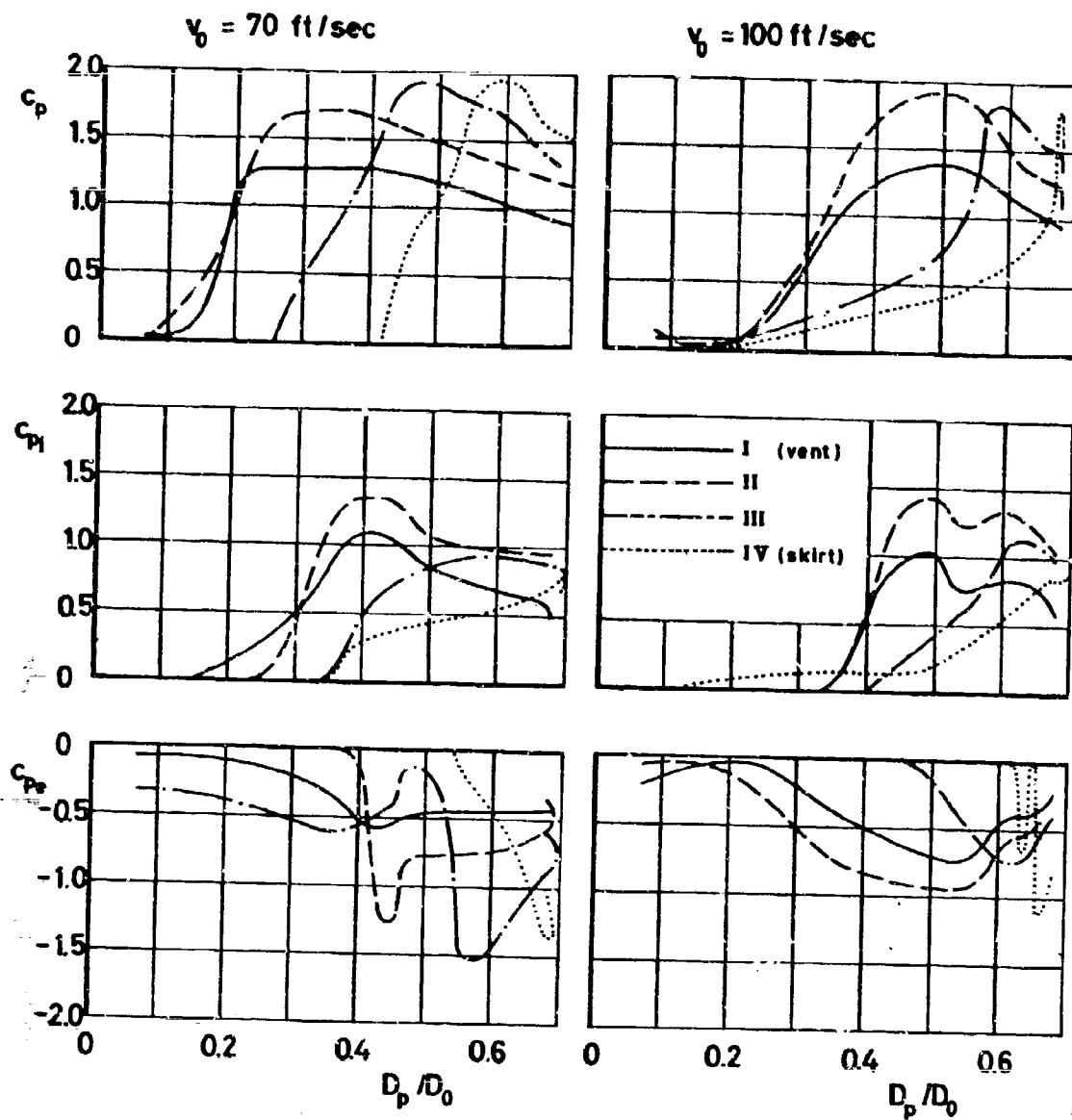
Figure 59 c_p versus D_p/D_0 for Ringslot
