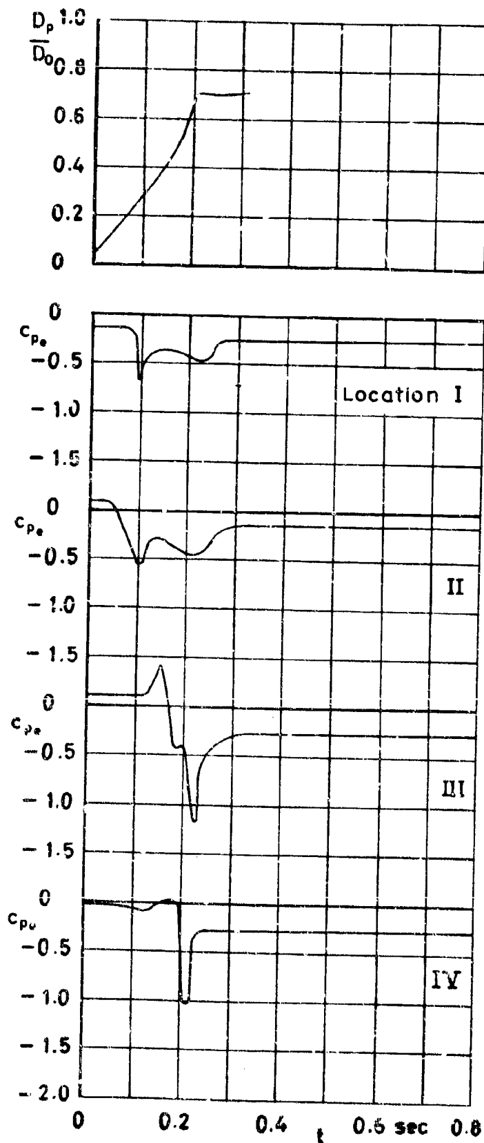
Figure 25 C_p and filling versus time v_0 = 130 ft/sec Run No 231
