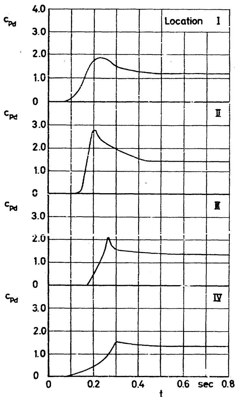
Figure 104 c_{pd} and filling versus time
