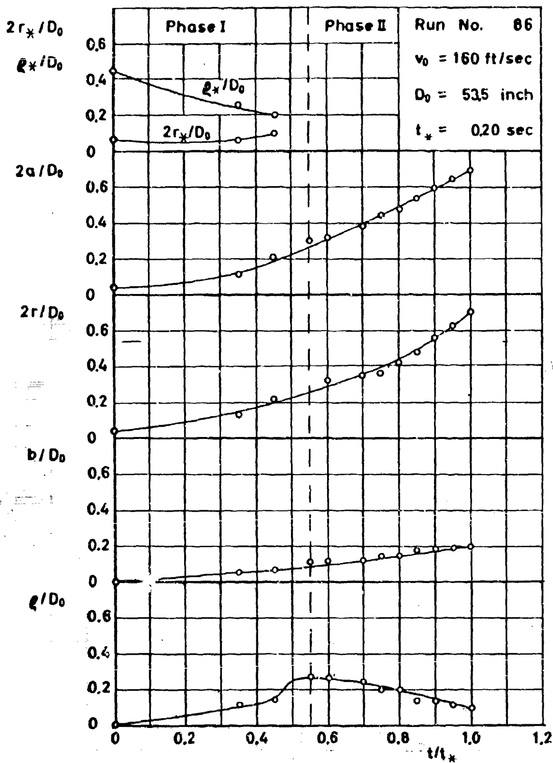
Figure 75 Parameters of Idealized Photographic Shape Versus Time for FIST
