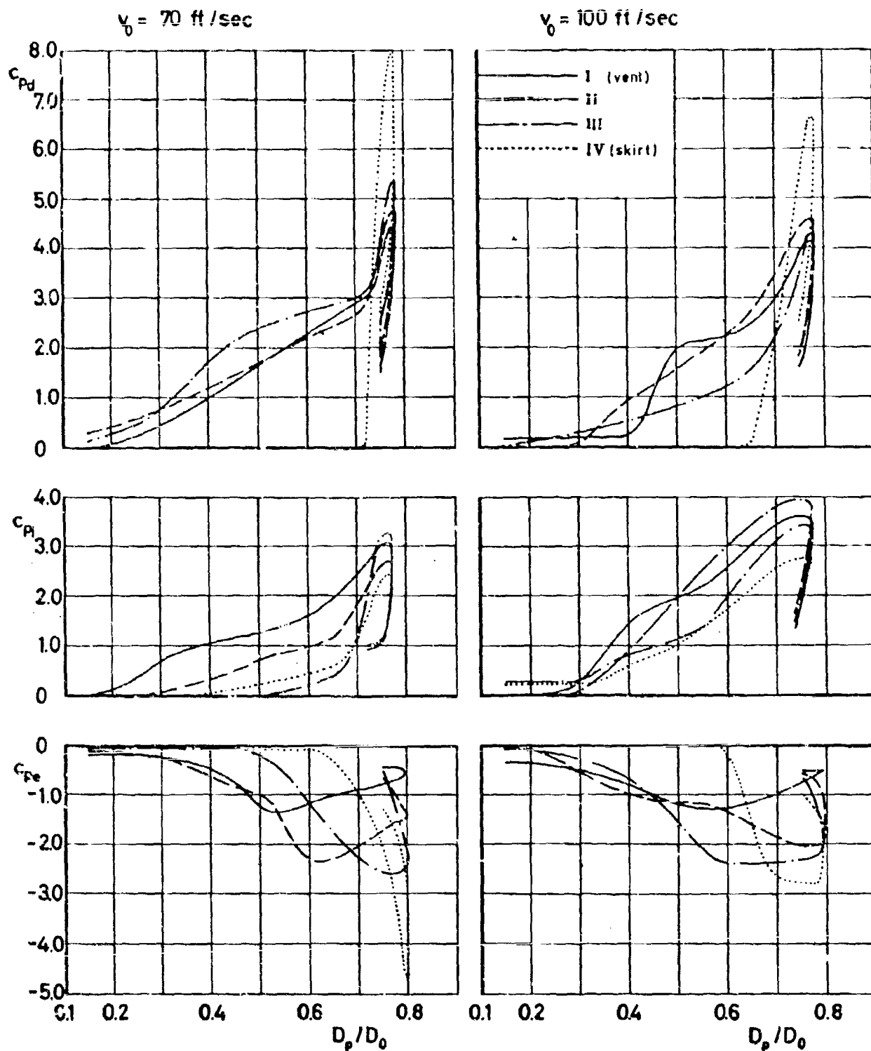
Figure 53 c_p versus D_p/D_0 for Circular Flat
