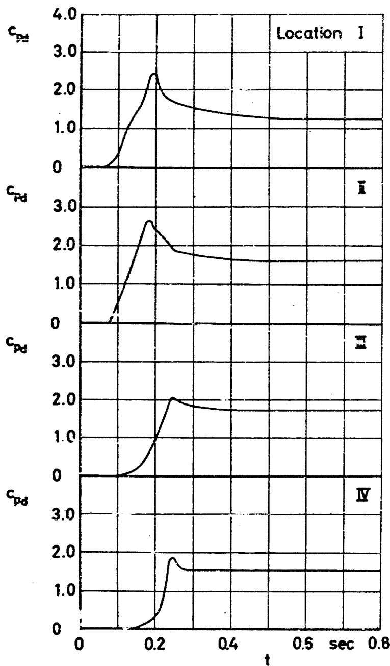
Figure 103 c_{pd} and filling versus time
