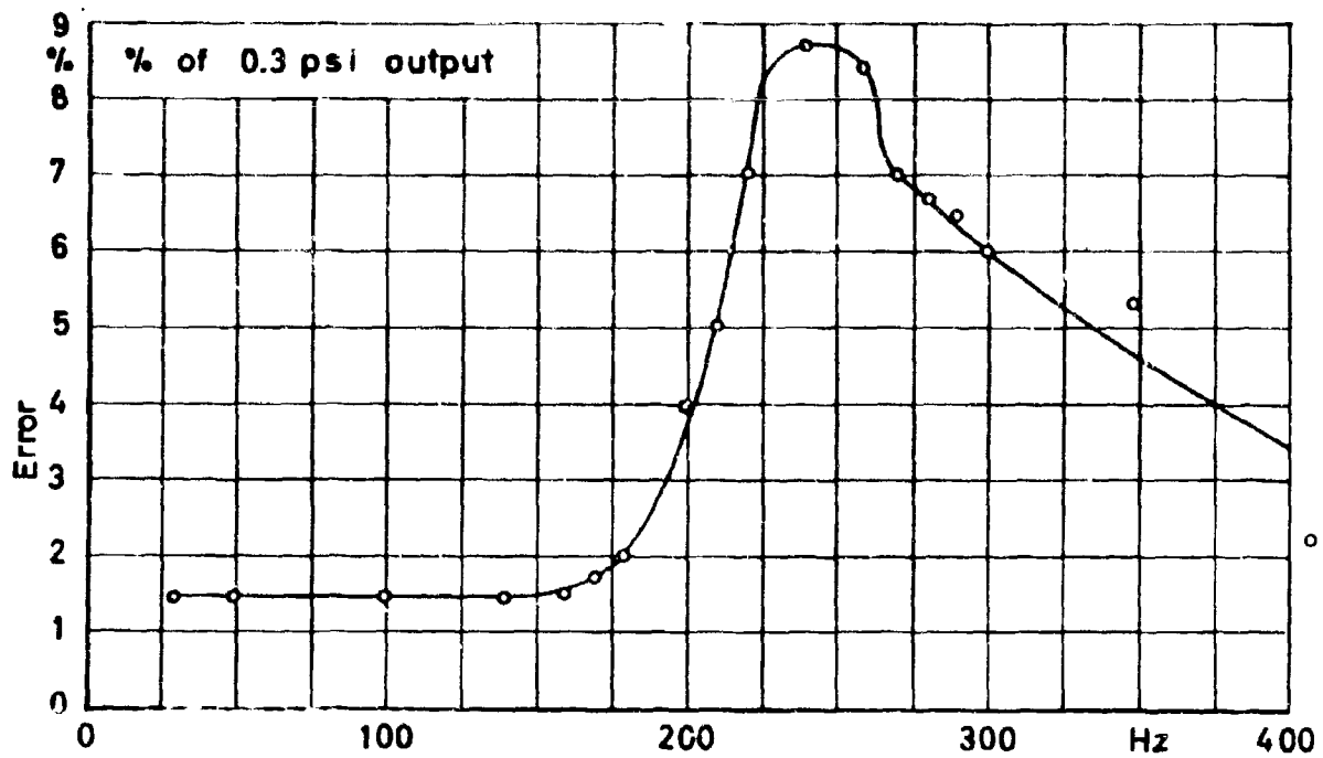
Figure 4 Frequency Response of Pressure Transducer
