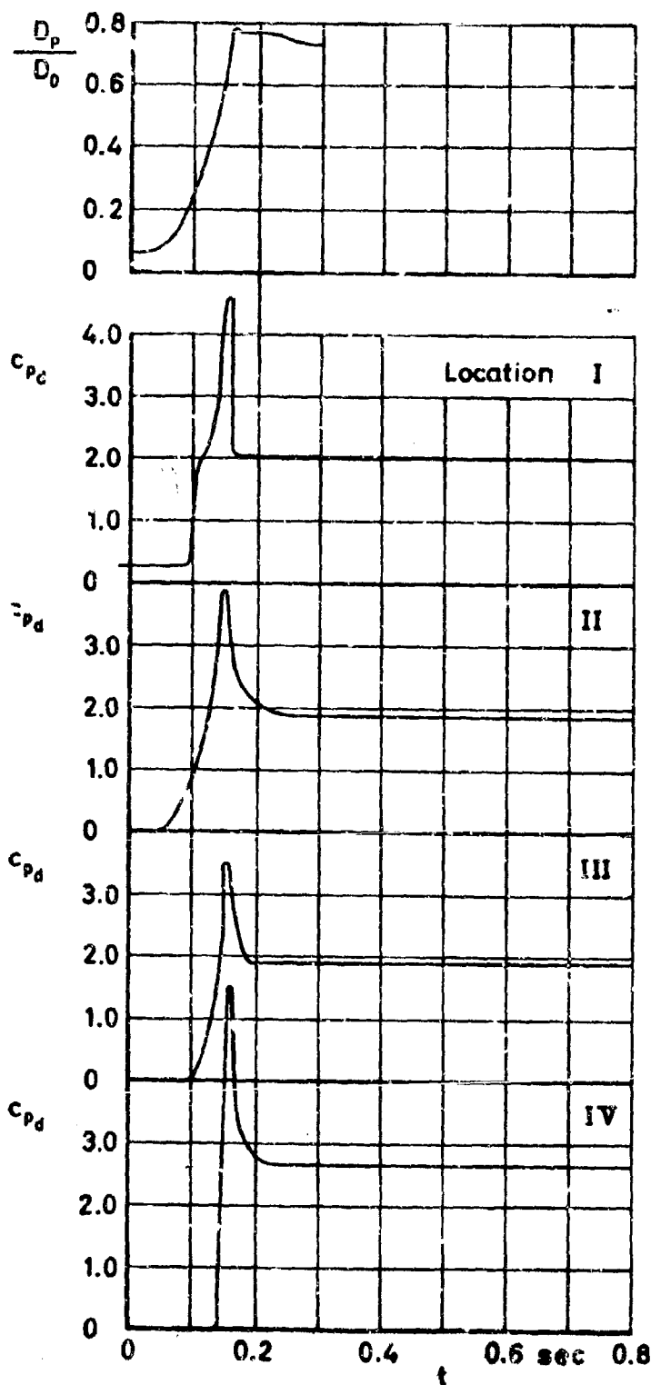
Figure 13 c_{pD} and filling versus time
