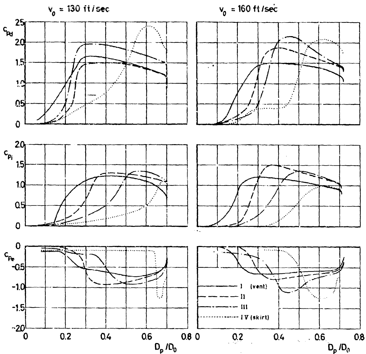
Figure 58 c_p versus D_p/D_0 for FIST
